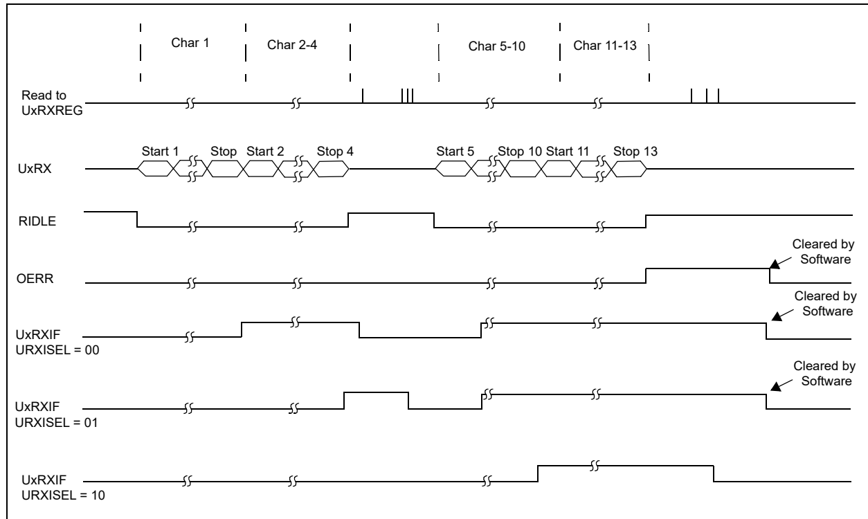
FIGURE 24-2: UART RECEPTION
