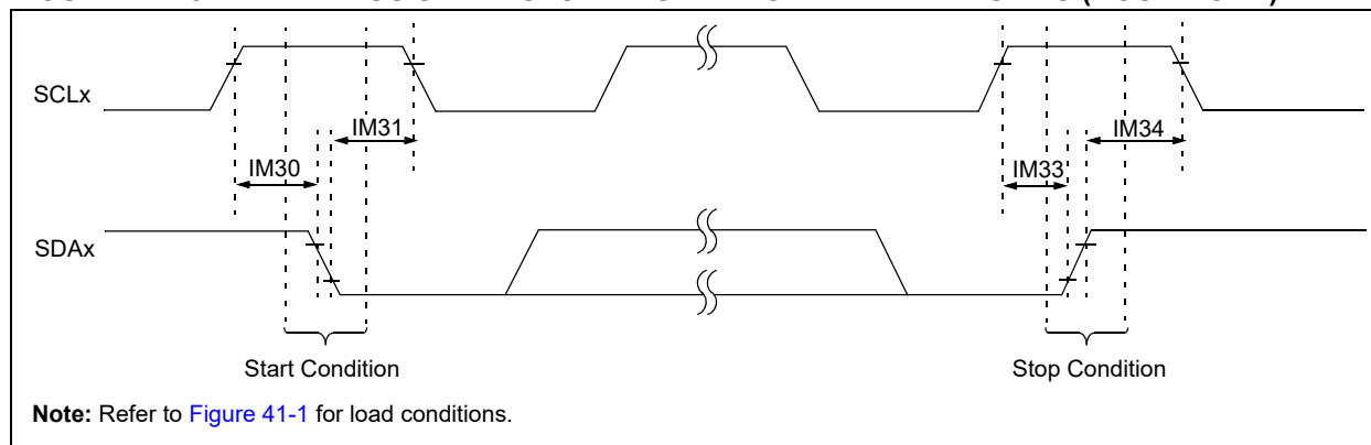
FIGURE 41-15: I2Cx BUS START/STOP BITS TIMING CHARACTERISTICS (HOST MODE)
