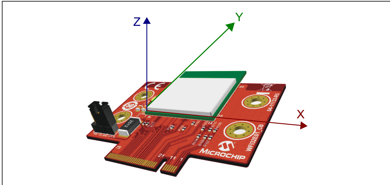
FIGURE 3-12: MODULE ORIENTATION FOR RADIATION PATTERN MEASUREMENT
