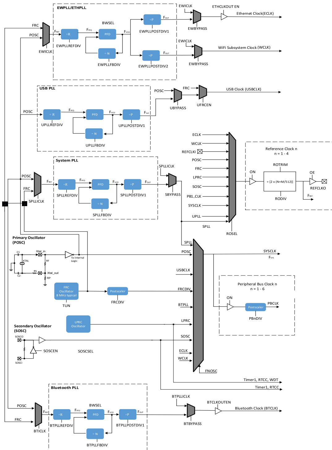
FIGURE 11-1: PIC32MZ1025W104 FAMILY OSCILLATOR DIAGRAM
