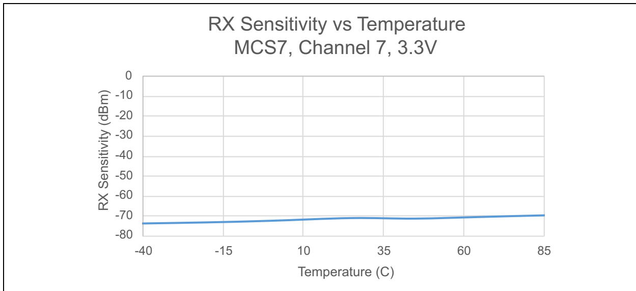
FIGURE 41-33: RECEIVE SENSITIVITY VS TEMPERATURE
