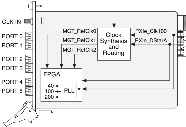
Figure 6-2. PXIe-7902 Clocking Diagram
