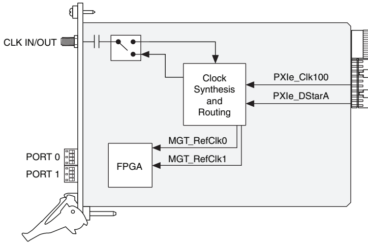
Figure 2-2. PXIe-6591R Clocking Diagram
