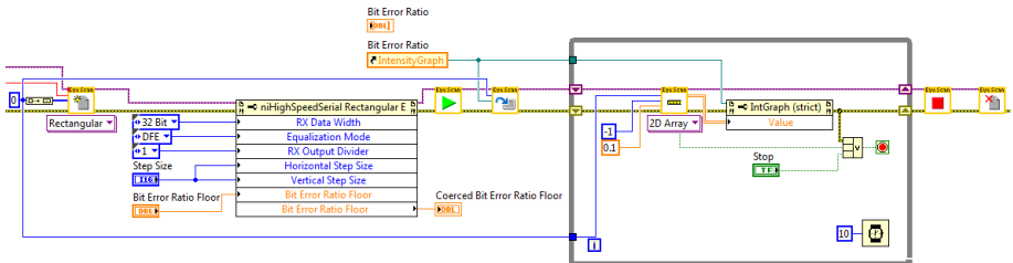
Figure 8-10. Rectangular Eye Scan
