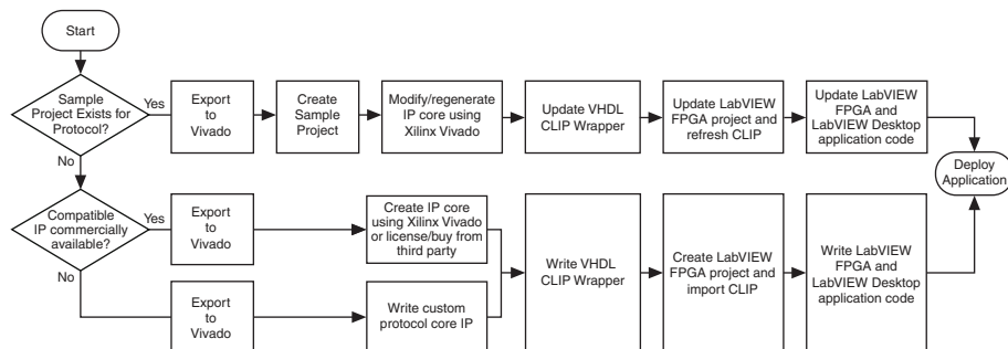
Figure 8-1. High-Speed Serial Development Process
