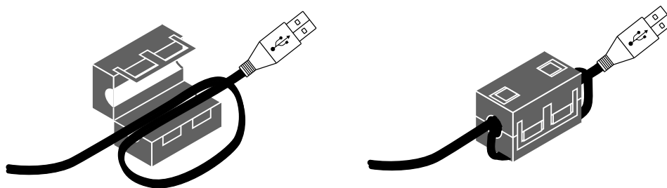
Figure 9. Installing a Ferrite on a Single USB 2.0 Cable
