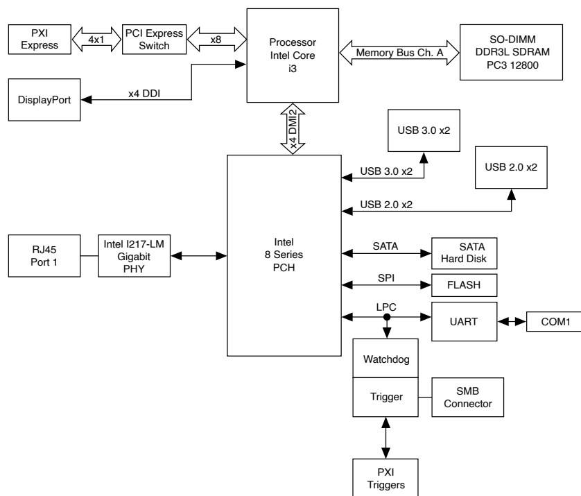
Figure 1. PXle-8821 Block Diagram
