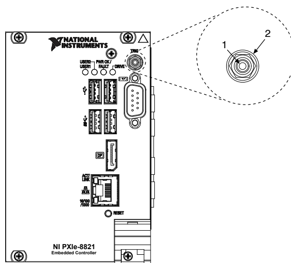
Figure 10. TRIG Connector Location and Pinout
