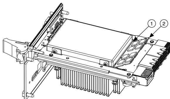
Figure 3. Installing a DDR3L SO-DIMM in a PXle-8821 Controller
