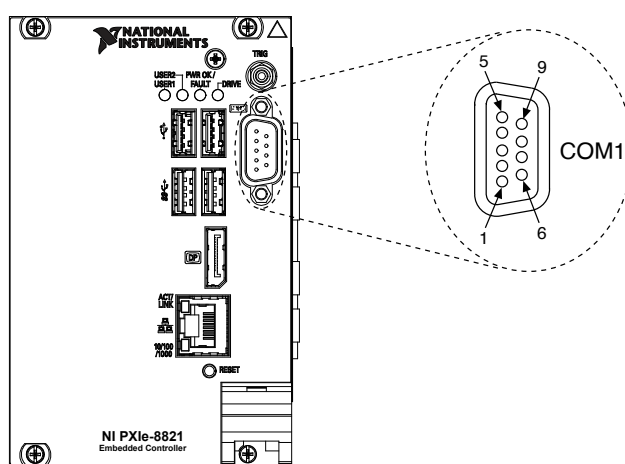
Figure 6. COM1 Connector Location and Pinout
