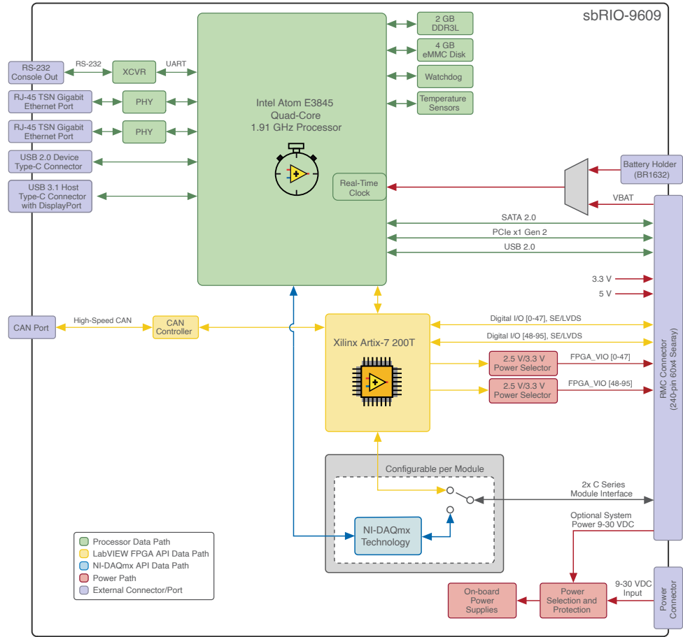
Figure 1. sbRIO-9609 Block Diagram
