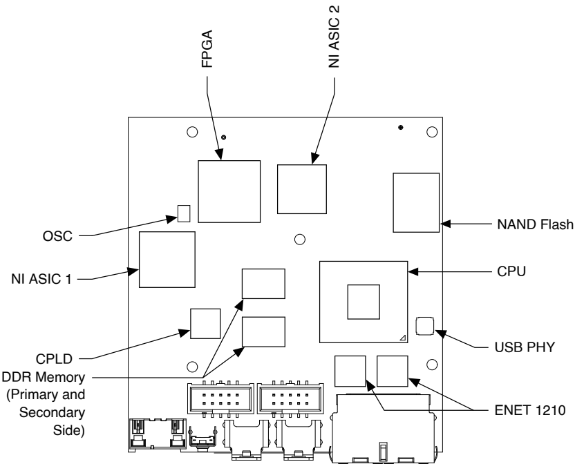
Figure 2. sbRIO-9609 Component Locations
