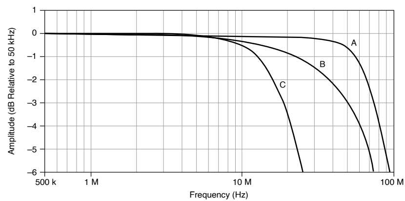
Figure 1. Frequency Response, Measured
