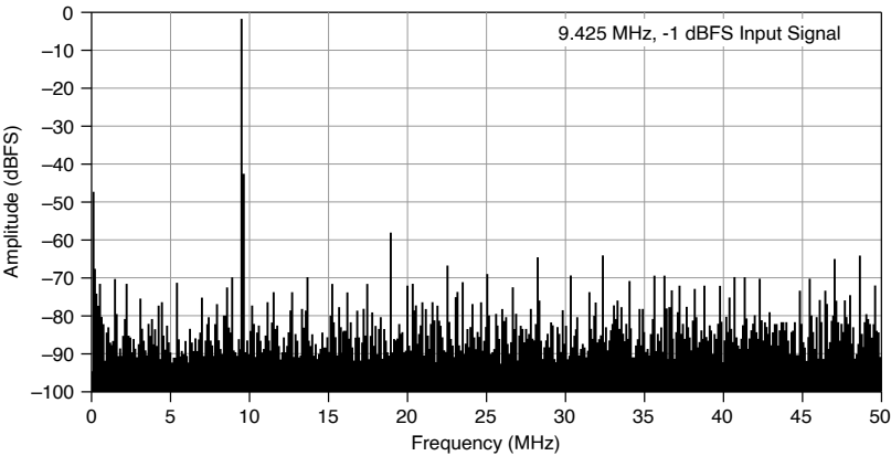
Figure 2. USB-5132 Dynamic Performance, 1 V pk-pk Range, 524,288-Point FFT, Measured
