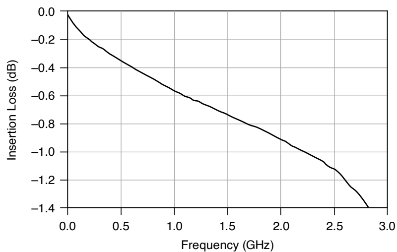
Figure 1. Insertion Loss, Typical
