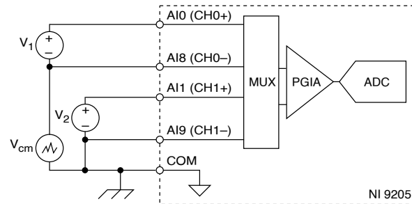
Figure 2. Connecting Grounded Differential Signals to the NI 9205
