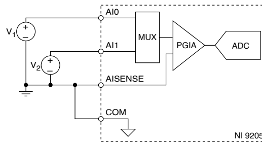
Figure 5. Connecting an RSE Voltage Signal to the NI 9205
