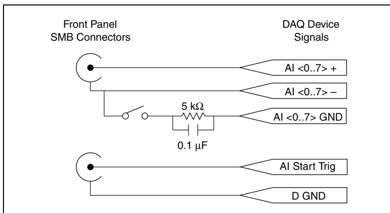
Figure 4. NI TB-2709 Block Diagram
