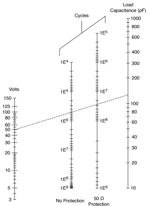
Figure 1. Reed Relay Lifetime Nomograph
