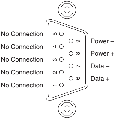
Figure 2-3. Fieldbus Connector Pinout
