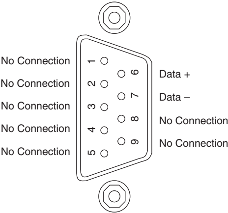
Figure 2-7. Pinout for 9-Pin D-SUB Female Connector of the DB-9 Cable
