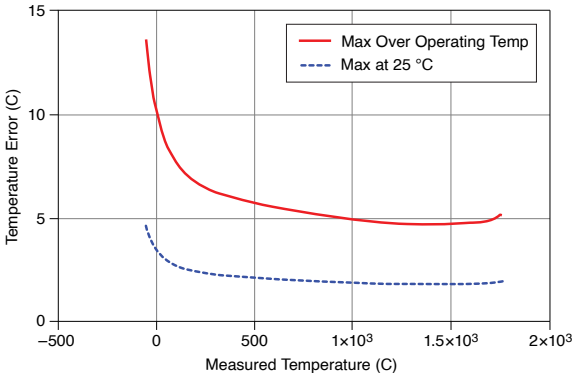
Figure 4. Temperature Error of Type S Thermocouple
