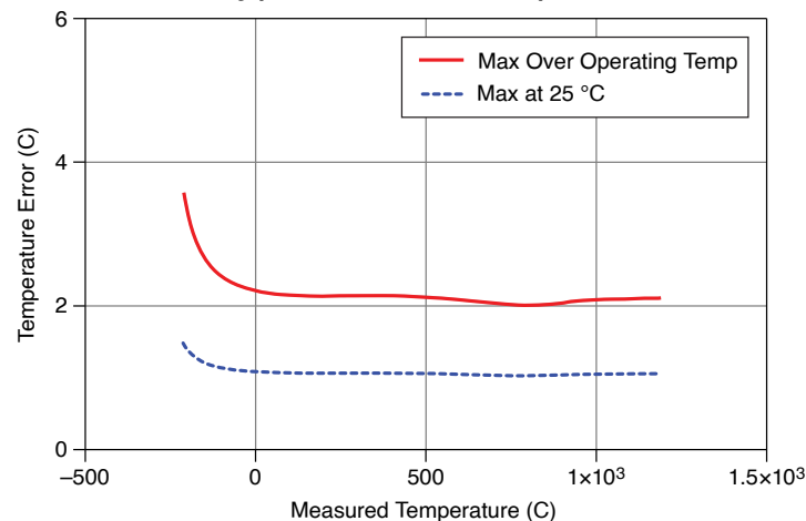
Figure 1. Temperature Error of Type J Thermocouple
