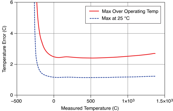
Figure 3. Temperature Error of Type R Thermocouple
