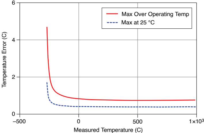
Figure 8. Temperature Error of Type E Thermocouple
