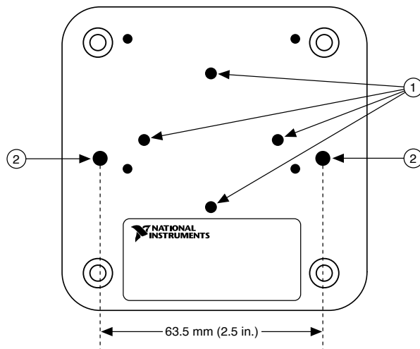
Figure 4. SCB-19 Mounting Screw Holes
