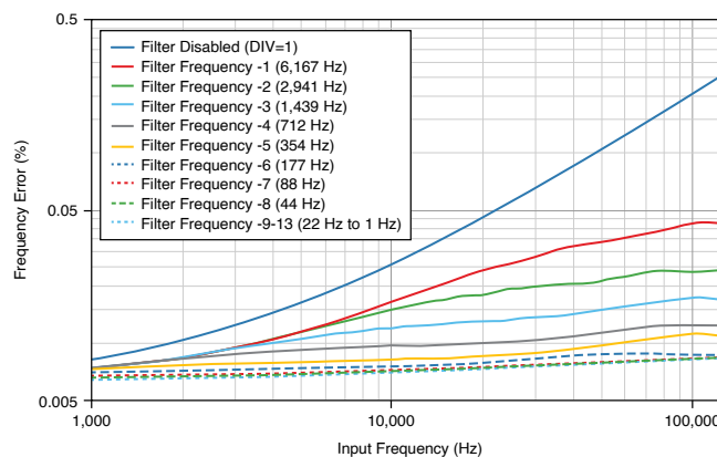
Figure 17. Maximum Frequency Accuracy across Frequencies
