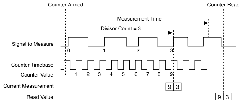
Figure 12. Divisor completes before Measurement Time
