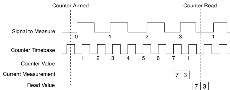
Figure 10. Measurement with Divisor set to 3
