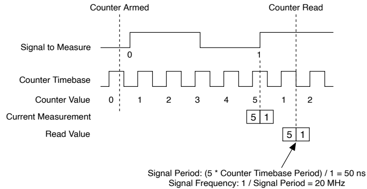
Figure 9. Measurement with Divisor set to 1
