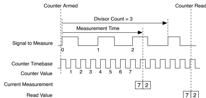
Figure 13. Measurement Time completes before Divisor
