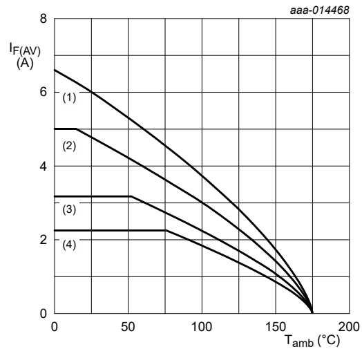
Fig. 8. Average forward current as a function of ambient temperature; typical values FR4 PCB, standard footprint T_j = 175 \text{ }^\circ\text{C} (1) \delta = 1 ; DC (2) \delta = 0.5 ; f = 20 \text{ kHz} (3) \delta = 0.2 ; f = 20 \text{ kHz} (4) \delta = 0.1 ; f = 20 \text{ kHz}
