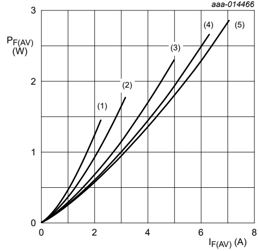
Fig. 6. Average forward power dissipation as a function of average forward current; typical values T_j = 100 \text{ }^\circ\text{C} (1) \delta = 0.1 (2) \delta = 0.2 (3) \delta = 0.5 (4) \delta = 0.8 (5) \delta = 1
