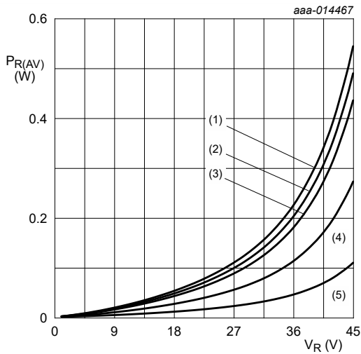
Fig. 7. Average reverse power dissipation as a function of reverse voltage; typical values T_j = 100 \text{ }^\circ\text{C} (1) \delta = 1 (2) \delta = 0.9 (3) \delta = 0.8 (4) \delta = 0.5 (5) \delta = 0.2
