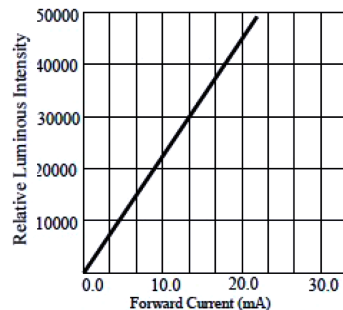
FORWARD CURRENT VS. LUMINOUS INTENSITY
