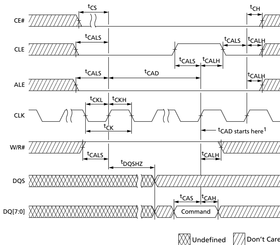
Figure 22: Synchronous Command Cycle
