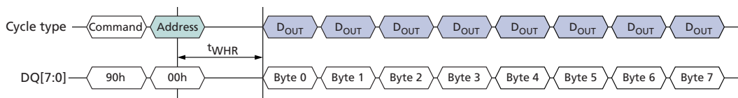
Figure 31: READ ID (90h) with 00h Address Operation
