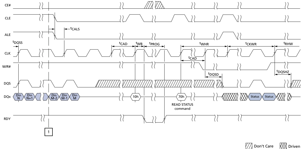
Figure 104: PROGRAM PAGE Operation (2 of 2)
