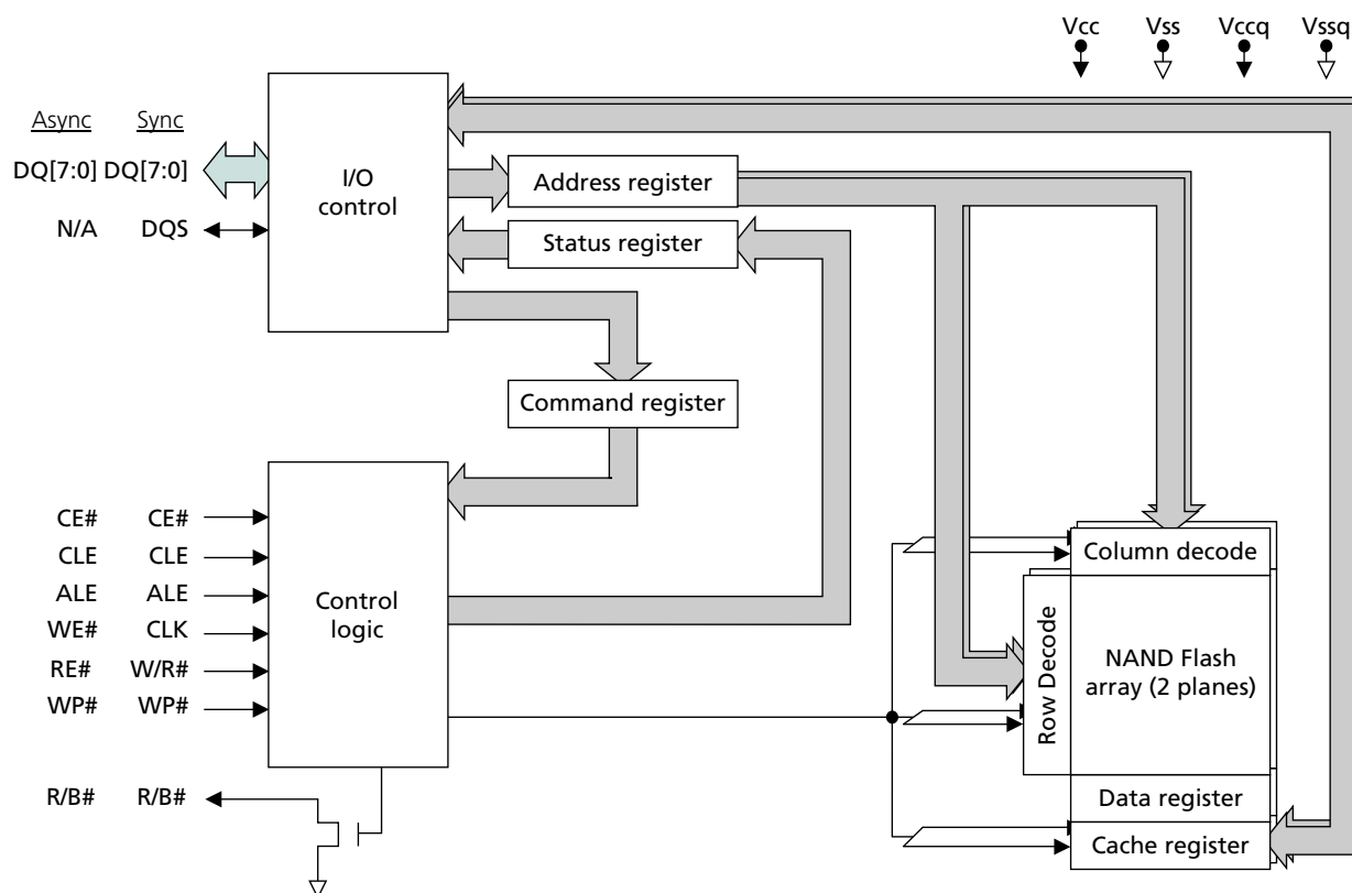
Figure 6: NAND Flash Die (LUN) Functional Block Diagram
