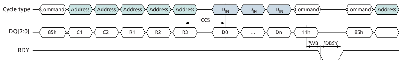
Figure 63: COPYBACK PROGRAM MULTI-PLANE (85h-11h) Operation
