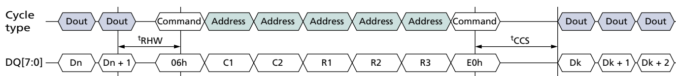
Figure 42: CHANGE READ COLUMN ENHANCED (06h-E0h) Operation
