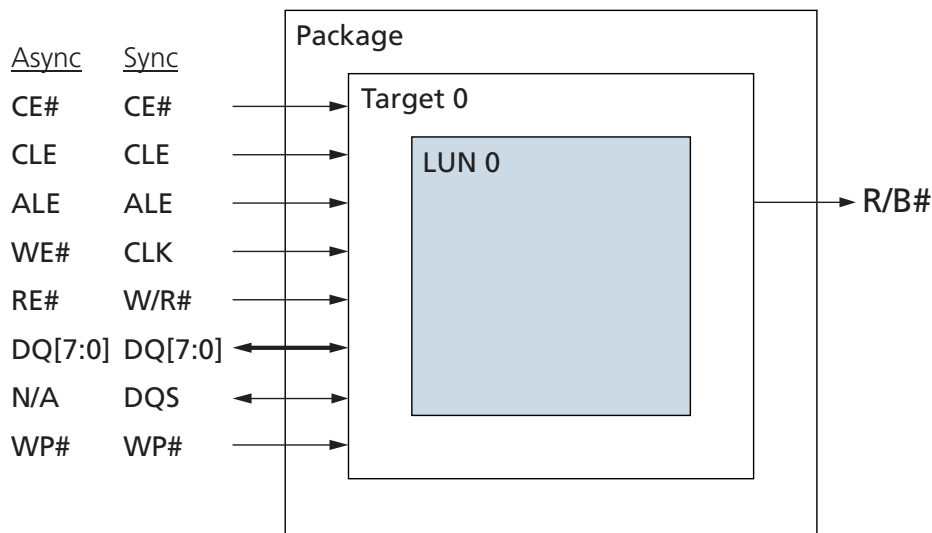
Figure 7: Device Organization for Single-Die Package (TSOP, BGA)
