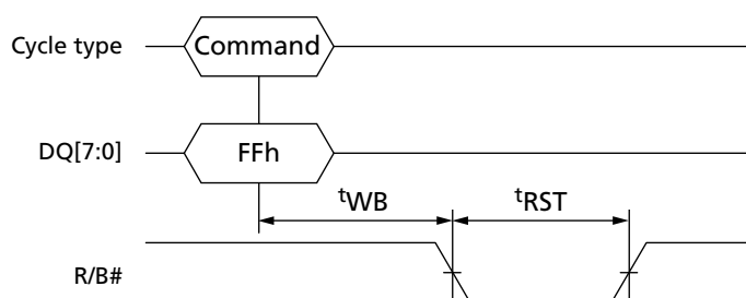
Figure 28: RESET (FFh) Operation
