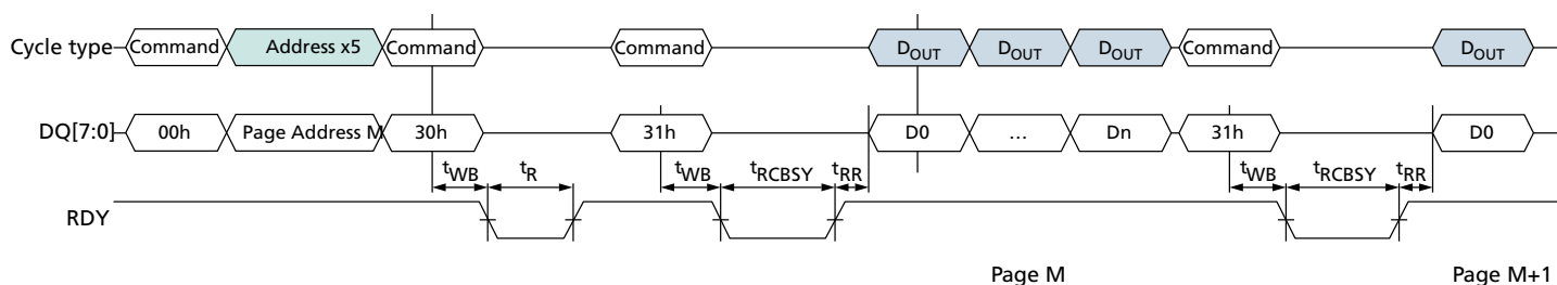
Figure 47: READ PAGE CACHE SEQUENTIAL (31h) Operation
