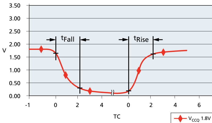
Figure 17: t_{\text{Fall}} and t_{\text{Rise}} ( V_{\text{CCQ}} = 1.7\text{-}1.95\text{V} )
