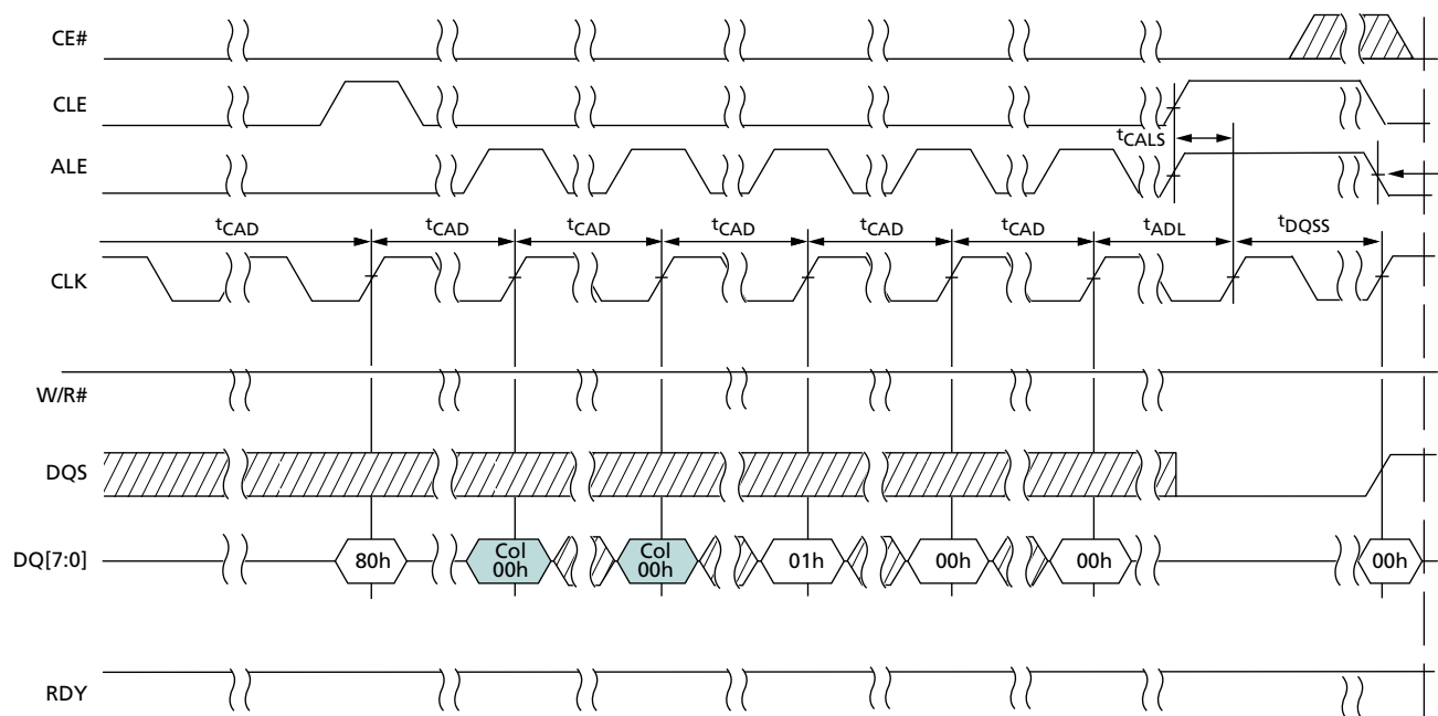
Figure 114: PROTECT OTP AREA
