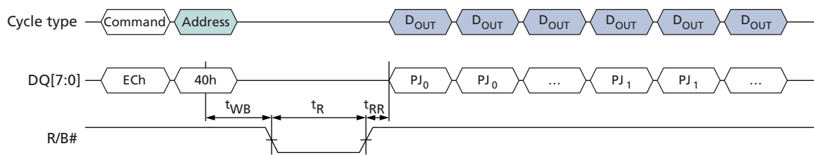
Figure 35: READ PARAMETER (ECh) with 40h Address Operation for JEDEC
