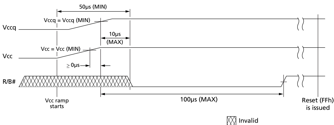
Figure 26: R/B# Power-On Behavior
