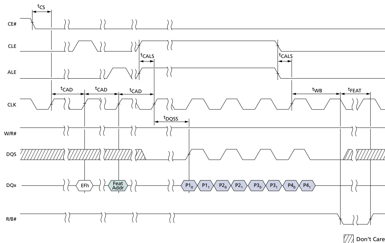
Figure 88: SET FEATURES Operation
