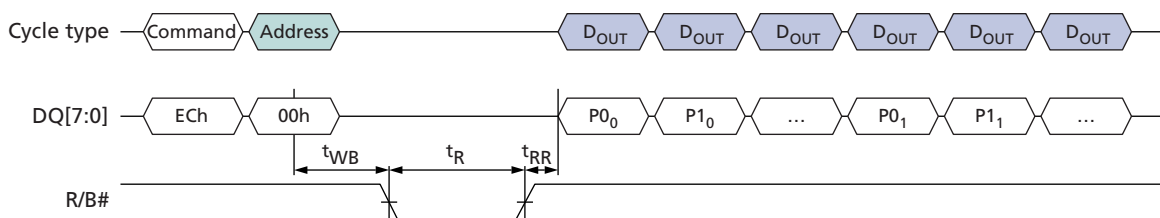
Figure 34: READ PARAMETER (ECh) with 00h Address Operation for ONFI
