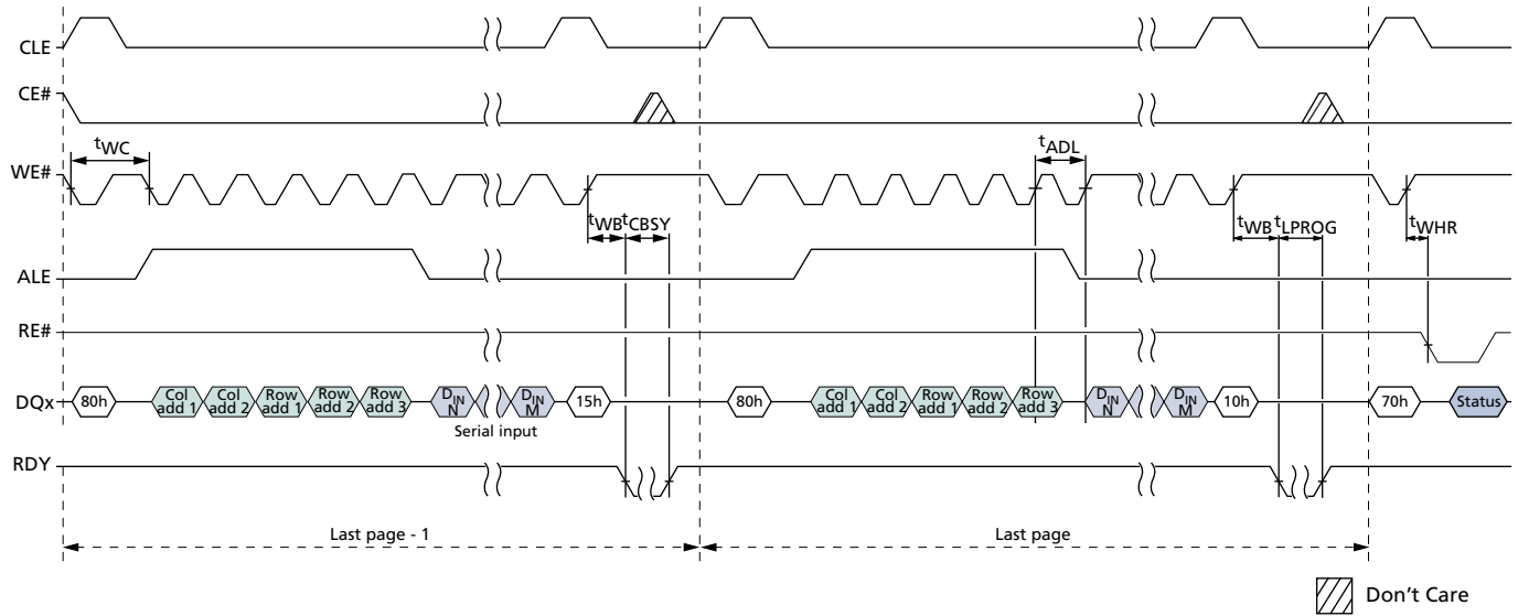
Figure 85: PROGRAM PAGE CACHE Ending on 15h
