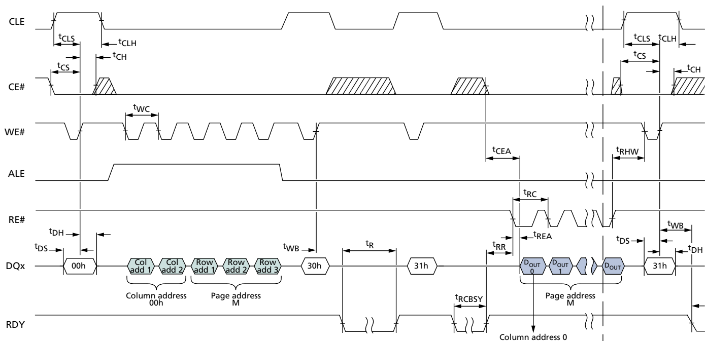
Figure 78: READ PAGE CACHE SEQUENTIAL
