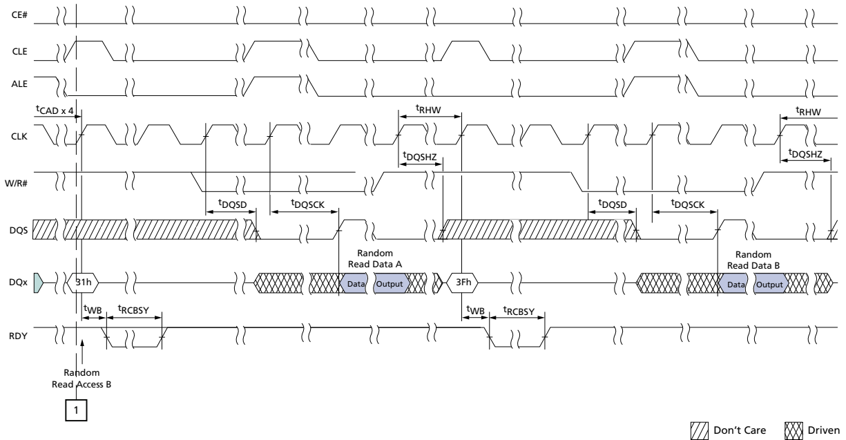
Figure 100: READ PAGE CACHE RANDOM (2 of 2)
