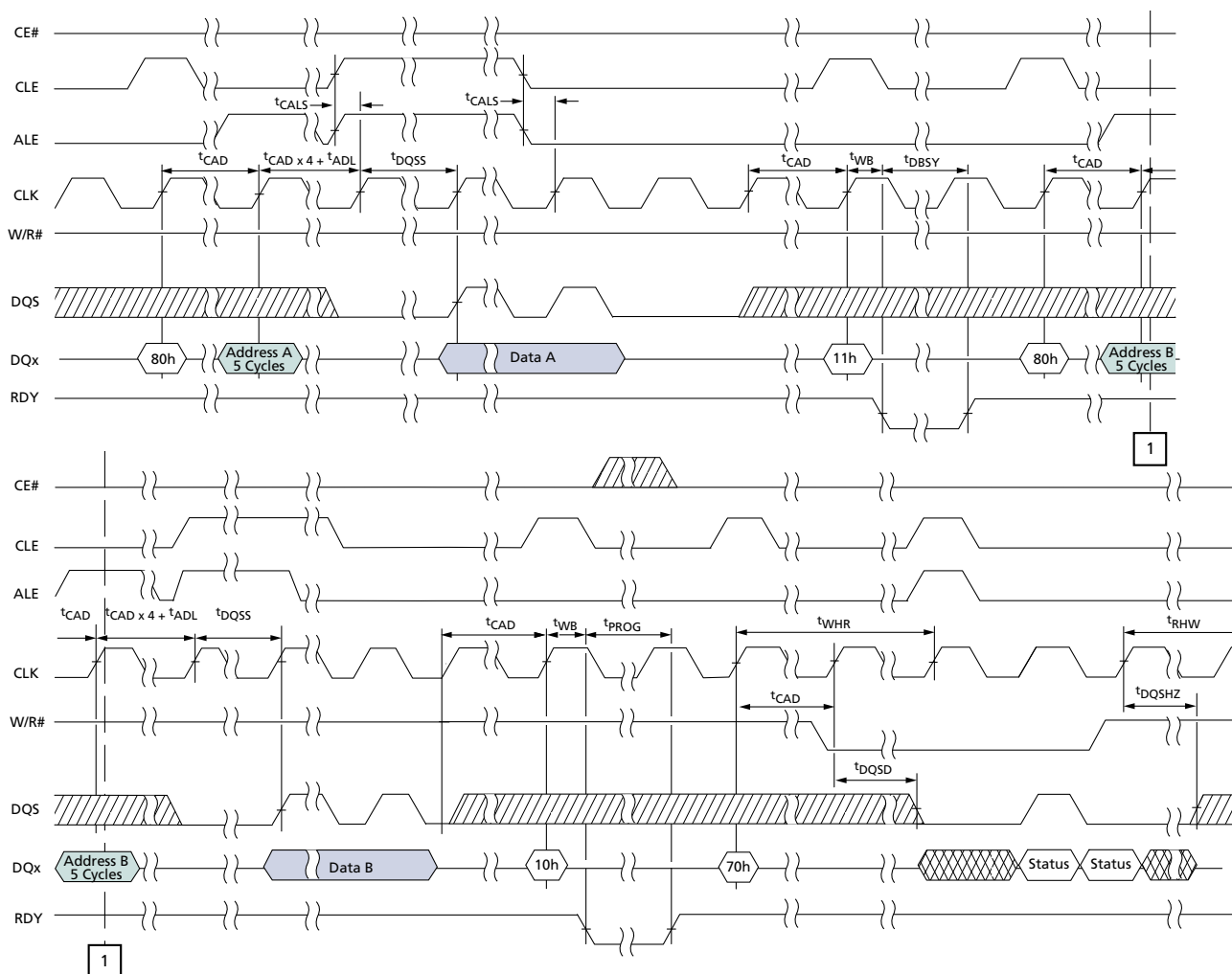
Figure 106: Multi-Plane Program Page
