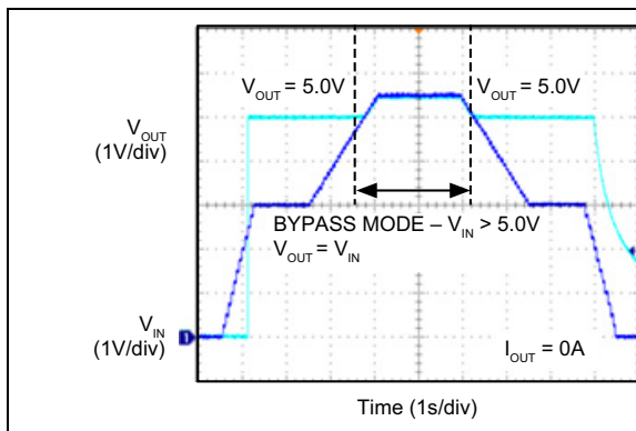
FIGURE 2-20: Bypass Mode.
