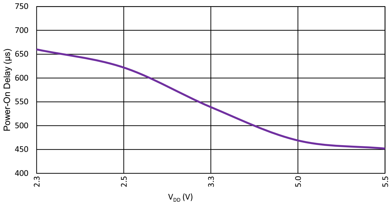
Figure 120. Oscillator0 Maximum Power-On Delay vs. V_{DD} at T = 25\text{ }^\circ\text{C} , \text{OSC0} = 2.048\text{ kHz}
