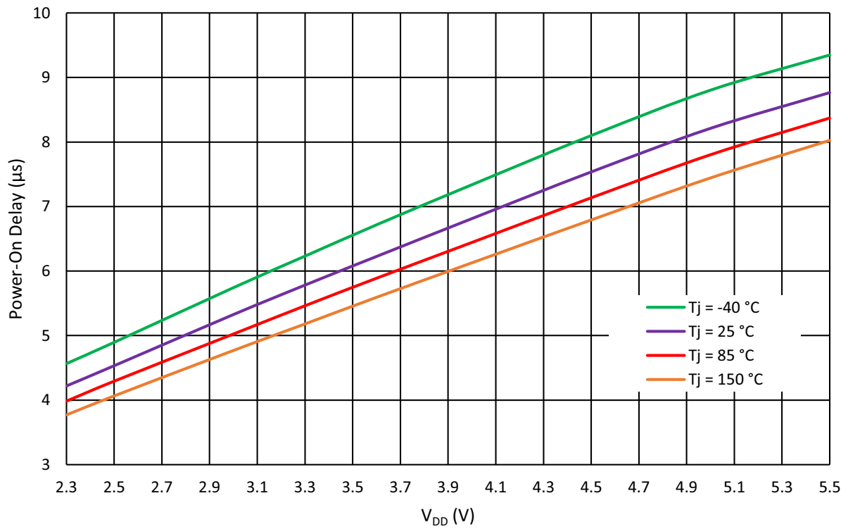
Figure 34. CCMP Power-On Delay vs. V DD (BG is Forced On)
