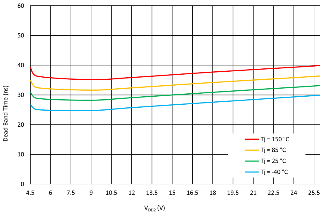
Figure 24. Half Bridge Dead Band Time vs. V DD2 at V DD = 2.3 V to 5.5 V, Rising Signal, f = 50 kHz for Pre-Driver Mode
