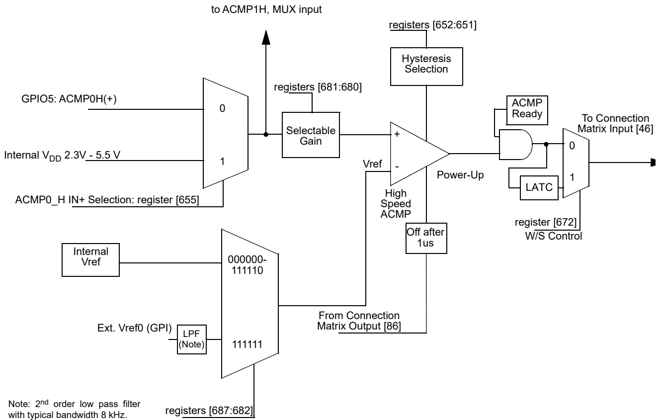
Figure 99. ACMP0H Block Diagram
