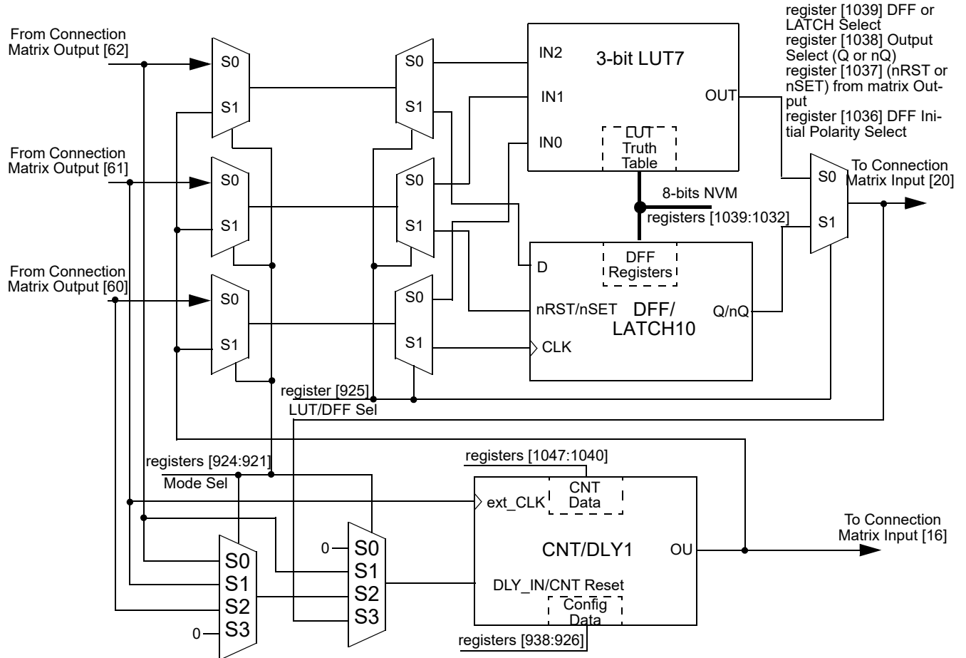
Figure 64. 8-bit Multi-Function Macrocells Block Diagram (3-bit LUT7/DFF10, CNT/DLY1)
