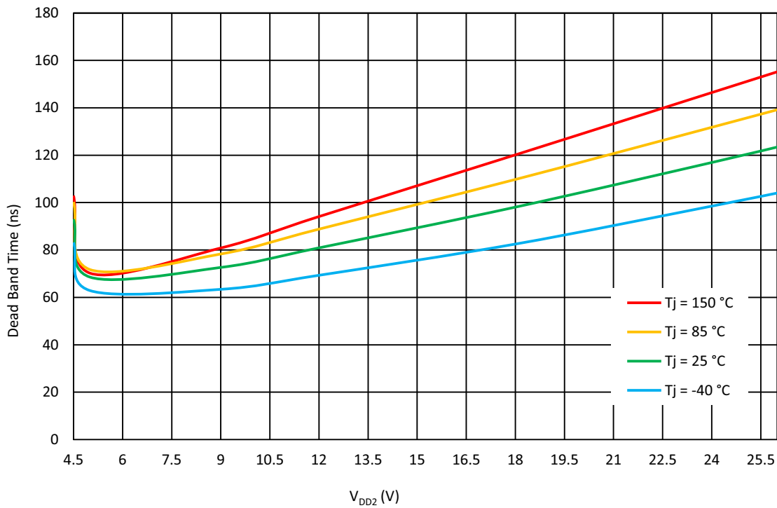
Figure 26. Half Bridge Dead Band Time vs. V DD2 at V DD = 2.3 V to 5.5 V, Rising Signal, f = 50 kHz, for Regular Mode
