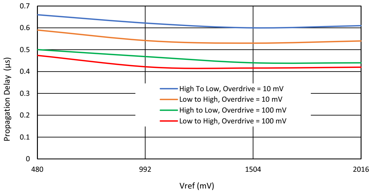
Figure 33. Typical Propagation Delay vs. Vref for CCMP at T = 25 °C, at V DD = 2.3 V to 5.5 V, Gain = 4
