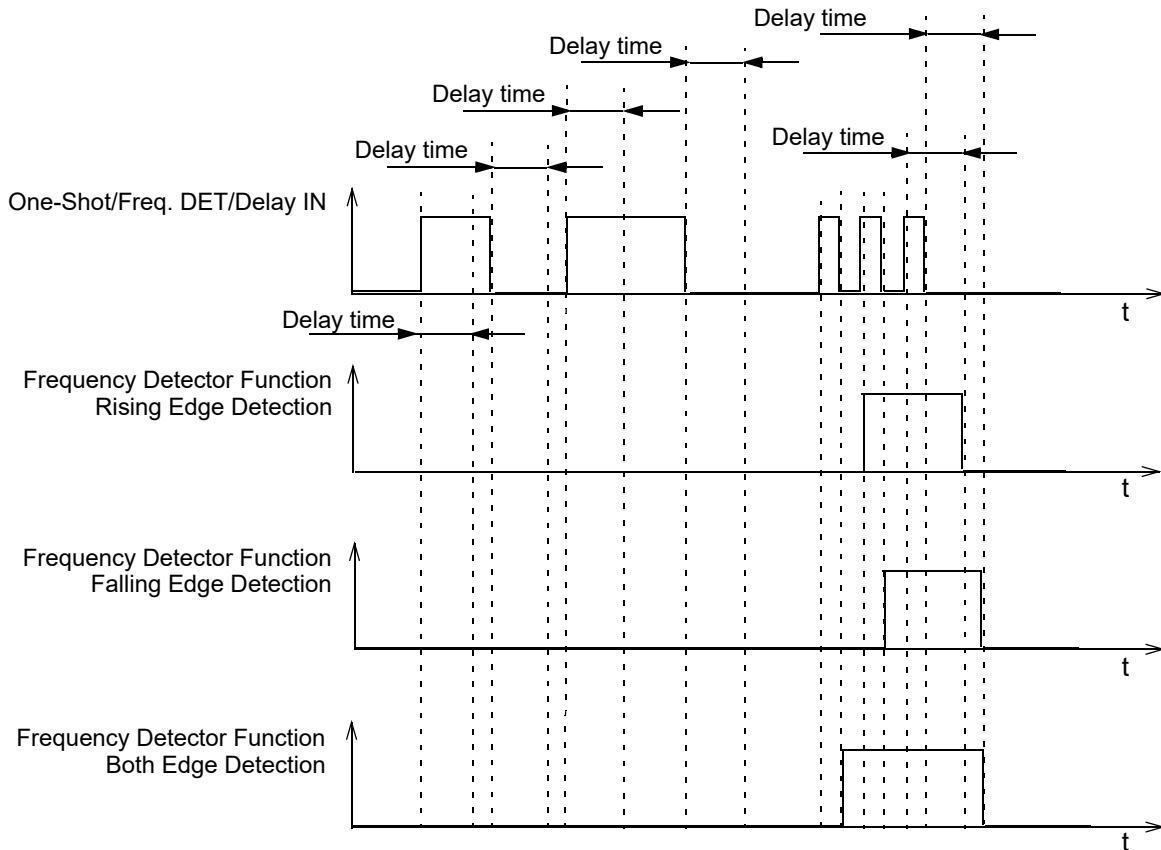
Figure 73. Frequency Detection Mode Timing Diagram
