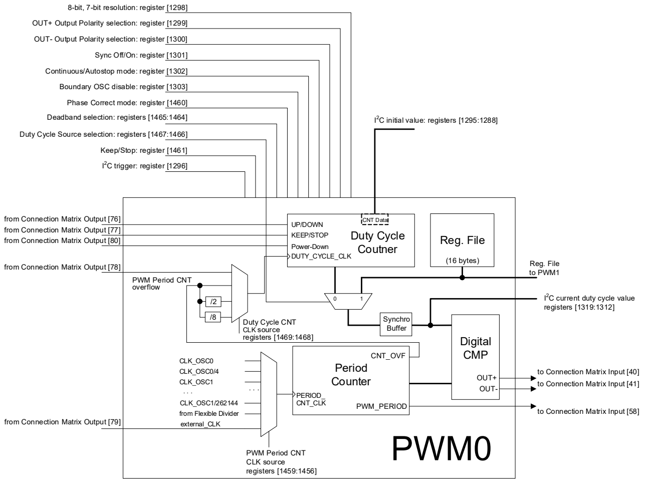
Figure 97. PWM0 Functional Diagram
