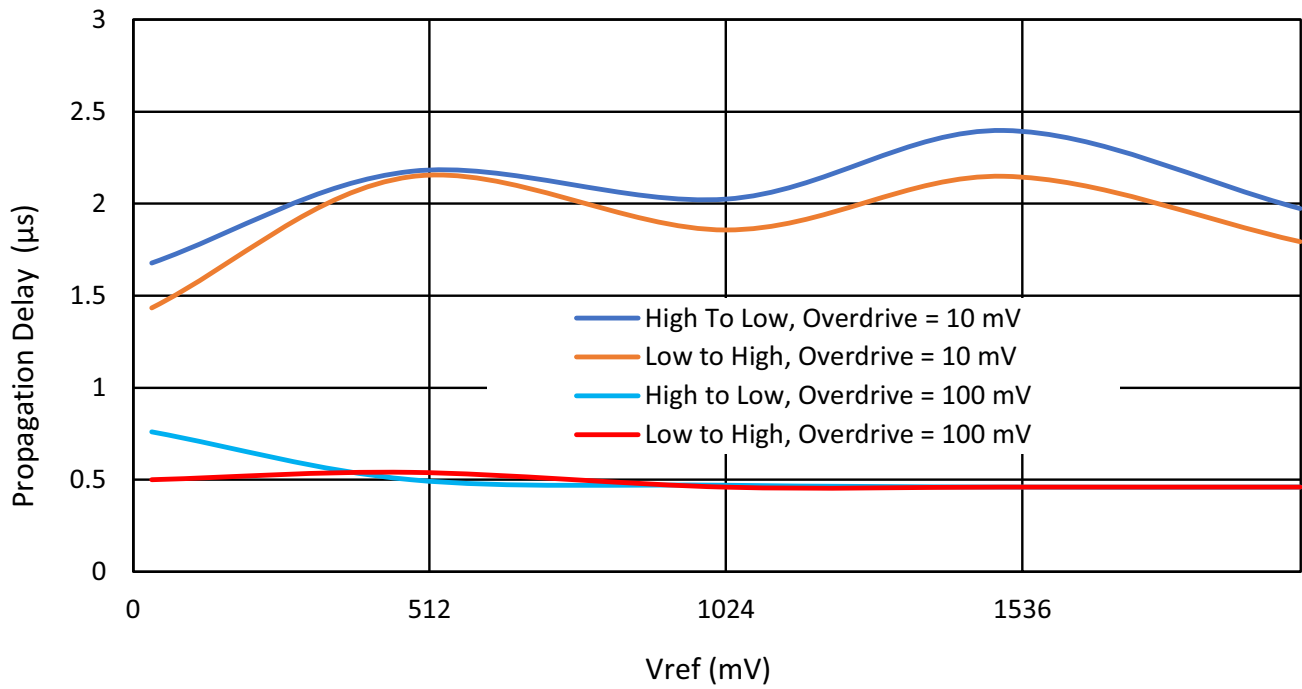
Figure 102. Propagation Delay vs. Vref for ACMPxH at T = 25 °C, at V DD = 2.3 V to 5.5 V, Gain = 1, Hysteresis = 0
