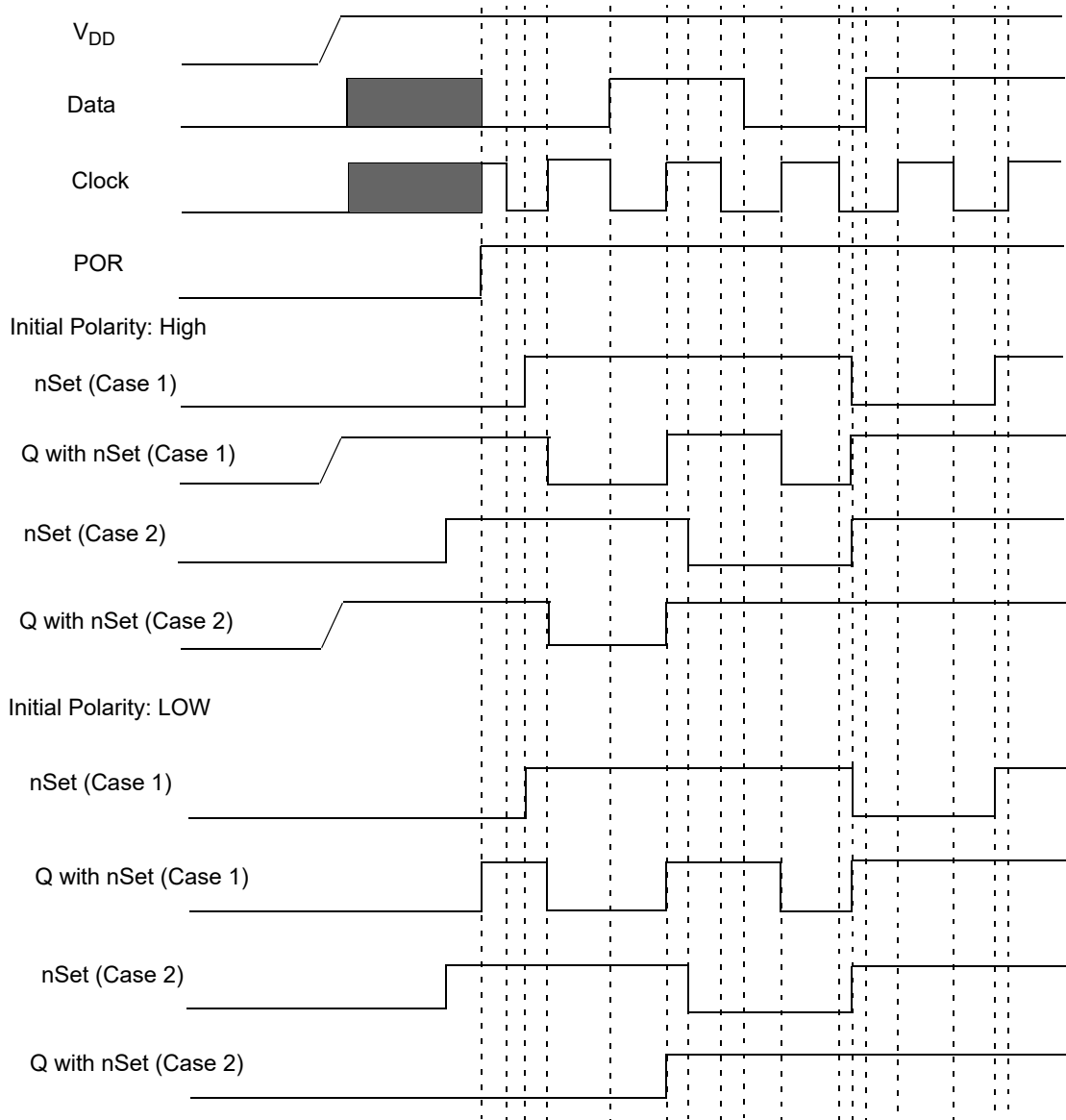
Figure 48. DFF Polarity Operations with nSet
