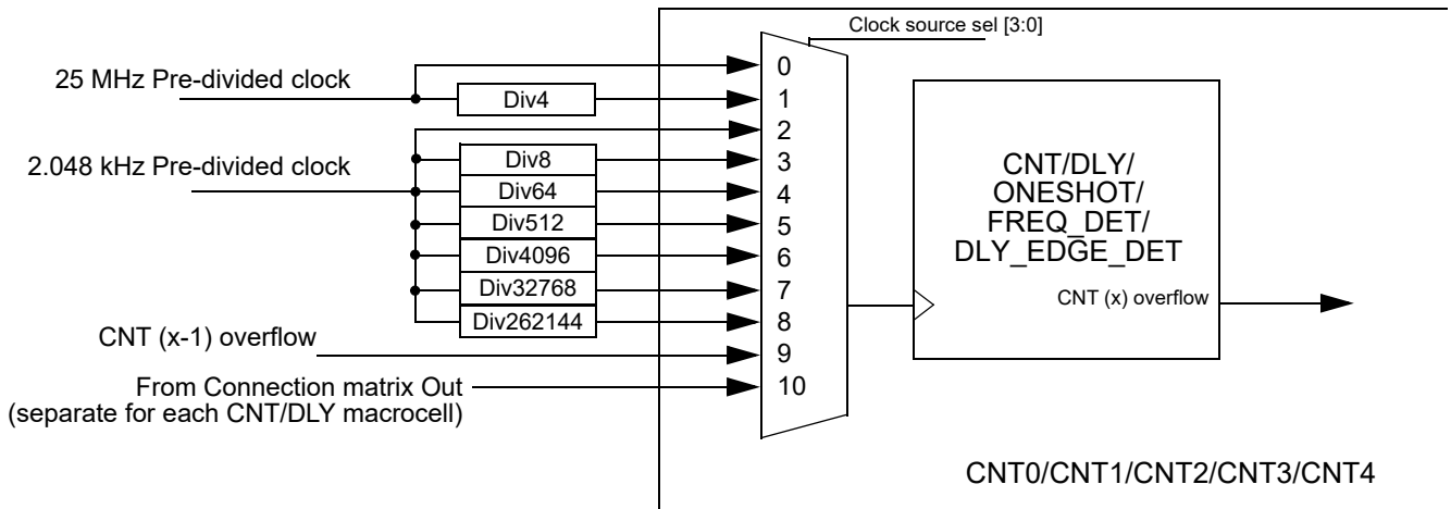
Figure 117. Clock Scheme
