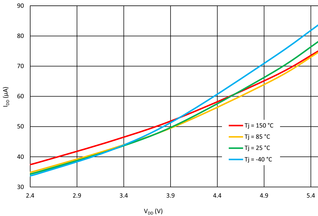
Figure 133. OSC1 Current Consumption vs. V DD (Pre-Divider = 12)
