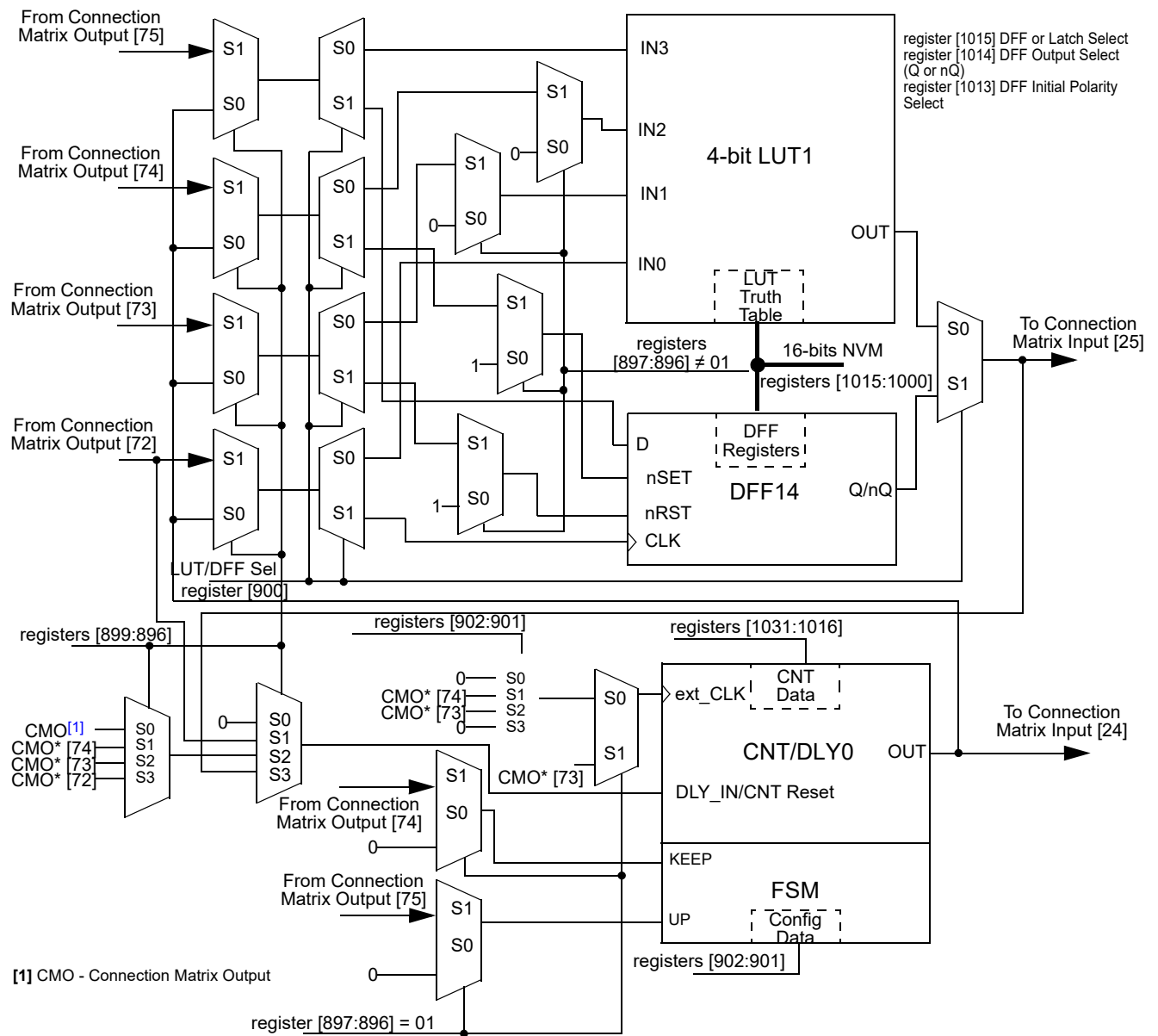
Figure 81. 16-bit Multi-Function Macrocell Block Diagram (4-bit LUT1/DFF14, CNT/DLY/FSM0)
