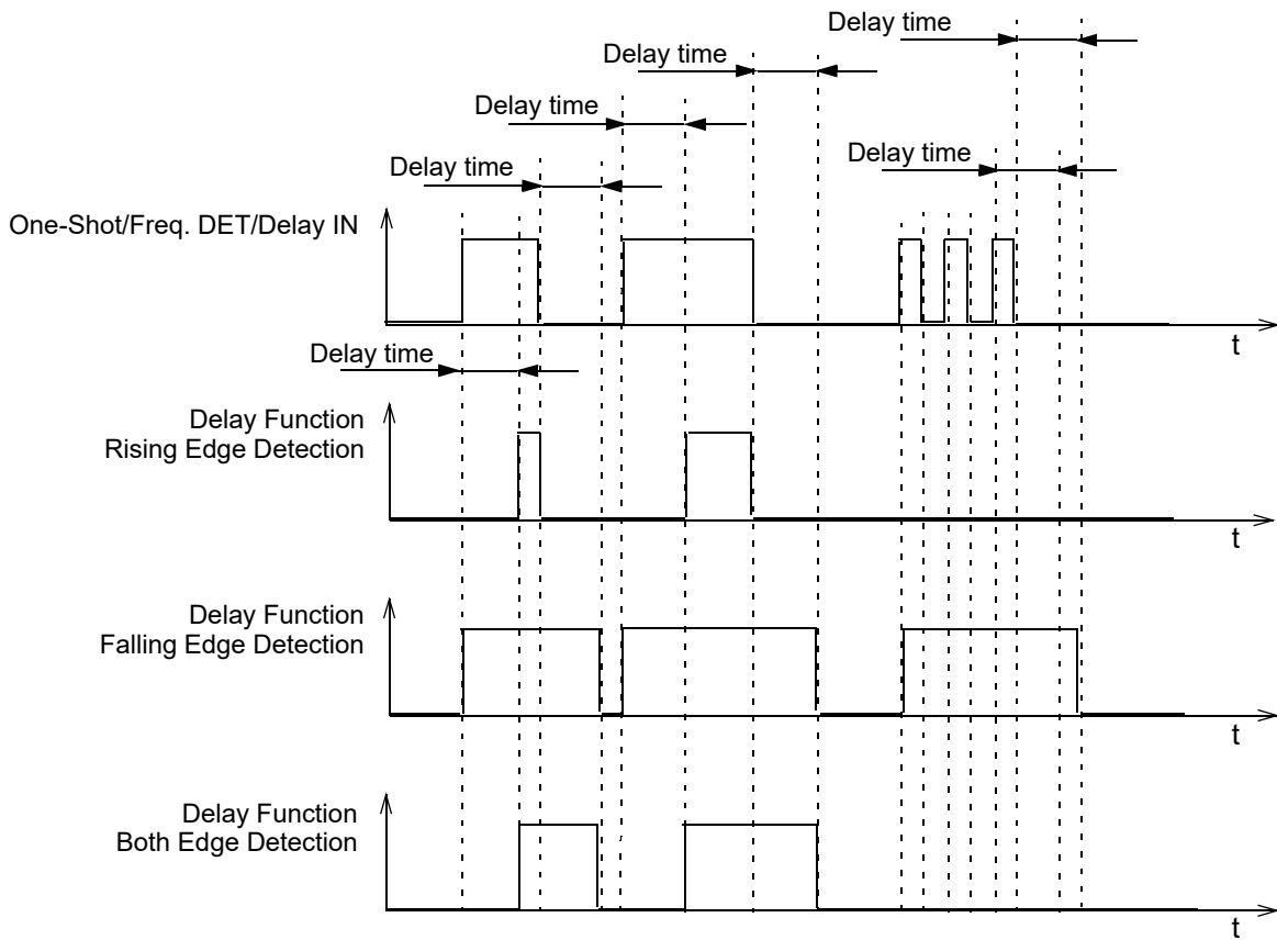
Figure 69. Delay Mode Timing Diagram for Different Edge Select Modes
