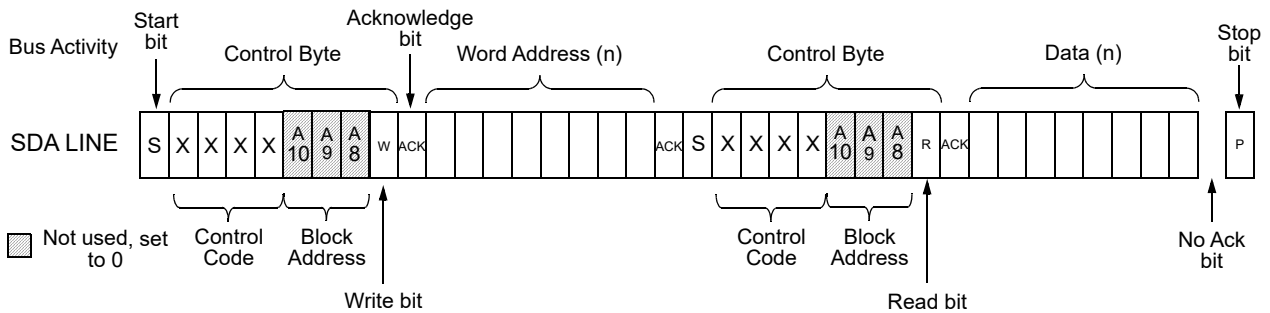
Figure 142. Random Read Command
