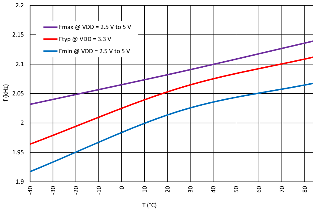
Figure 122. Oscillator0 Frequency vs. Temperature, OSC0 = 2.048 kHz
