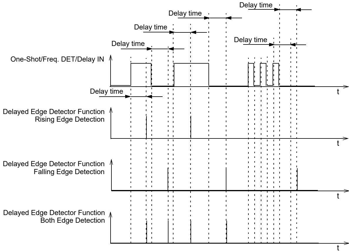
Figure 75. Delayed Edge Detection Mode Timing Diagram
