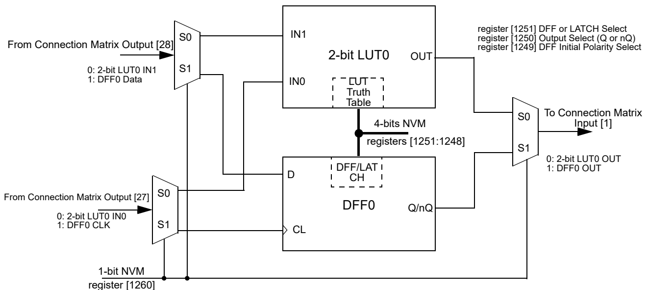
Figure 37. 2-bit LUT0 or DFF0
