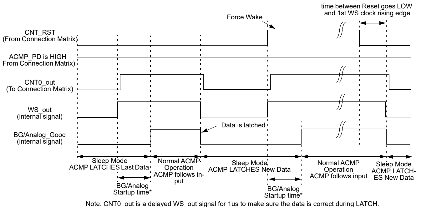
Figure 83. Wake/Sleep Timing Diagram, Normal Wake Mode, Counter Reset is Used
