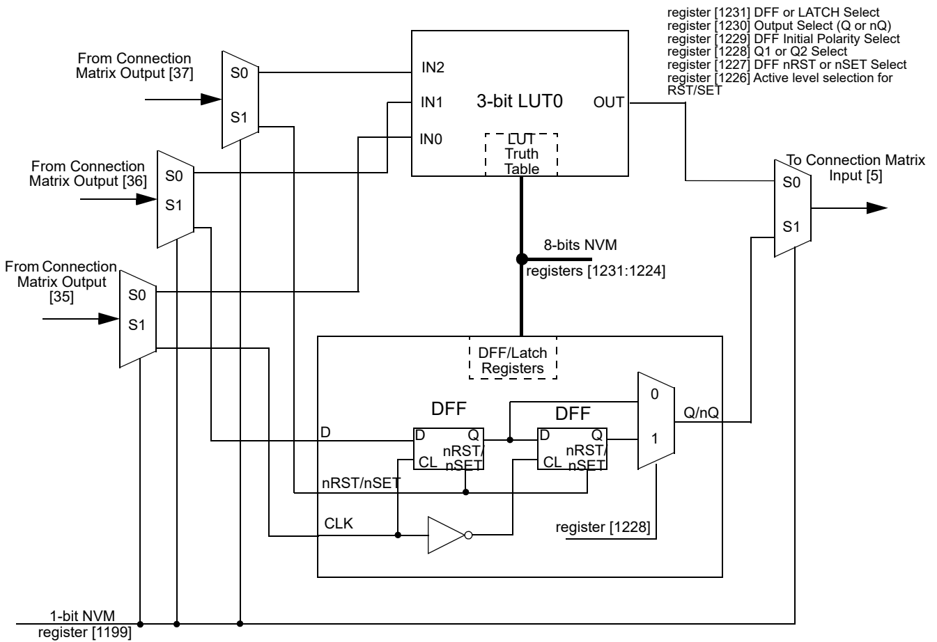
Figure 43. 3-bit LUT0 or DFF3
