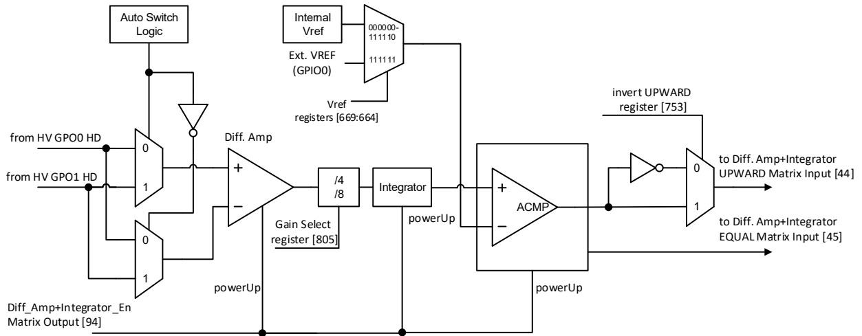
Figure 28. Differential Amplifier with Integrator Block Diagram
