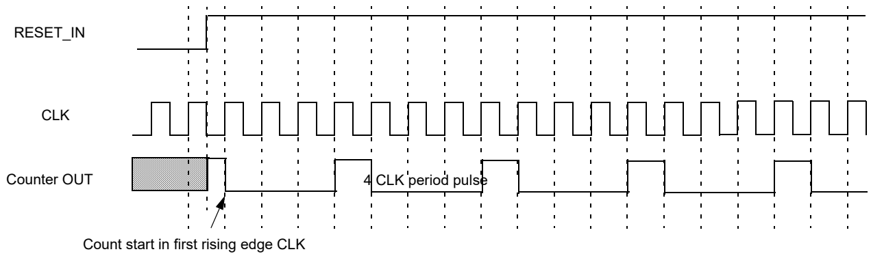
Figure 70. Counter Mode Timing Diagram without Two DFFs Synced Up
