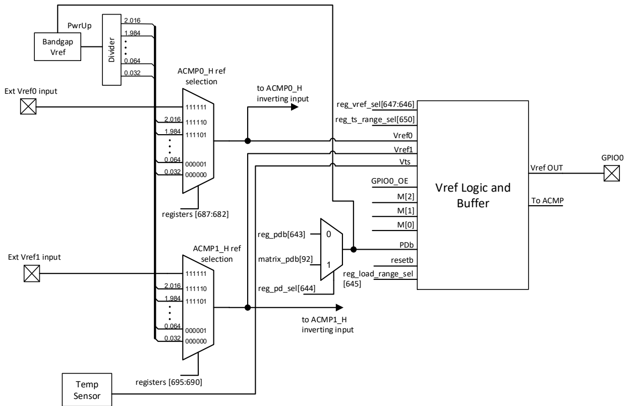
Figure 110. Voltage Reference Block Diagram
