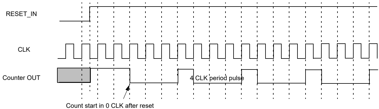
Figure 71. Counter Mode Timing Diagram with Two DFFs Synced Up
