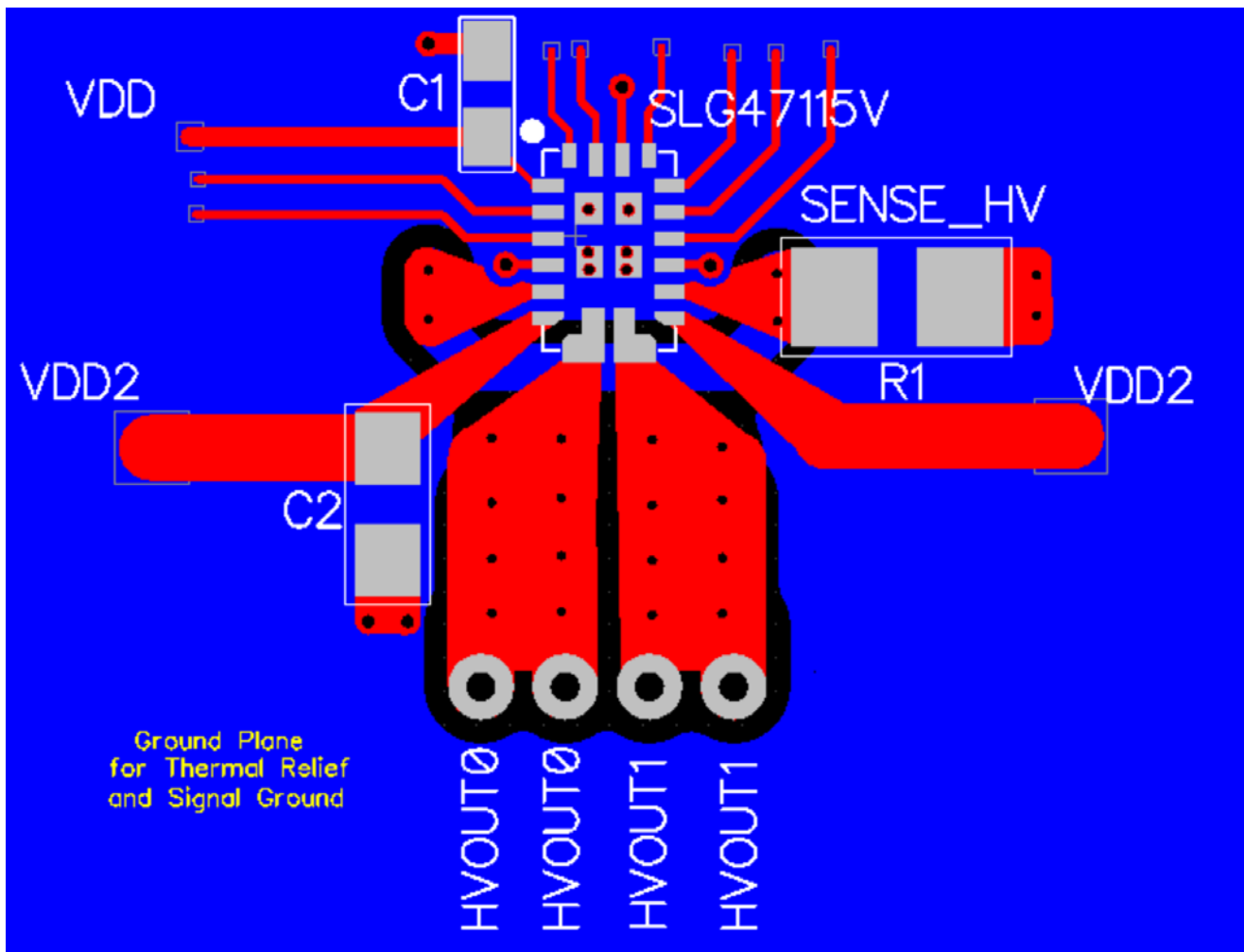
Figure 151. PCB Layout Example
