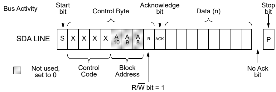
Figure 141. Current Address Read Command, R/W = 1
