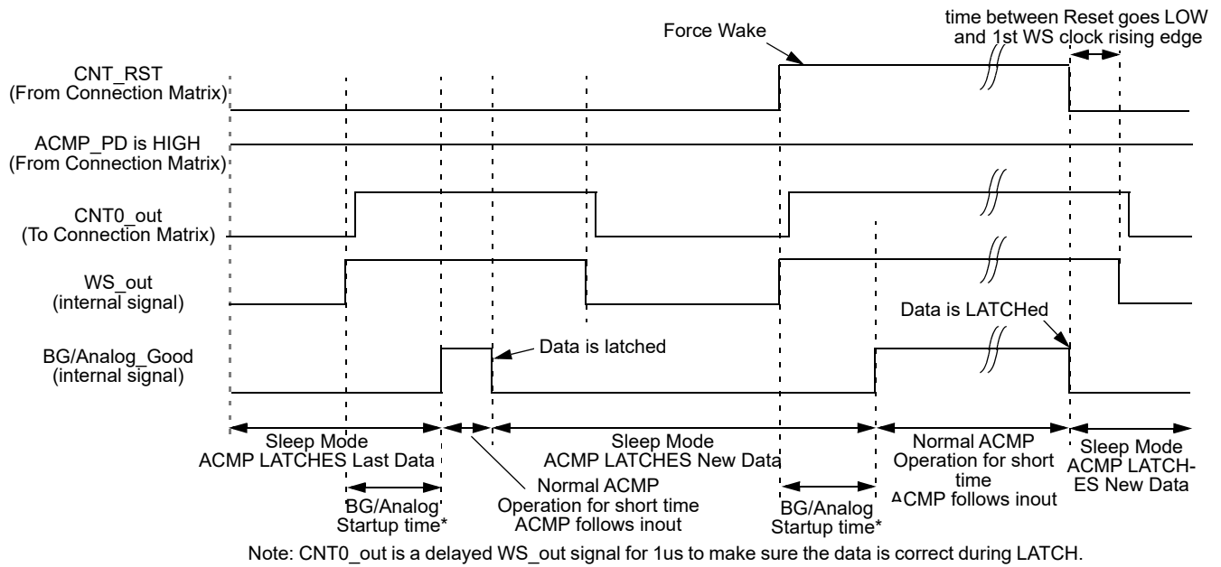
Figure 84. Wake/Sleep Timing Diagram, Short Wake Mode, Counter Reset is Used
