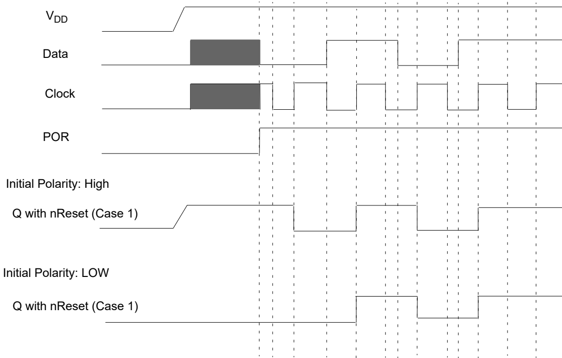
Figure 40. DFF Polarity Operations
