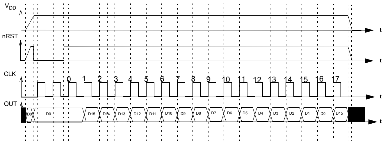
Figure 42. PGen Timing Diagram
