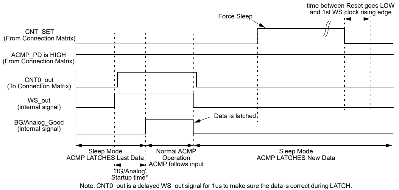
Figure 85. Wake/Sleep Timing Diagram, Normal Wake Mode, Counter Set is Used
