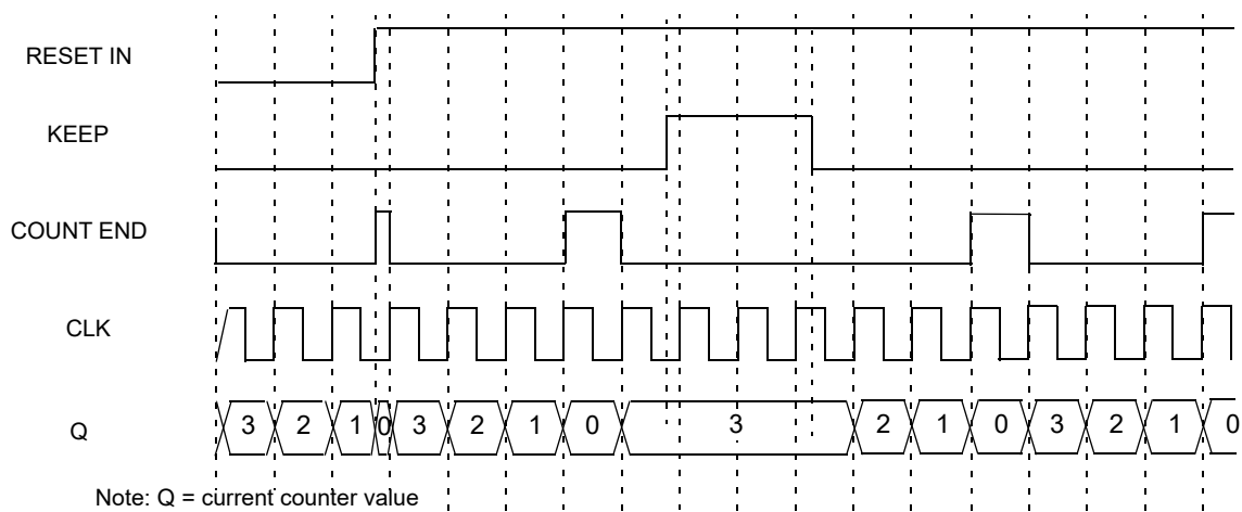
Figure 76. CNT/FSM Timing Diagram (Reset Rising Edge Mode, Oscillator is Forced On, UP = 0) for Counter Data = 3
