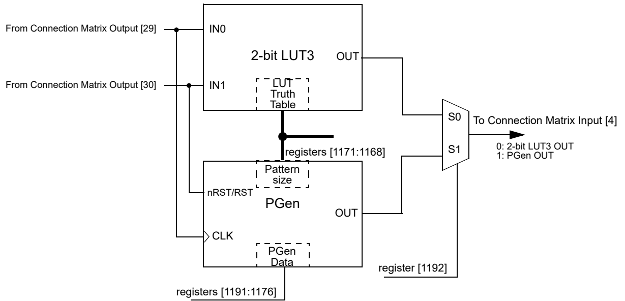
Figure 41. 2-bit LUT3 or PGen
