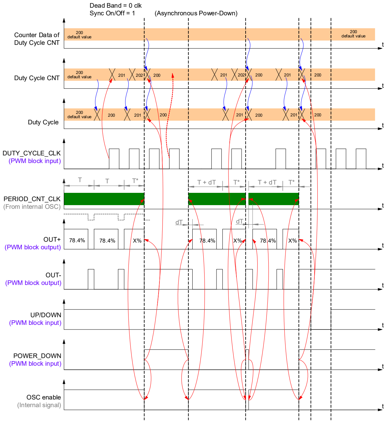
Figure 90. Power-Down with SYNC On/Off = 1 and Dead Band = 0 CLK
