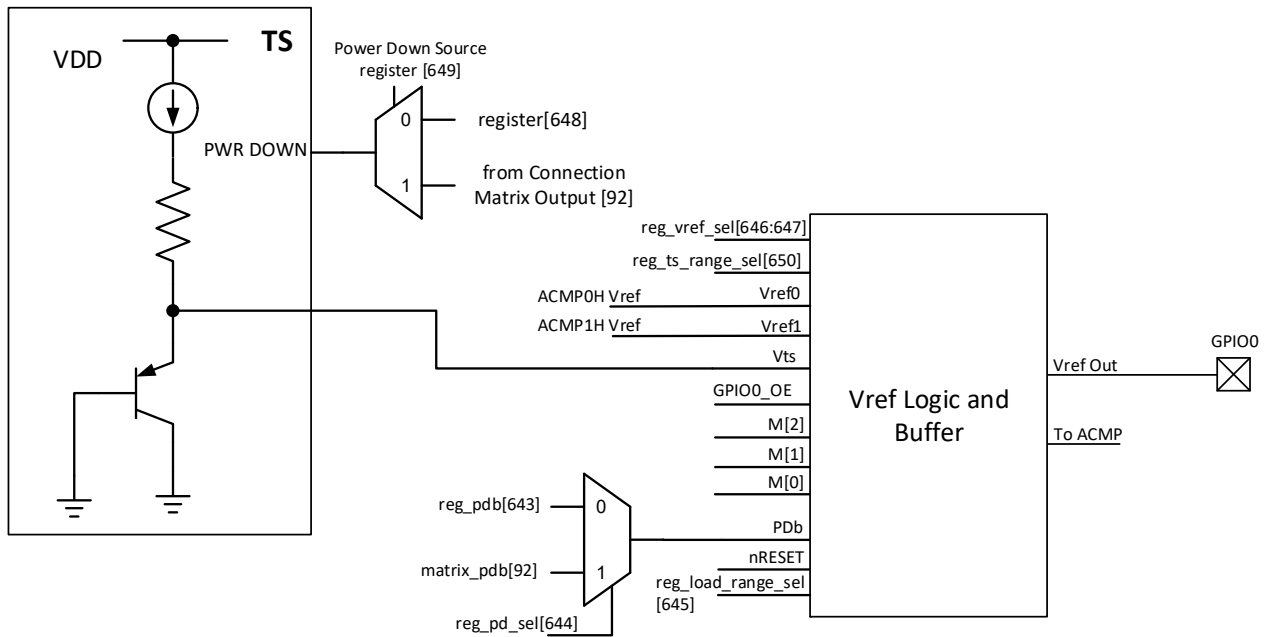
Figure 146. Analog Temperature Sensor Structure Diagram
