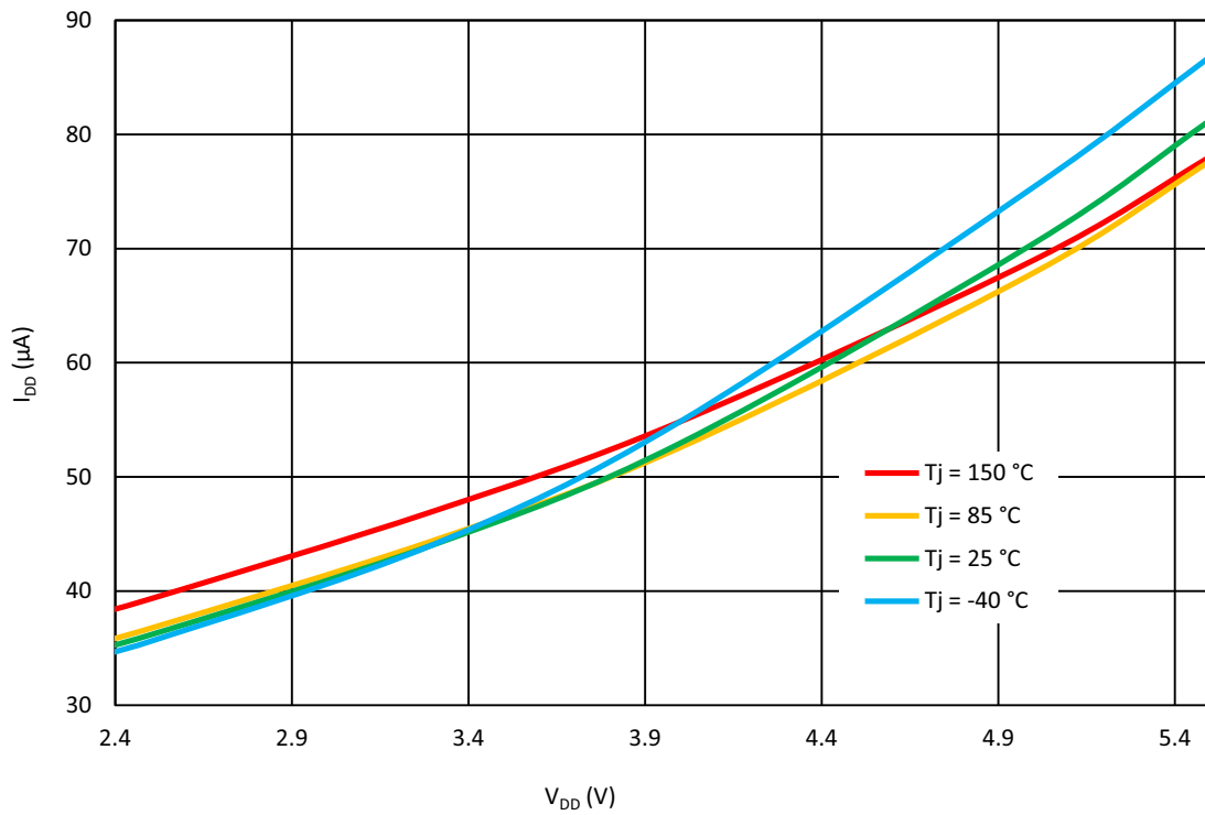
Figure 132. OSC1 Current Consumption vs. V DD (Pre-Divider = 8)
