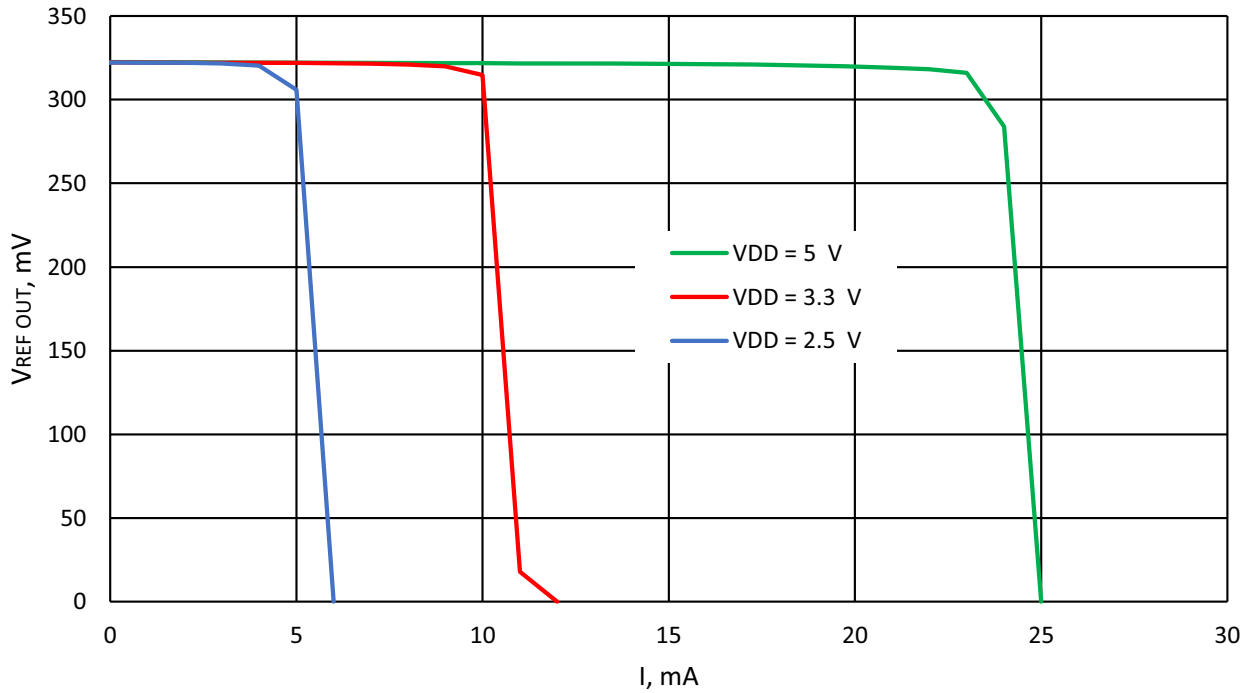
Figure 111. Typical Load Regulation, Vref = 320 mV, T = -40 °C to +85 °C, Buffer - Enabled
