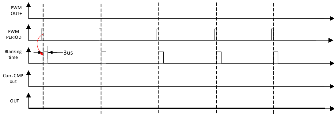
Figure 56. PWM Chopper. 0 % Duty Cycle
