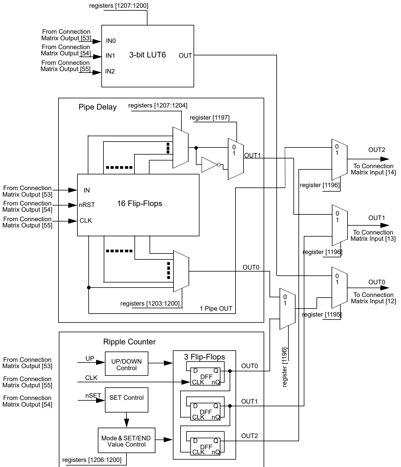
Figure 60. 3-bit LUT6/Pipe Delay/Ripple Counter
