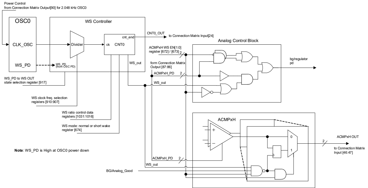
Figure 82. Wake/Sleep Controller
