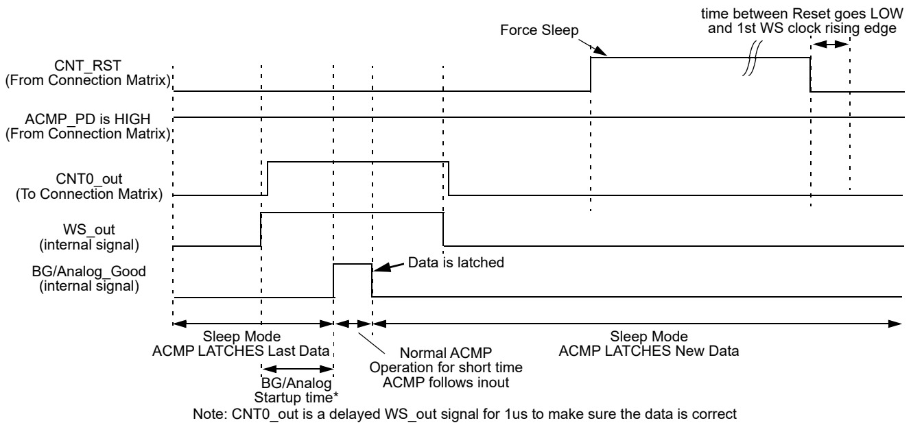
Figure 86. Wake/Sleep Timing Diagram, Short Wake Mode, Counter Set is Used
