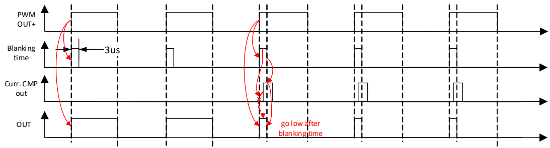
Figure 54. PWM Chopper. Overcurrent Start during Blanking Time
