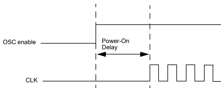
Figure 119. Oscillator Startup Diagram
