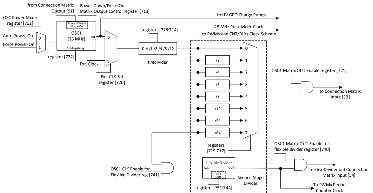
Figure 116. Oscillator1 Block Diagram
