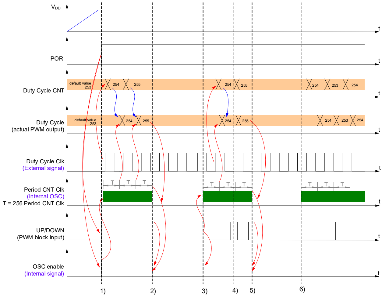
Figure 94. Example of PWM Auto Oscillator Control
