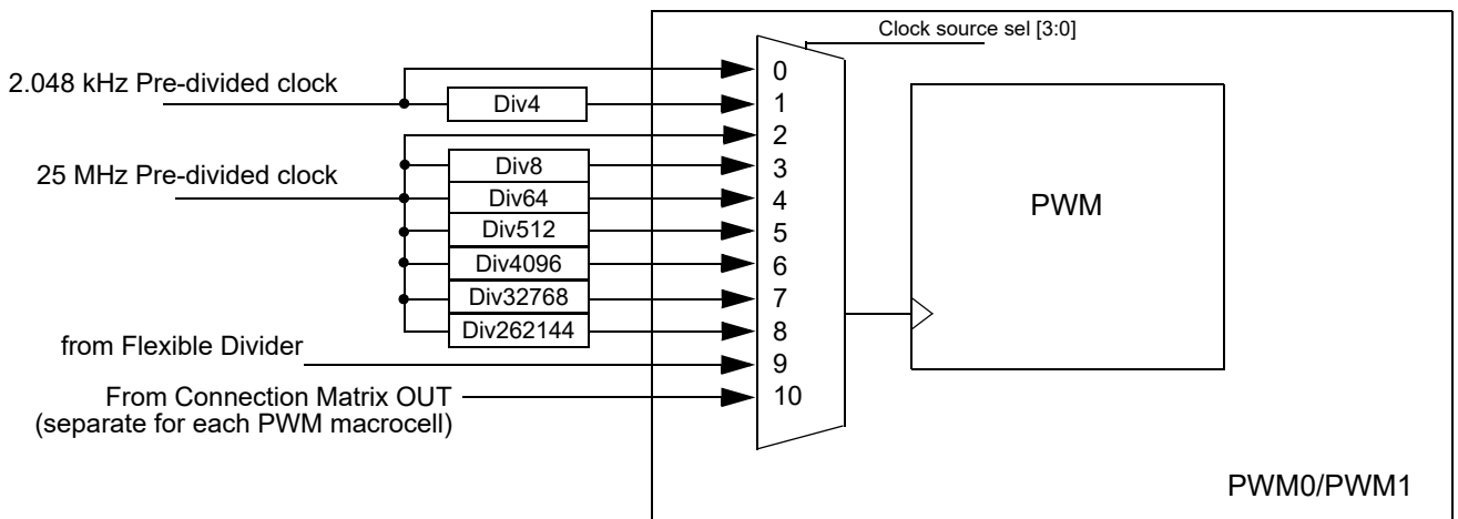
Figure 118. PWM Clock Scheme
