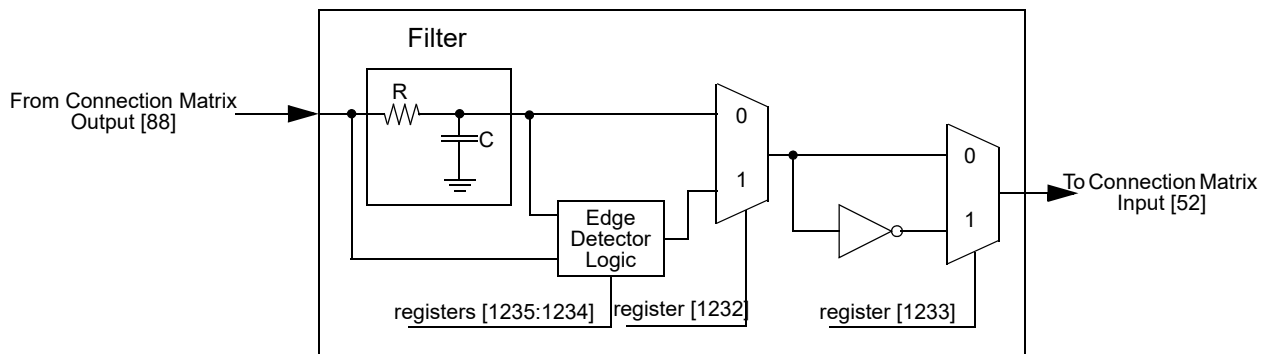
Figure 109. Deglitch Filter/Edge Detector
