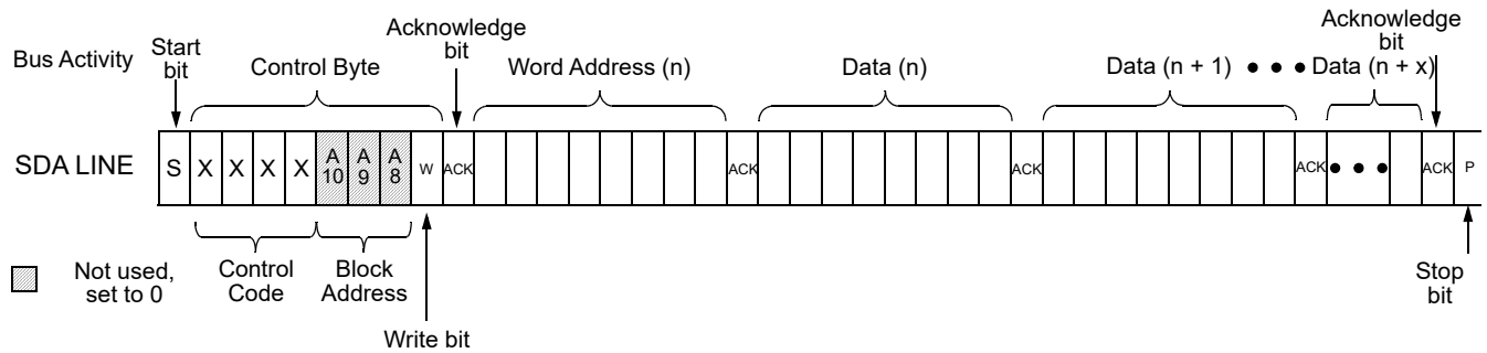
Figure 140. Sequential Write Command
