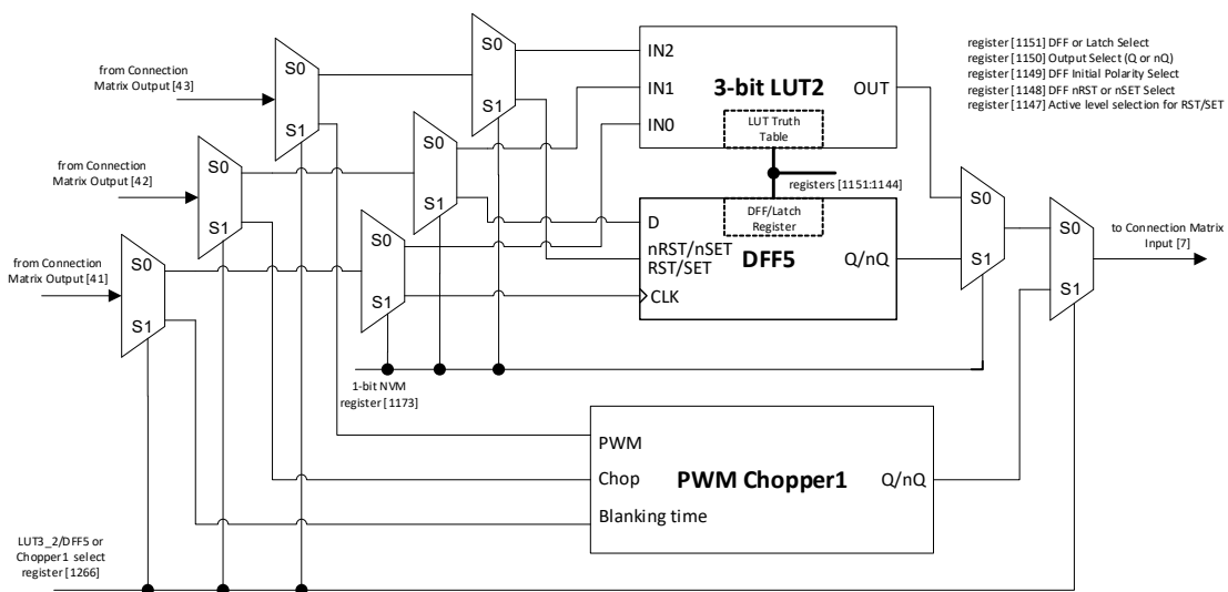
Figure 50. 3-bit LUT2 or DFF5
