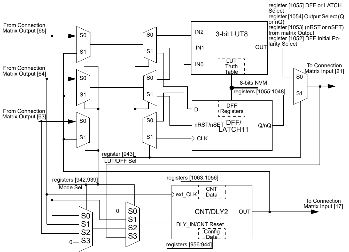
Figure 65. 8-bit Multi-Function Macrocells Block Diagram (3-bit LUT8/DFF11, CNT/DLY2)
