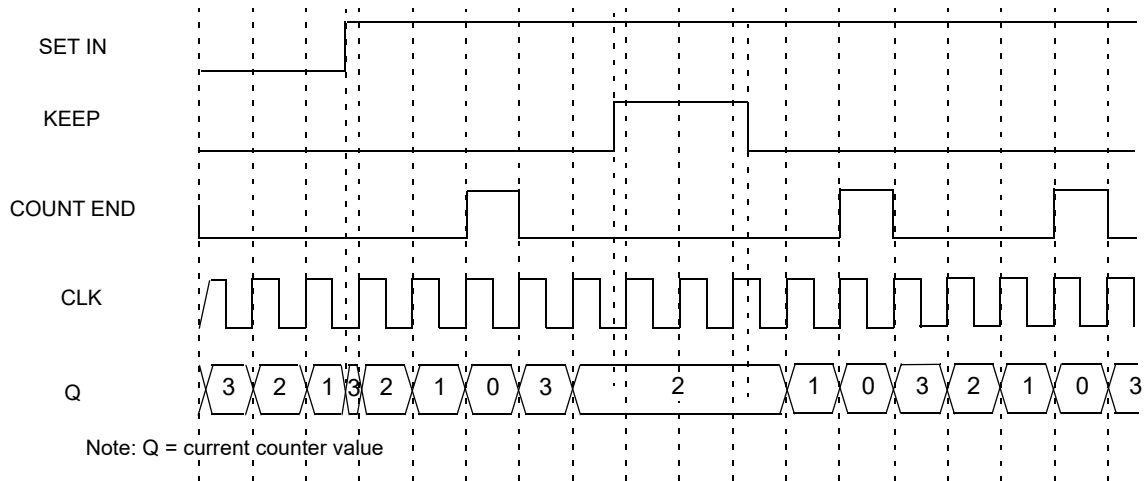
Figure 77. CNT/FSM Timing Diagram (Set Rising Edge Mode, Oscillator is Forced On, UP = 0) for Counter Data = 3
