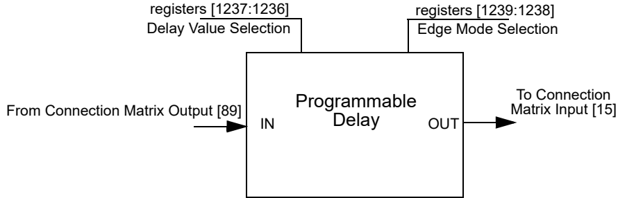
Figure 107. Programmable Delay
