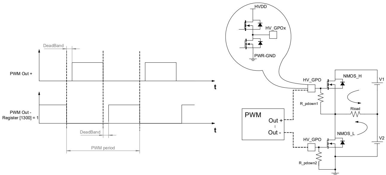
Figure 87. PWM Output Waveforms and Test Circuit Example for Driving NMOS FETs
