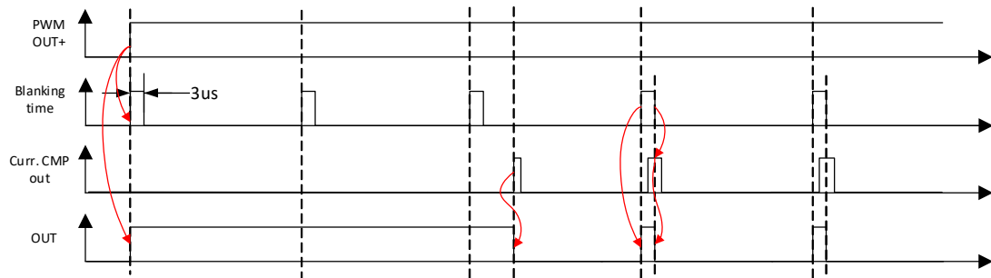
Figure 57. PWM Chopper. Overcurrent when 100 % Duty Cycle
