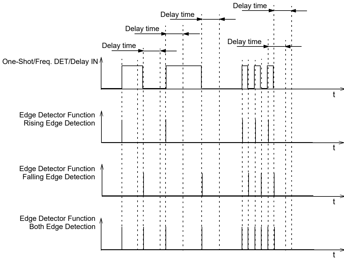
Figure 74. Edge Detection Mode Timing Diagram
