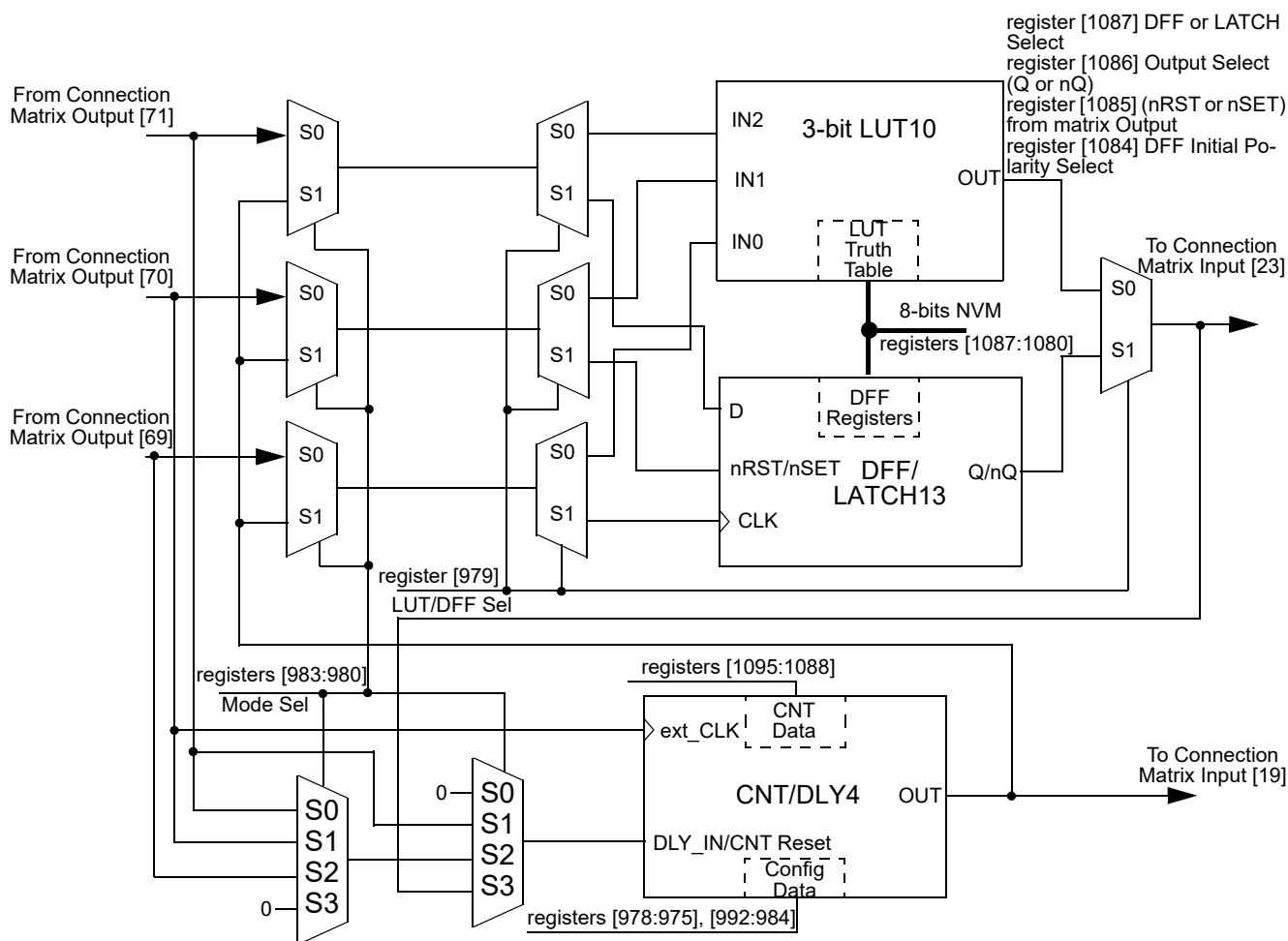
Figure 67. 8-bit Multi-Function Macrocells Block Diagram (3-bit LUT10/DFF13, CNT/DLY4)
