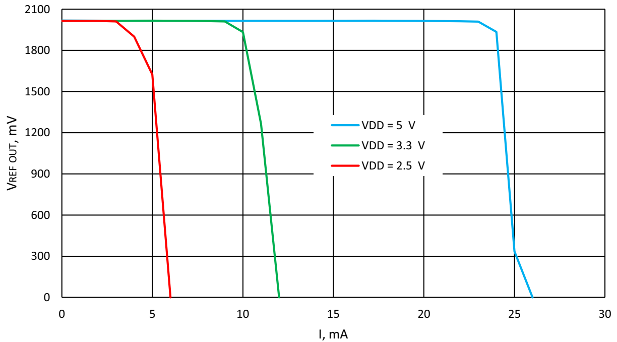
Figure 114. Typical Load Regulation, Vref = 2016 mV, T = -40 °C to +85 °C, Buffer - Enabled
