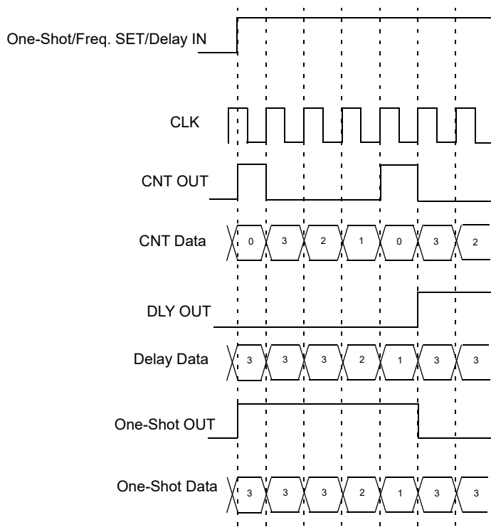
Figure 80. Counter Value, Counter Data = 3
