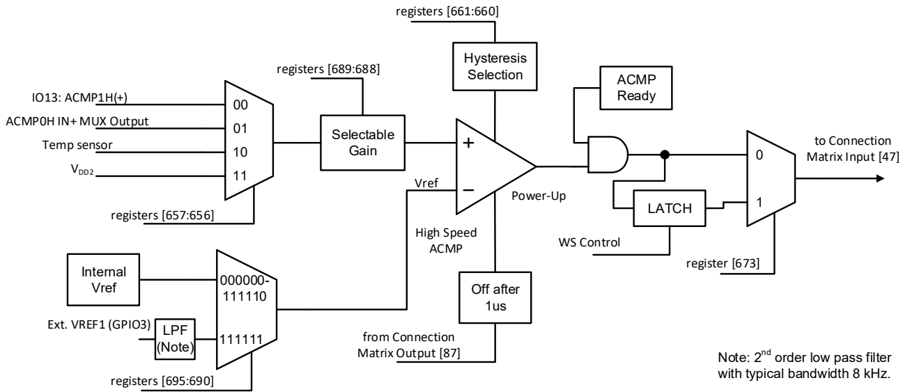
Figure 100. ACMP1H Block Diagram
