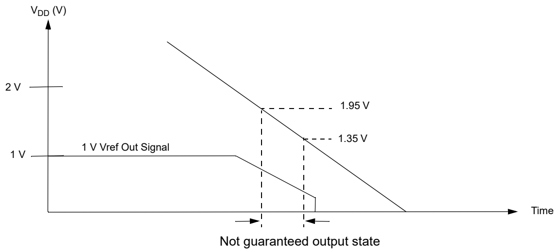
Figure 136. Power-Down
