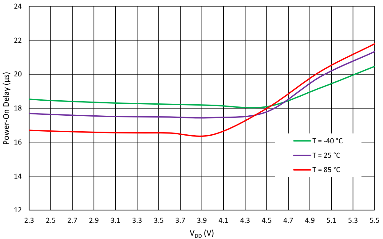
Figure 103. ACMPxH Power-On Delay vs. V DD
