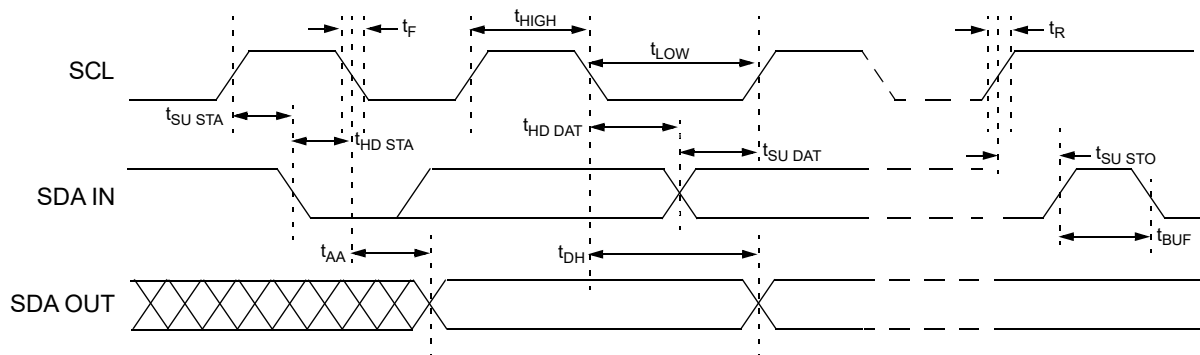
Figure 138. I 2 C General Timing Characteristics
