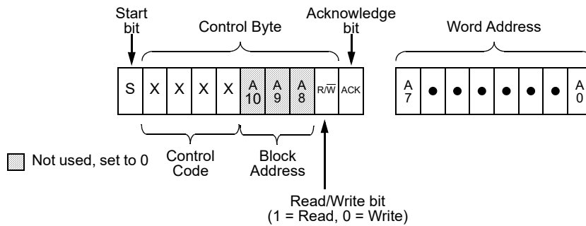
Figure 137. Basic Command Structure
