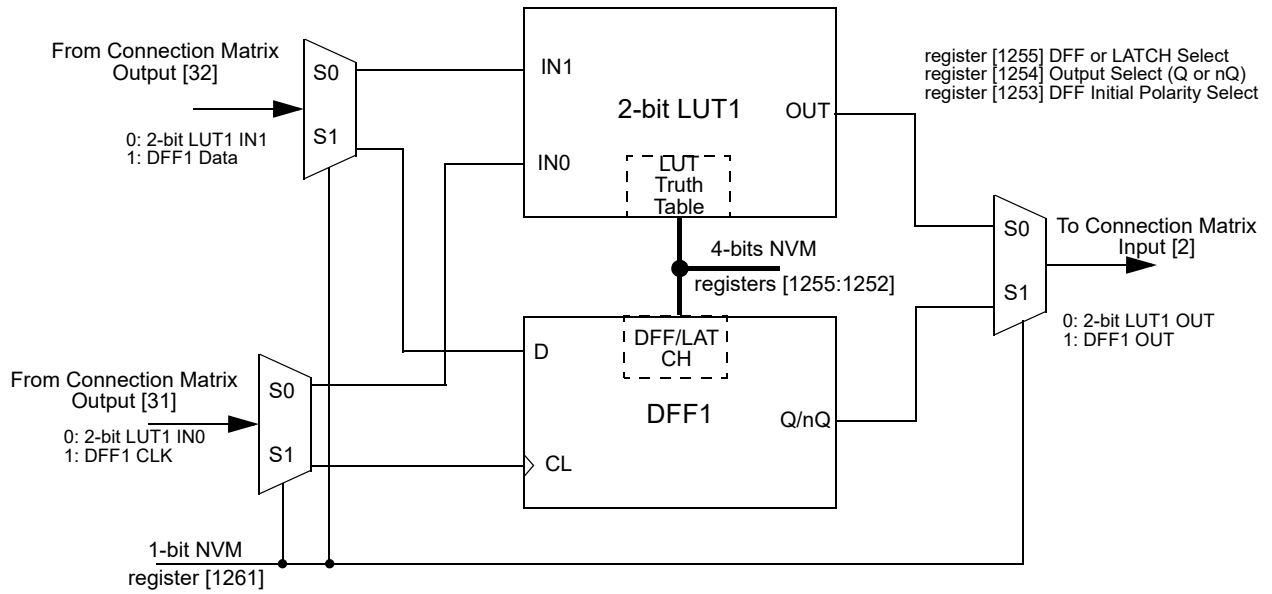
Figure 38. 2-bit LUT1 or DFF1
