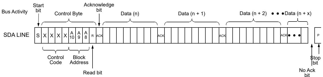
Figure 143. Sequential Read Command
