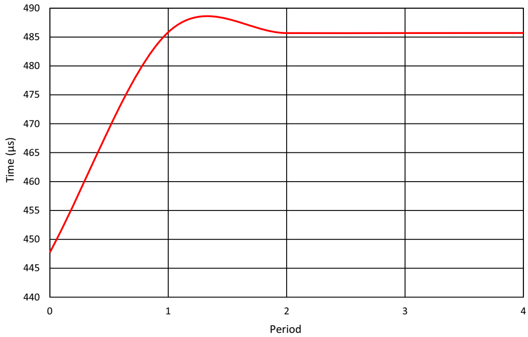
Figure 125. Oscillator0 Settling Time, V_{DD} = 3.3\text{ V} , T = 25\text{ }^{\circ}\text{C} , \text{OSC0} = 2\text{ kHz}
