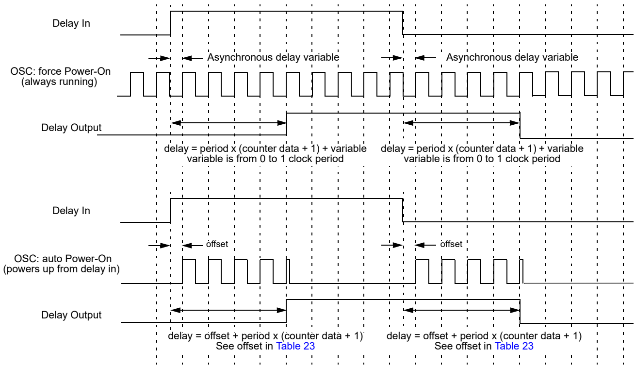
Figure 68. Delay Mode Timing Diagram, Edge Select: Both, Counter Data: 3
