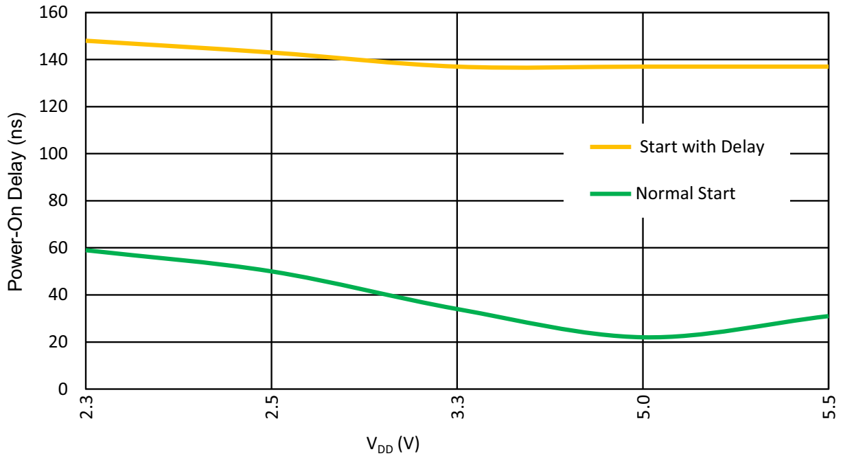
Figure 121. Oscillator1 Maximum Power-On Delay vs. V DD at T = 25 °C, OSC1 = 25 MHz
