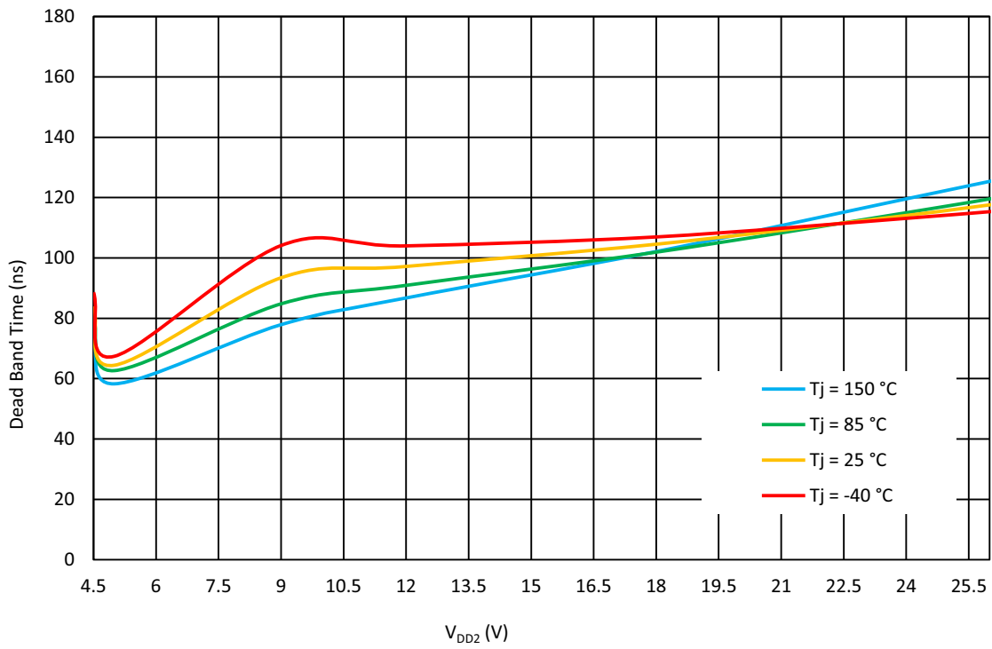
Figure 27. Half Bridge Dead Band Time vs. V DD2 at V DD = 2.3 V to 5.5 V, Falling Signal, f = 50 kHz for Regular Mode
