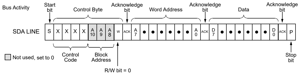
Figure 139. Byte Write Command, R/W = 0
