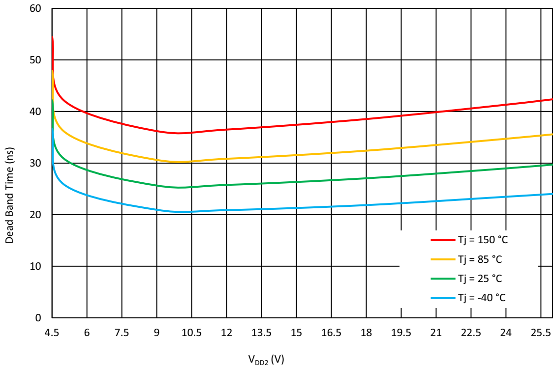
Figure 25. Half Bridge Dead Band Time vs. V DD2 at V DD = 2.3 V to 5.5 V, Falling Signal, f = 50 kHz for Pre-Driver Mode
