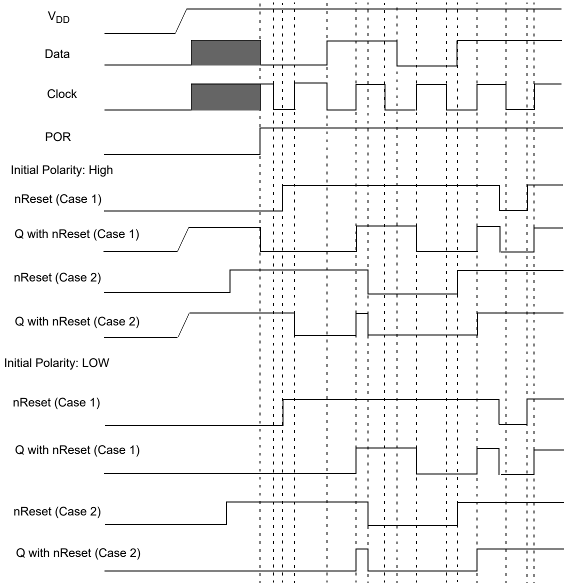
Figure 47. DFF Polarity Operations with nReset
