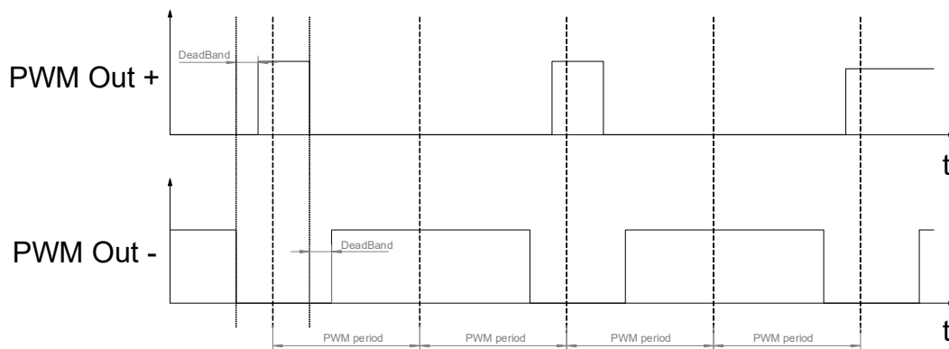
Figure 89. PWM Output Waveforms for Phase Correct PWM Mode
