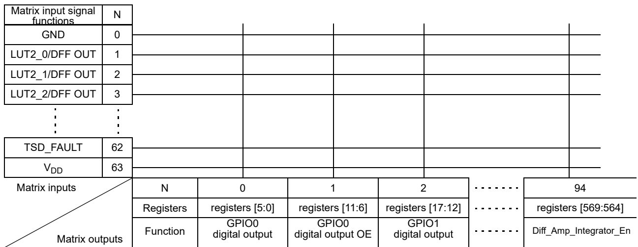
Figure 35. Connection Matrix
