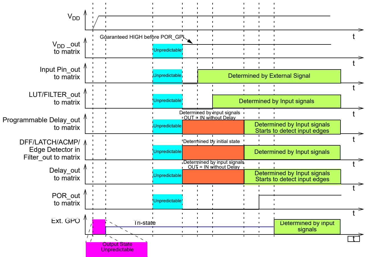
Figure 135. Internal Macrocell States during POR Sequence
