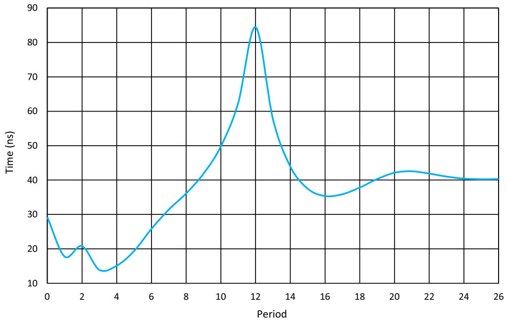
Figure 126. Oscillator1 Settling Time, V_{DD} = 3.3\text{ V} , T = 25\text{ }^{\circ}\text{C} , \text{OSC1} = 25\text{ MHz} (Normal Start)
