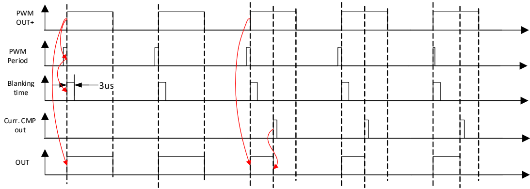
Figure 53. PWM Chopper. Overcurrent Timing Diagram
