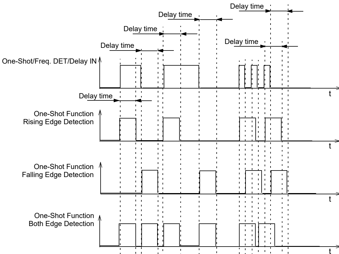
Figure 72. One-Shot Function Timing Diagram
