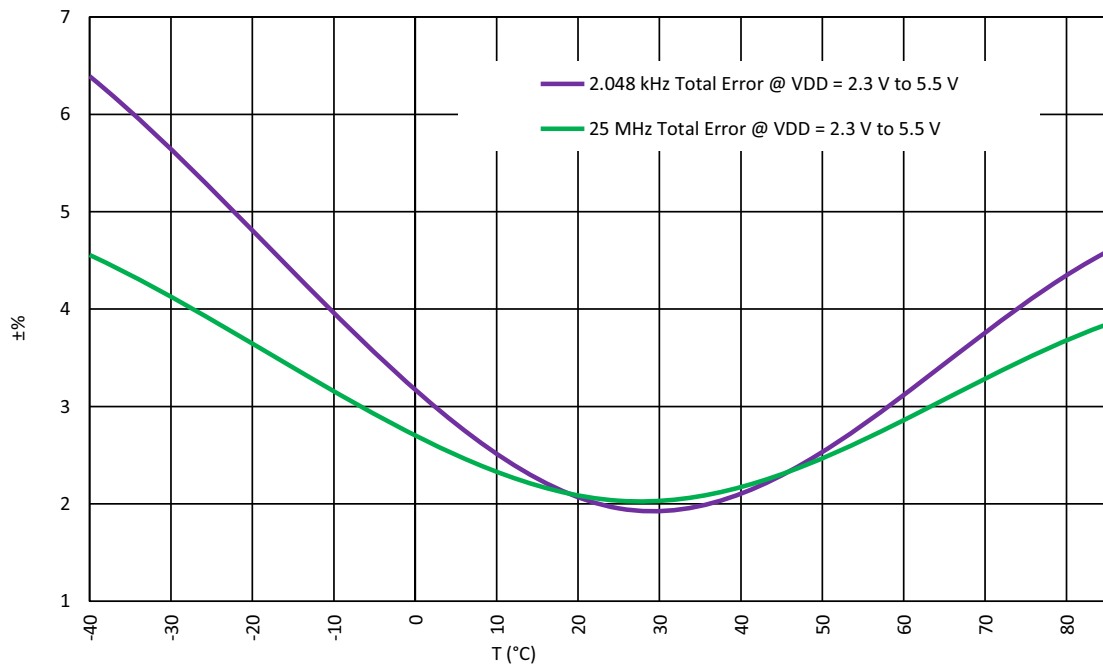
Figure 124. Oscillators Total error vs. Temperature
