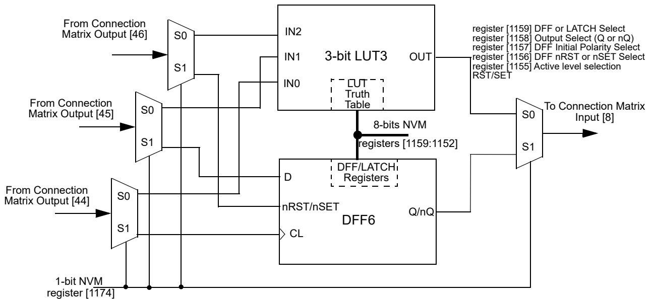
Figure 44. 3-bit LUT3 or DFF6
