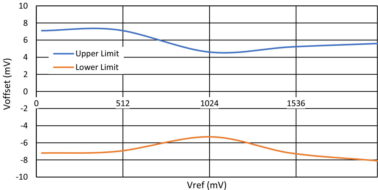
Figure 101. ACMPxH Input Offset Voltage vs. V ref at V DD = 2.3 V to 5.5 V, T = -40 °C to 85 °C,
