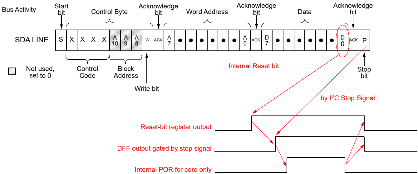
Figure 144. Reset Command Timing
