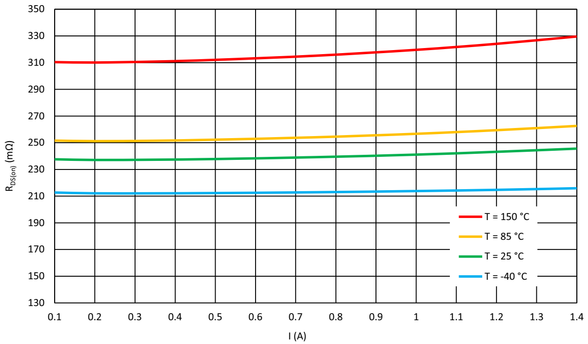
Figure 19. Full Bridge High Side Typical Drain-Source On-Resistance vs. Load Current at V_{DD} = 5.5\text{ V} , V_{DD2} = 5\text{ V}
