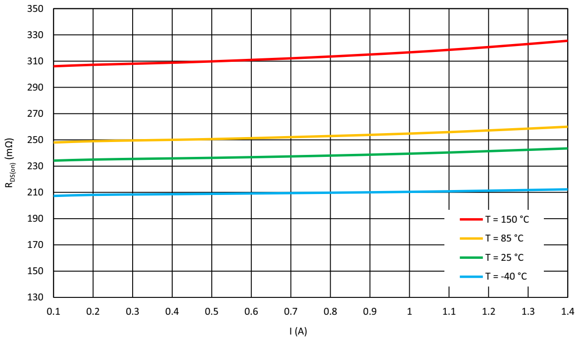
Figure 20. Full Bridge Low-Side Typical Drain-Source On-Resistance vs. Load Current at V_{DD} = 5.5\text{ V} , V_{DD2} = 5\text{ V}
