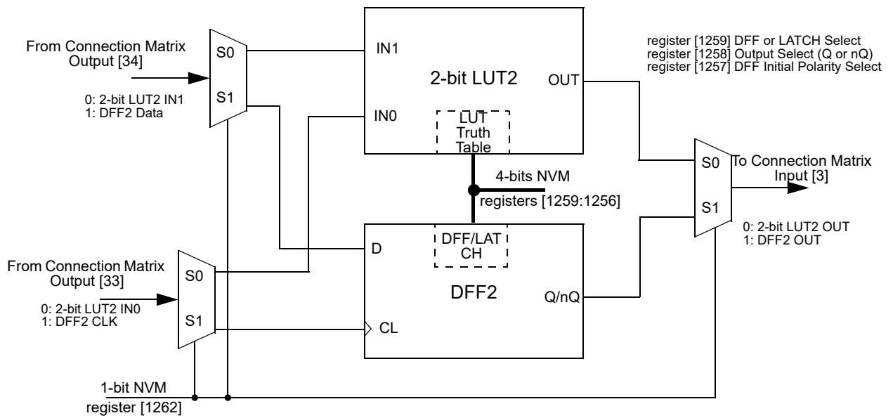
Figure 39. 2-bit LUT2 or DFF2
