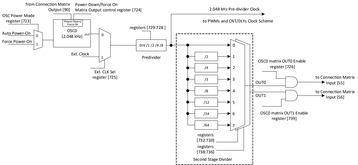
Figure 115. Oscillator0 Block Diagram
