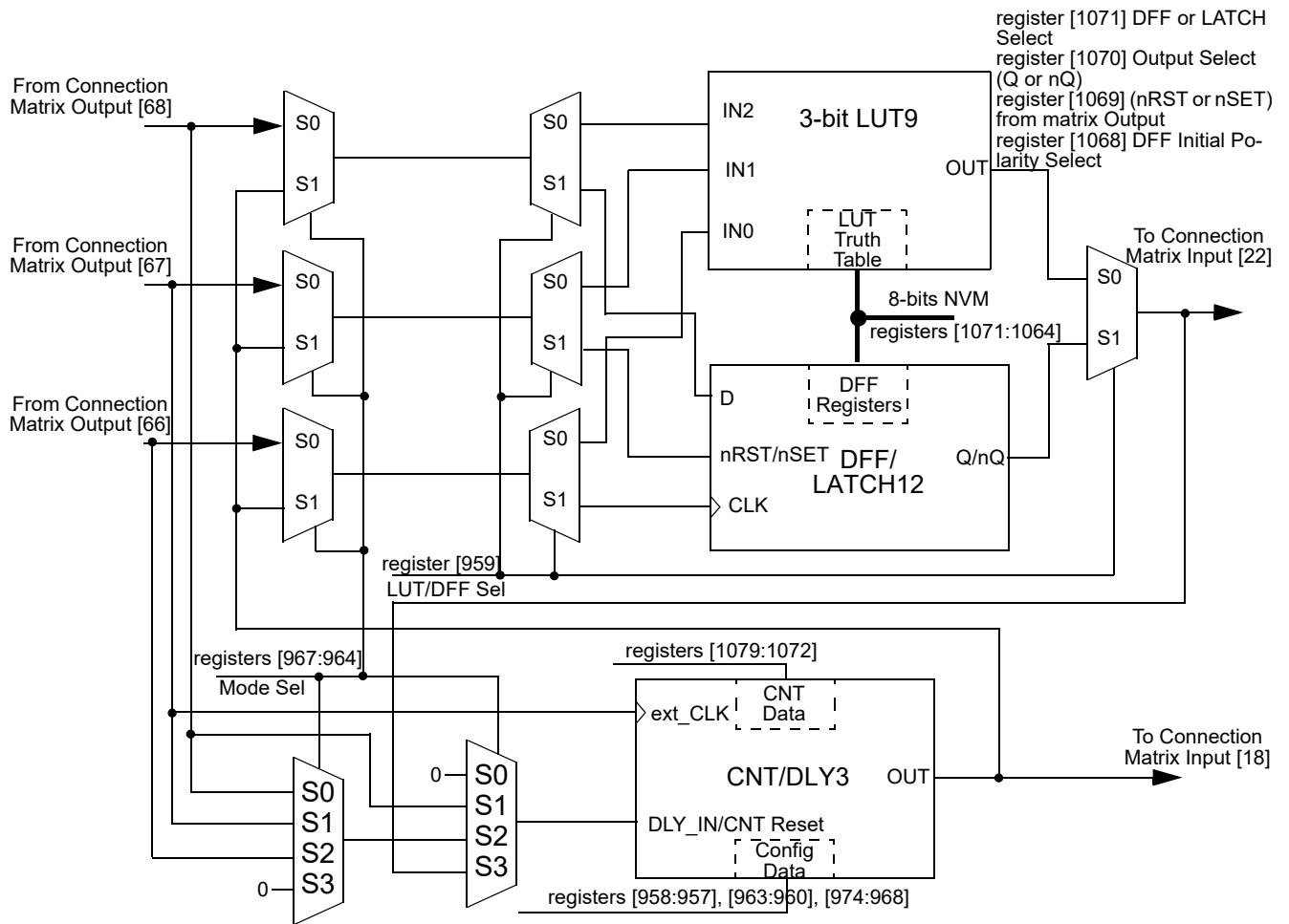
Figure 66. 8-bit Multi-Function Macrocells Block Diagram (3-bit LUT9/DFF12, CNT/DLY3)
