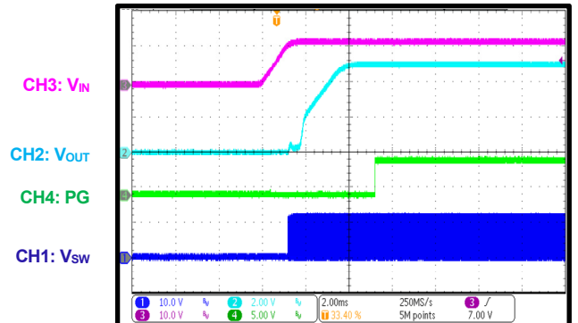
PG in Start-Up through VIN I_{OUT} = 3A
