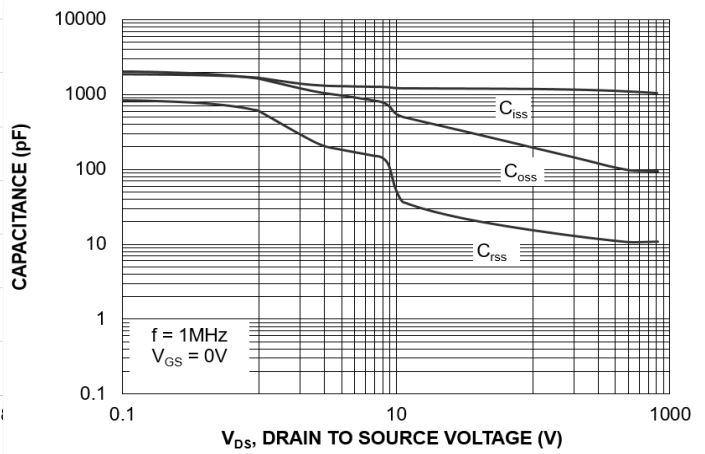
Figure 29. Capacitance Charge
