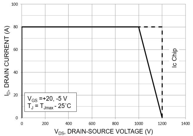
Figure 31. RBSOA
