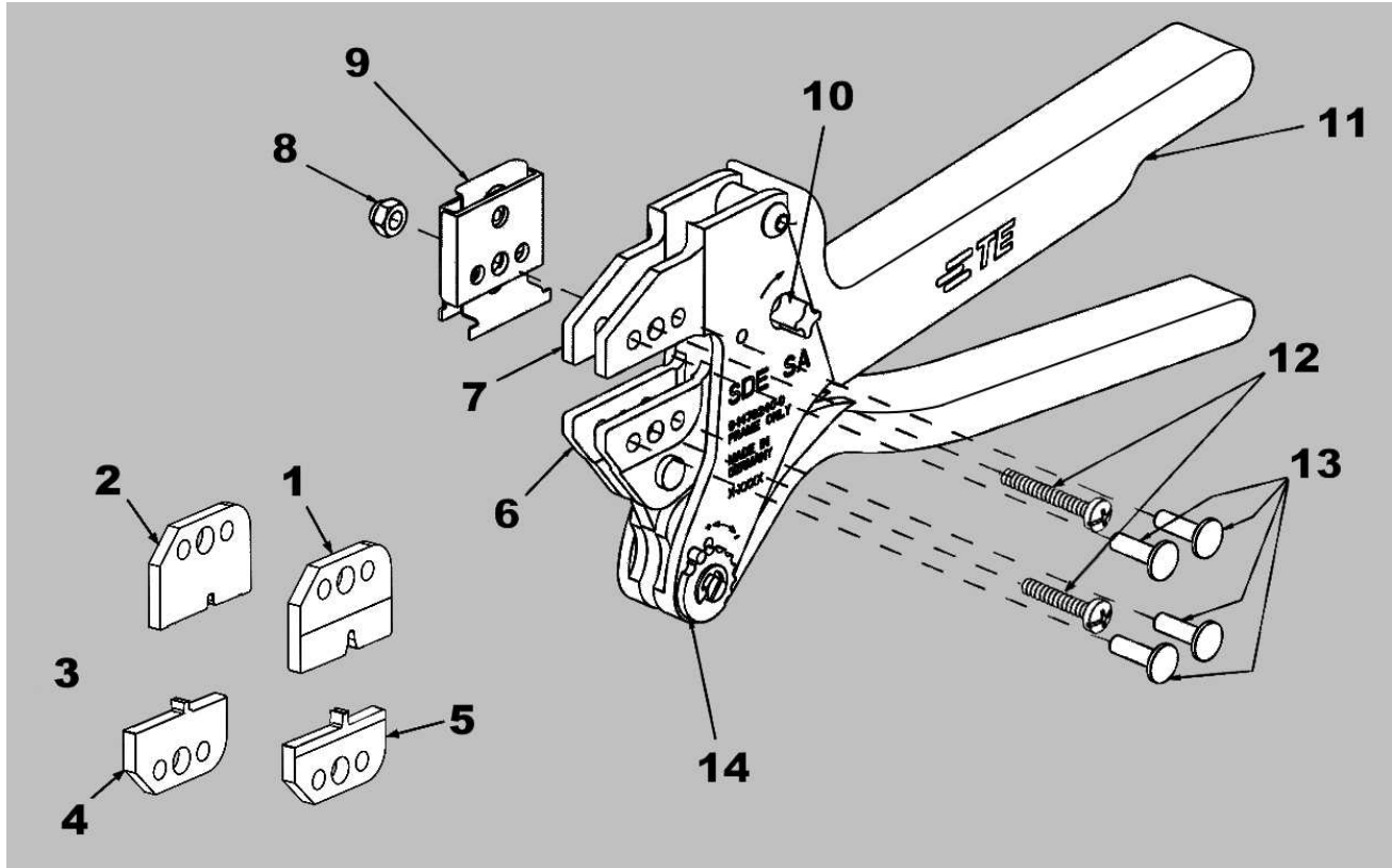
Figure 1: SDE-SA Commercial Hand Tool Assembly 2397569-1 with Die Assembly 2397569-2
