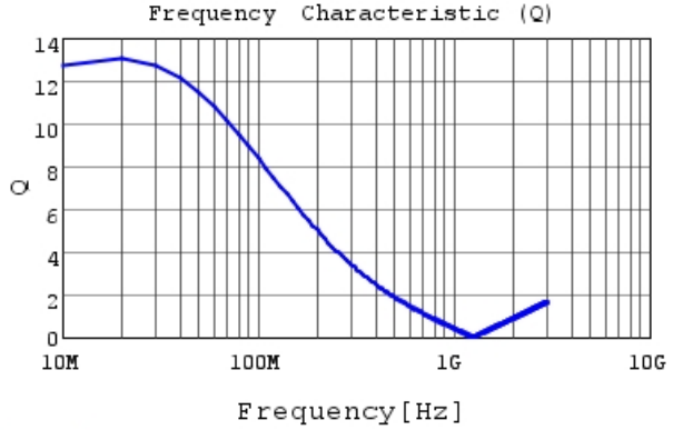
LQW18CNR39J0H Q
