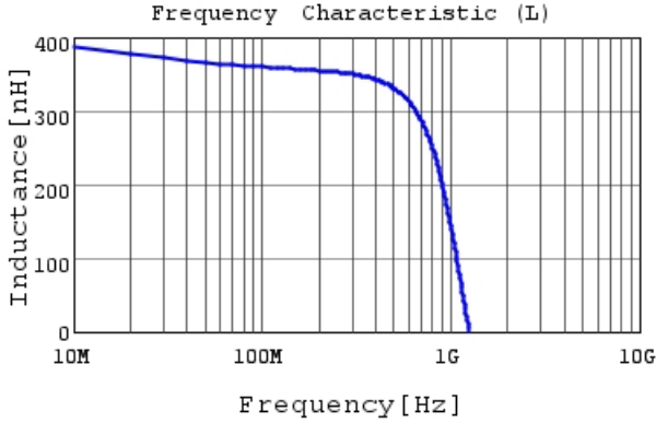
LQW18CNR39J0H L
