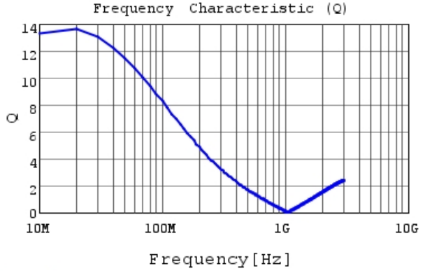
LQW18CNR56J0H Q
