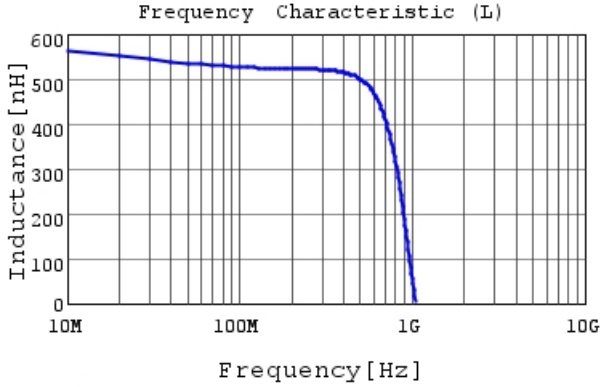
LQW18CNR56J0H L
