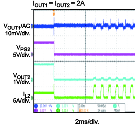
CH1 Steady State, CH2 SCP Entry I_{OUT1} = I_{OUT2} = 2A
