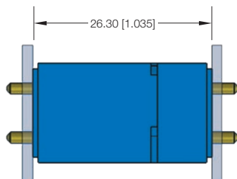
Straight PCB Mount (Male) to Straight PCB Mount (Female)
