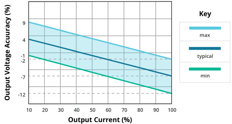
OUTPUT REGULATION CURVE VQA3-S12-D15-S (-Vo)
