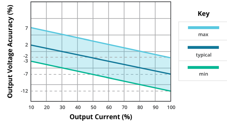
OUTPUT REGULATION CURVE VQA3-S15-D15-S (-Vo)
