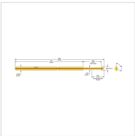
SPL-30T-021
