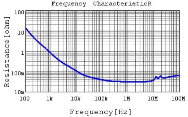
RDEC71H105K1K1H03B R DC0V, 25degC
