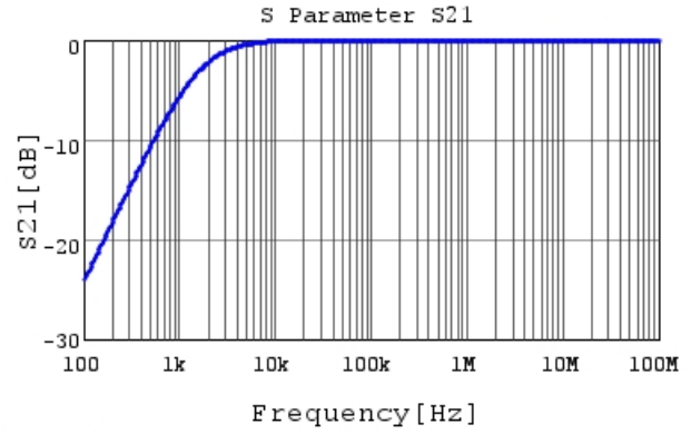
RDEC71H105K1K1H03B S21 DC0V, 25degC
