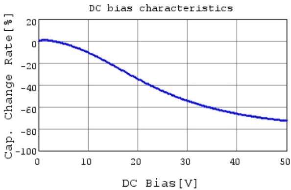
RDEC71H105K1K1H03B C-DC bias capchange, 25.0
