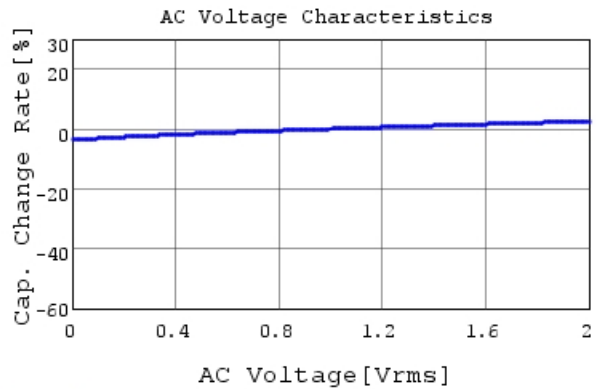
RDEC71H105K1K1H03B C-AC Voltage capchange, I
