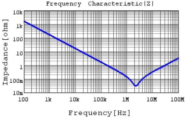
RDEC71H105K1K1H03B |Z| DC0V, 25degC
