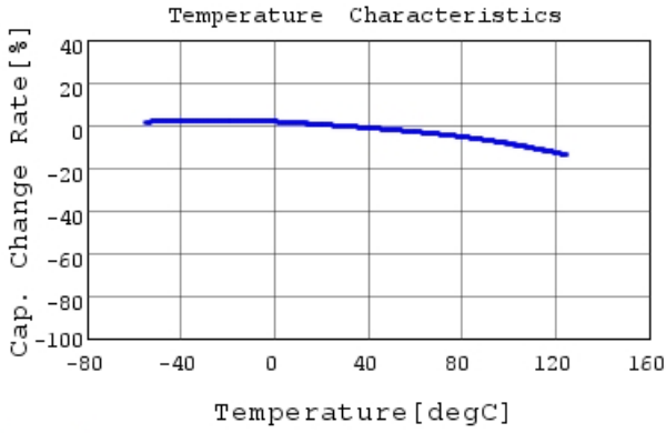
RDEC71H105K1K1H03B C-Temp. capchange, DC0.0V
