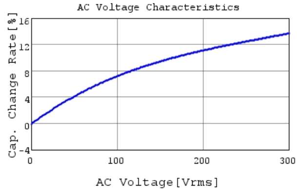
DE6B3KJ101KN3AE01J C-AC Voltage capchange, I
