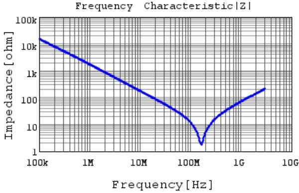
DE6B3KJ101KN3AE01J |Z| DC0V, 20degC
