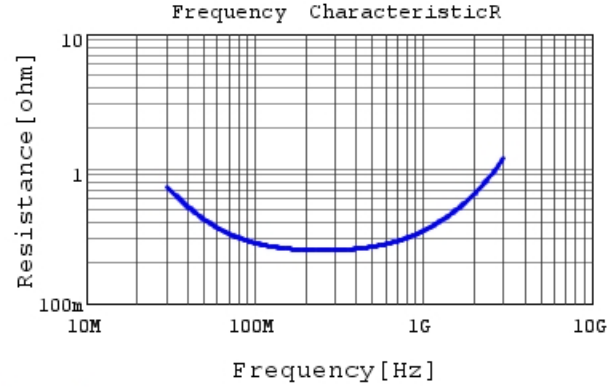
RCE5C2J270J1K1H03B R DC0V, 25degC
