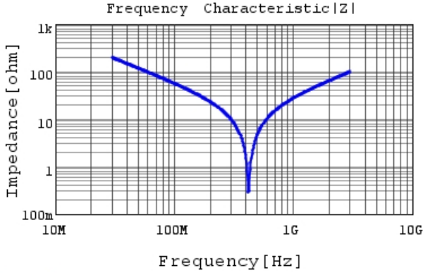
RCE5C2J270J1K1H03B |Z| DC0V, 25degC
