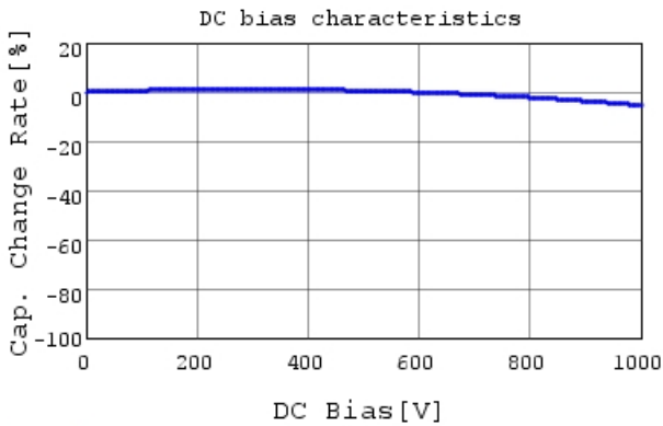
DE6B3KJ471KB3BE01J C-DC bias capchange, 20.0
