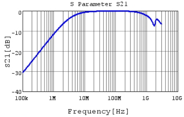
DE6B3KJ471KB3BE01J S21 DCOV, 20degC
