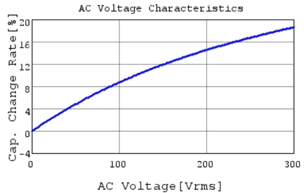
DE6B3KJ471KB3BE01J C-AC Voltage capchange, I
