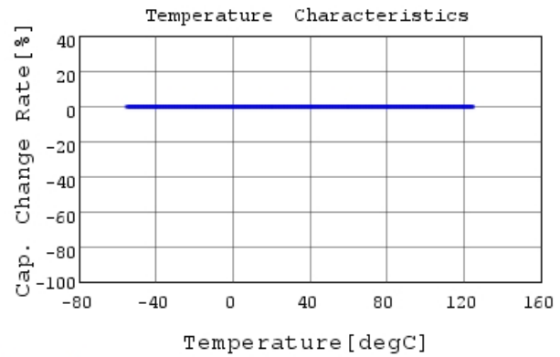
RCE5C2E100J1K1H03B C-Temp. capchange, DC0V,
