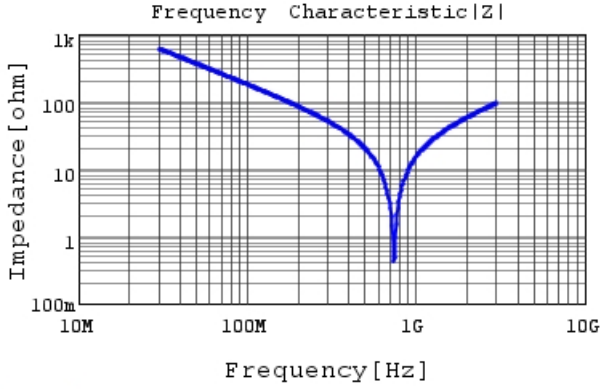
RCE5C2E100J1K1H03B |Z| DC0V, 25degC
