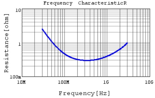
RCE5C2E100J1K1H03B R DC0V, 25degC
