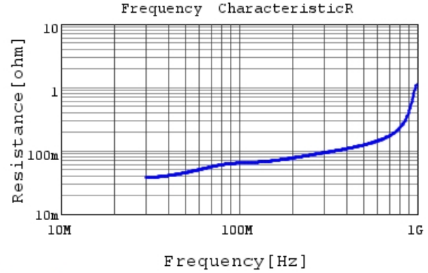
RCE5C2E271J1K1H03B R DC0V, 25degC
