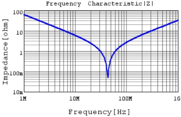
RCE5C2E272J1K1H03B |Z| DC0V, 25degC
