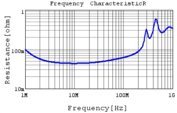
RCE5C2E272J1K1H03B R DC0V, 25degC
