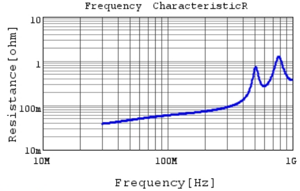
RCE5C2J821J1K1H03B R DC0V,25degC
