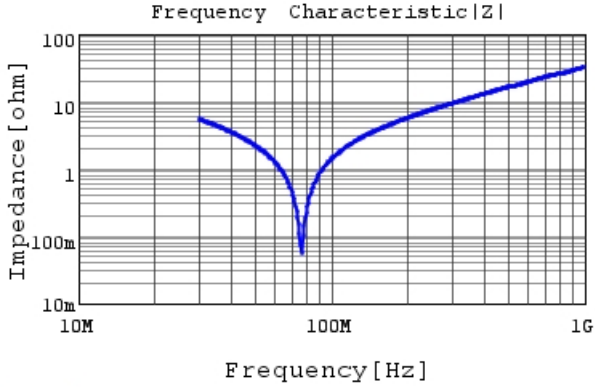
RCE5C2J821J1K1H03B |Z| DC0V,25degC
