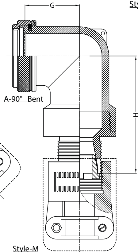
Style-M Clamp Medium Duty (Table-3)
