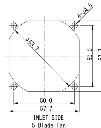
(Panel Out-line)
