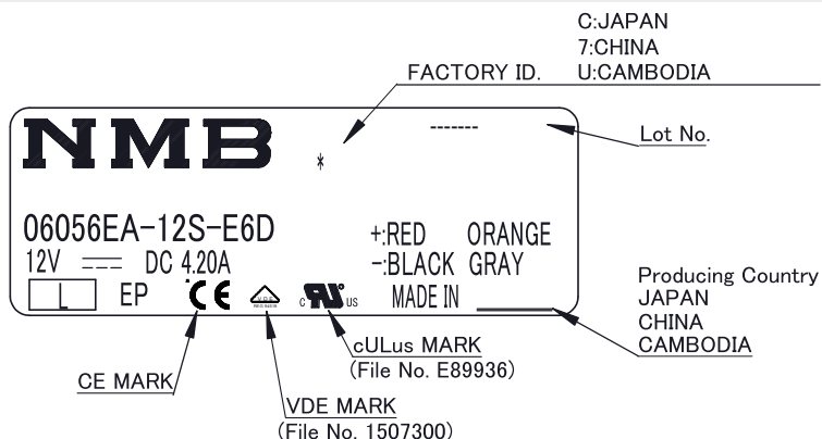
(Name Plate)
