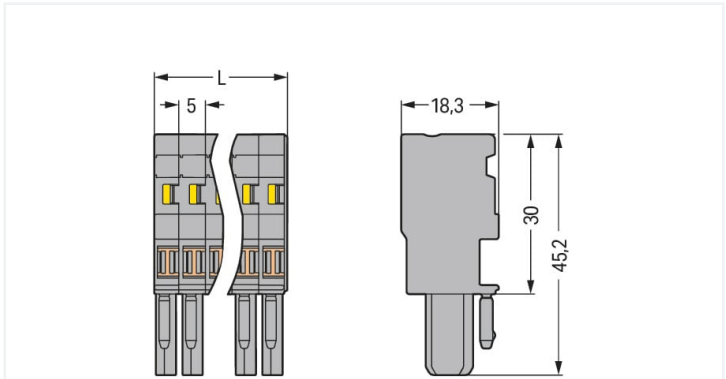
L = pole no. x module width
