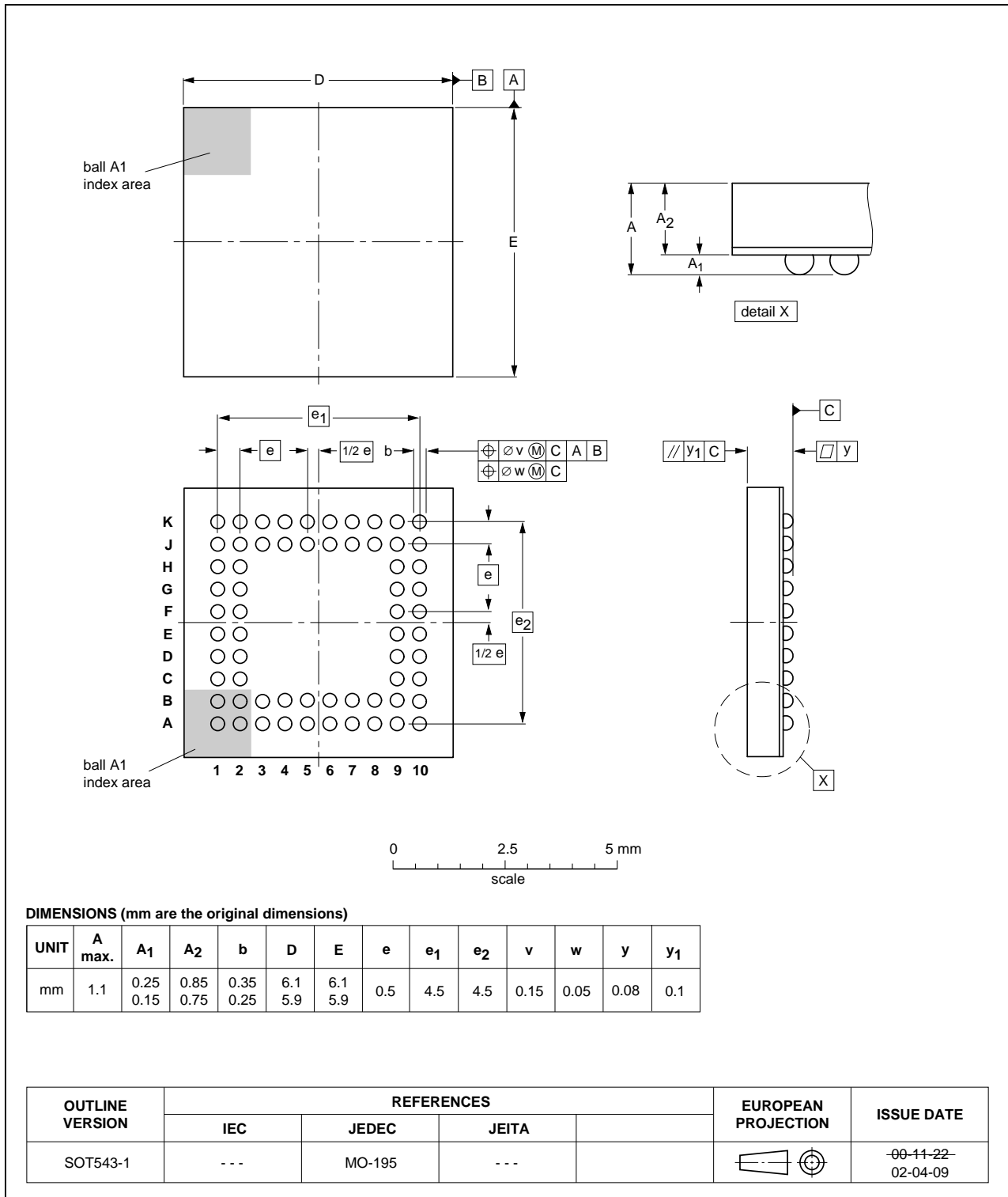
TFBGA64: plastic thin fine-pitch ball grid array package; 64 balls; body 6 x 6 x 0.8 mm
