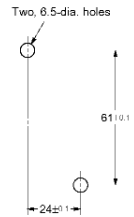
Mounting Hole Dimensions (TOP VIEW)
