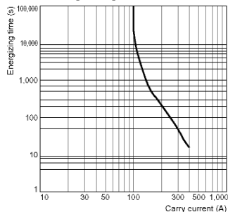
Carry Current vs Energizing Time
