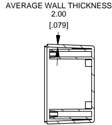
SECTION A-A SCALE 3 / 8
