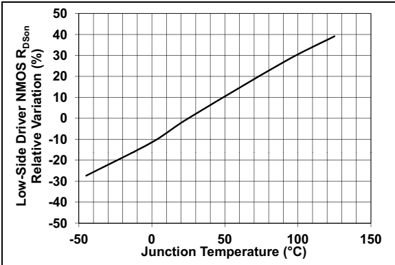
FIGURE 2-16: LDRV N-Ch R_{DS(on)} Relative Variation vs. Temperature
