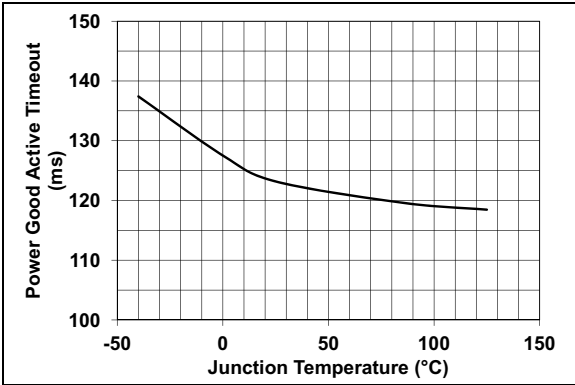
FIGURE 2-17: PG Active Time Out Period vs. Temperature.
