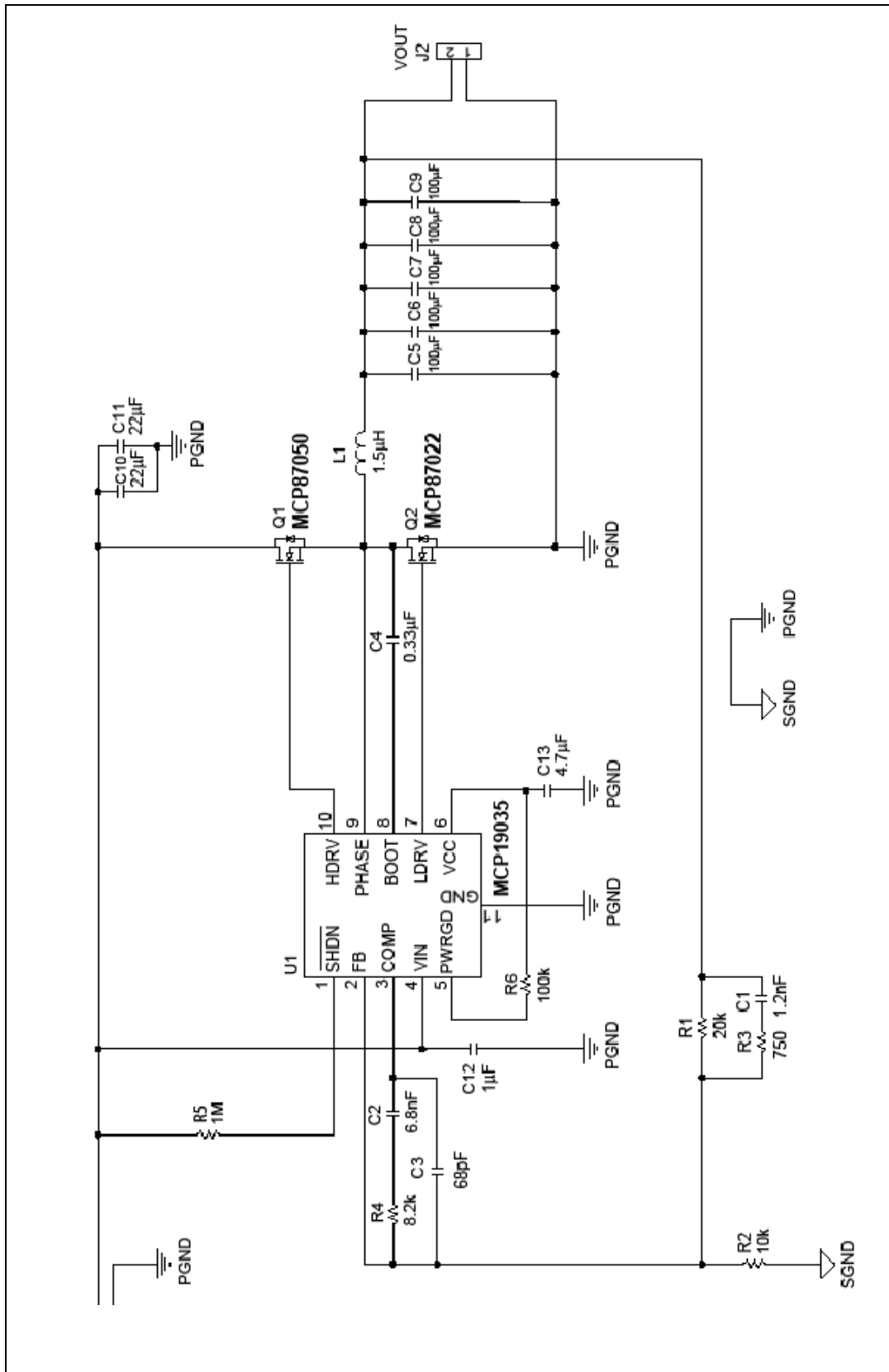
FIGURE 6-4: Schematic Diagram.
