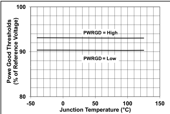
FIGURE 2-18: PG Thresholds Voltage vs. Temperature.
