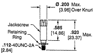
Jackscrew Assembly High Profile (H) 096-0002-0061 M83513/5-16 (HM) 096-0002-0088
