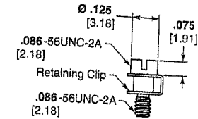
Lockscrew Assembly 096-0002-0008
