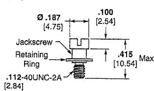
Jackscrew Assembly Low Profile (J) 096-0002-0062 M83513/5-15 (JM) 096-0002-0089
