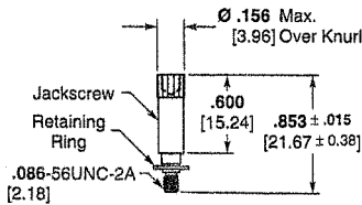
Jackscrew Assembly High Profile (Q) 096-0002-0014 M83513/5-03 (QM) 096-0002-0086
