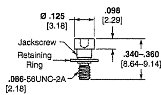
Jackscrew Assembly Low Profile (R) 096-0002-0015 M83513/5-02 (RM) 096-0002-0087
