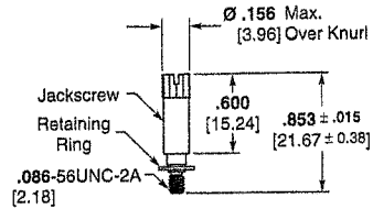
Jackscrew Assembly High Profile (K) 096-0002-0010 M83513/5-06 (KM) 096-0002-0084
