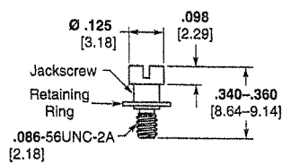
Jackscrew Assembly Low Profile (L) 096-0002-0011 M83513/5-05 (LM) 096-0002-0085
