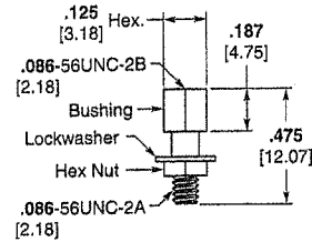
Jackpost Assembly (P) 096-0002-0009 M83513/5-07 P mates with K,KM, L,LM, Q,QM and R,RM Jackscrew Assemblies.
