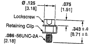
Lockscrew Assembly 096-0002-0013
