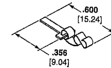
Mounting Key and Clip P/N 096-0001-0000 (2 Required)
