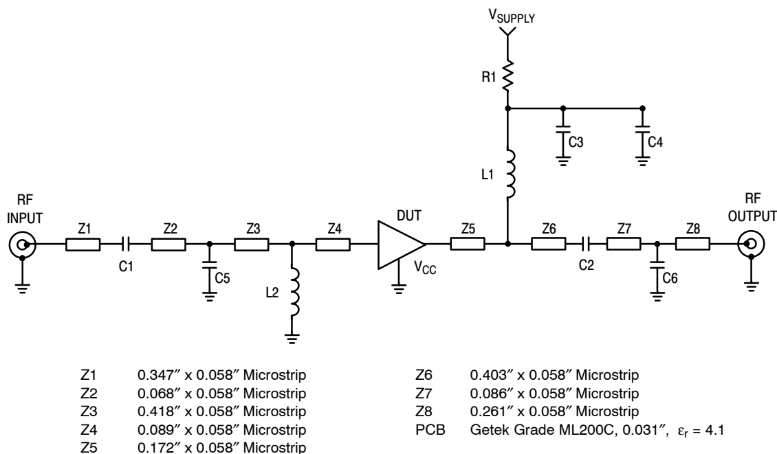
Figure 14. 50 Ohm Test Circuit Schematic
