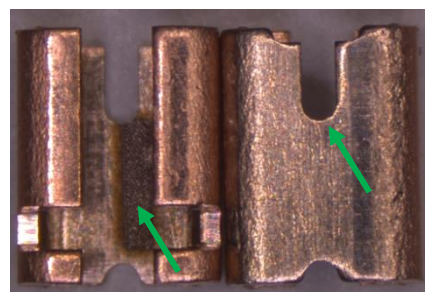
Figure 2 Laser Ablation
