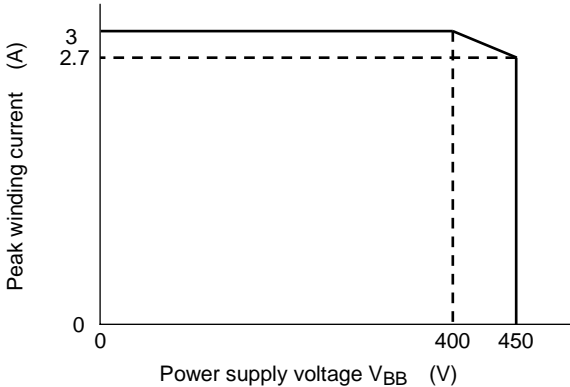
Figure 1 SOA at T_j = 135\text{ }^\circ\text{C}
