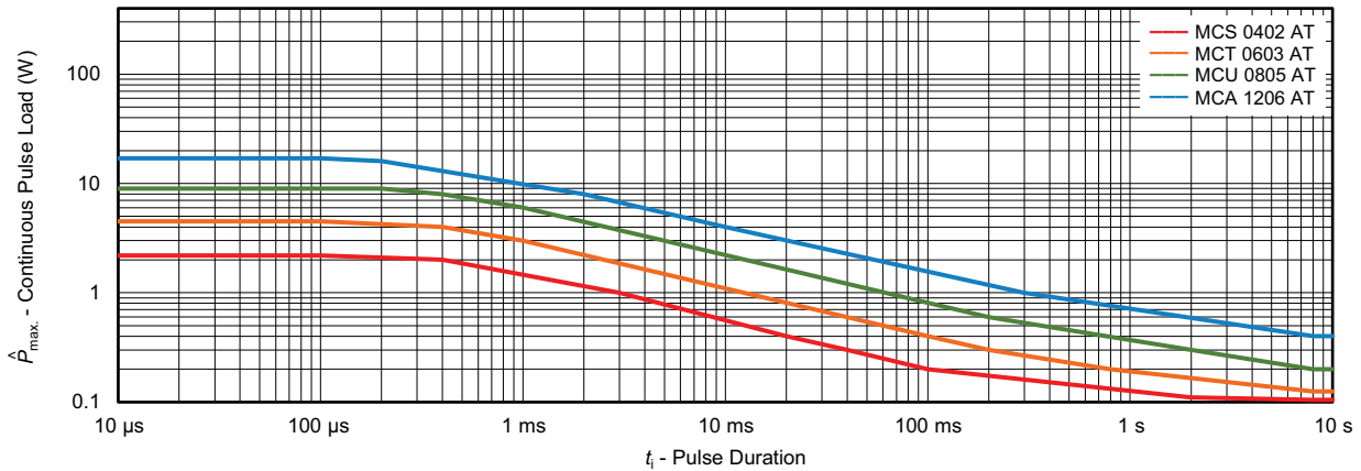
Maximum pulse load, continuous pulses; applicable if \bar{P} \leq P(\vartheta_{amb}) and \hat{U} \leq \hat{U}_{max} ; for permissible resistance change equivalent to 8000 h operation in standard operation mode
