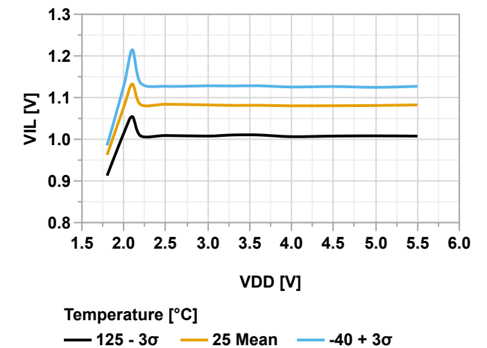
Figure 40-72. Input Pin SMBus - Maximum V_{IL} vs. V_{DD}
