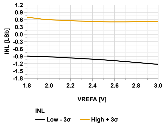
Figure 40-113. INL vs. V_{\text{REFA}} (ADC Single Ended Mode @60 kpsps, V_{\text{DD}} = 3.0\text{V} , T = 125^\circ\text{C} )
