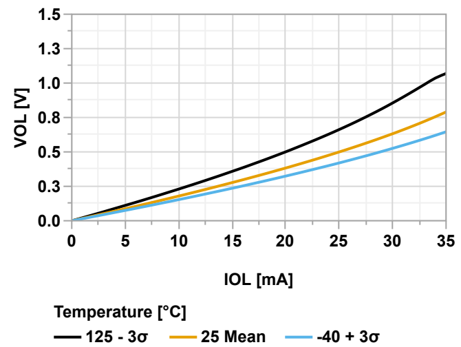
Figure 40-79. Output Pin - Maximum V_{OL} vs. Current, V_{DD} = 3.0V
