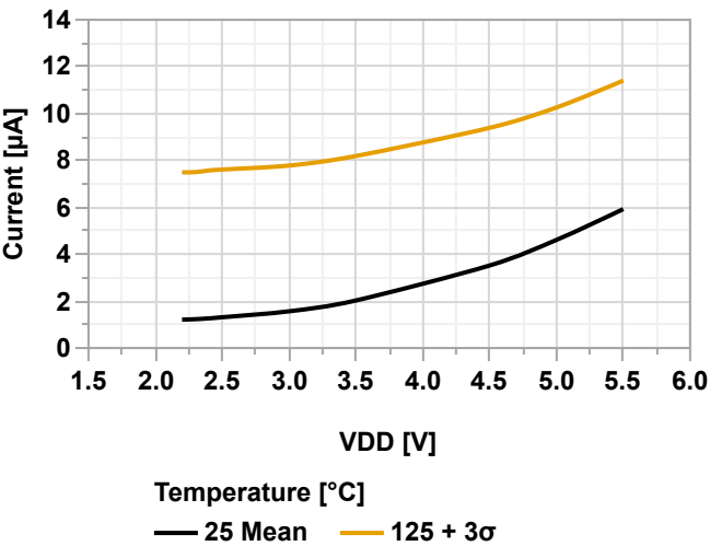
Figure 40-25. BOD Power Consumption vs. V_{DD} (BOD Sampling Mode @128 Hz)
