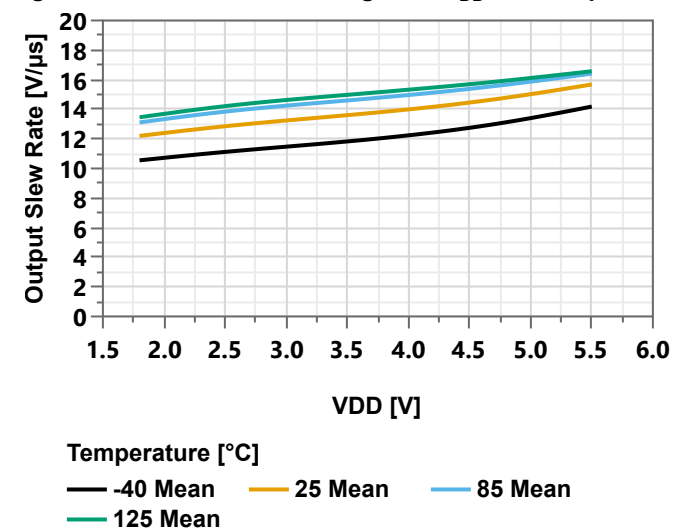
Figure 40-166. Slew Rate Falling Over V DD and Temperature
