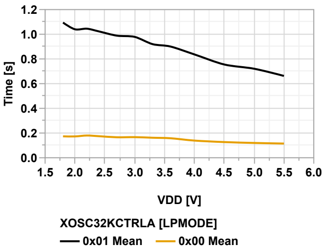
Figure 40-42. Typical XOSC32K Start-up Time vs. V_{DD} ( T = 25^{\circ}\text{C} )
