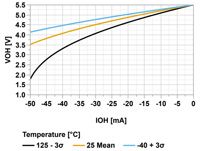
Figure 40-82. Output Pin - Minimum V_{OH} vs. Current, V_{DD} = 5.5V
