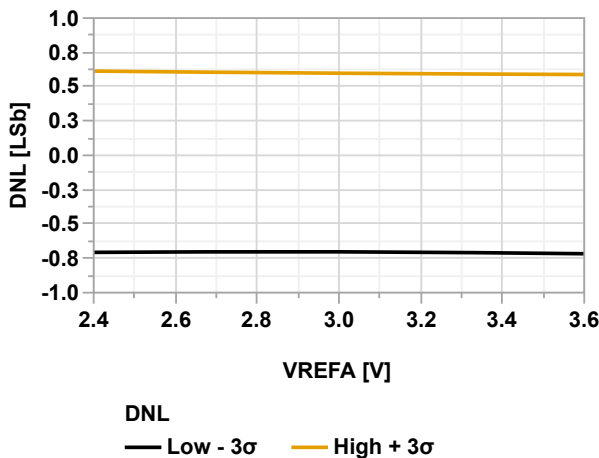
Figure 40-124. DNL vs. V_{\text{REFA}} (ADC Differential Mode @60 kps, V_{\text{DD}} = 3.6\text{V} , T = 125^\circ\text{C} )
