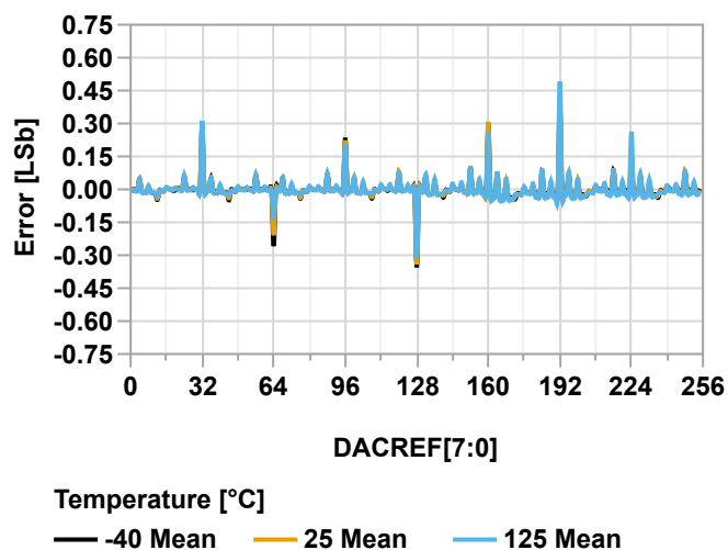
Figure 40-154. DNL vs. DAC Code ( V_{\text{REFA}} = V_{\text{DD}} = 3.0\text{V} )
