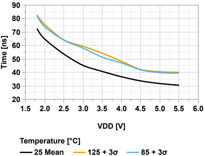
Figure 40-66. Rise Time vs. V_{DD} (PORTCTRL.SRL = 0x01)
