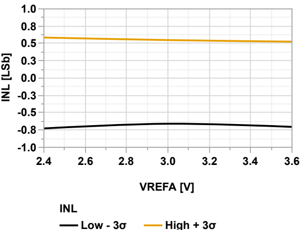
Figure 40-128. INL vs. V_{\text{REFA}} (ADC Differential Mode) @60 ksp/s, V_{\text{DD}} = 3.6\text{V} , T = 125^\circ\text{C}
