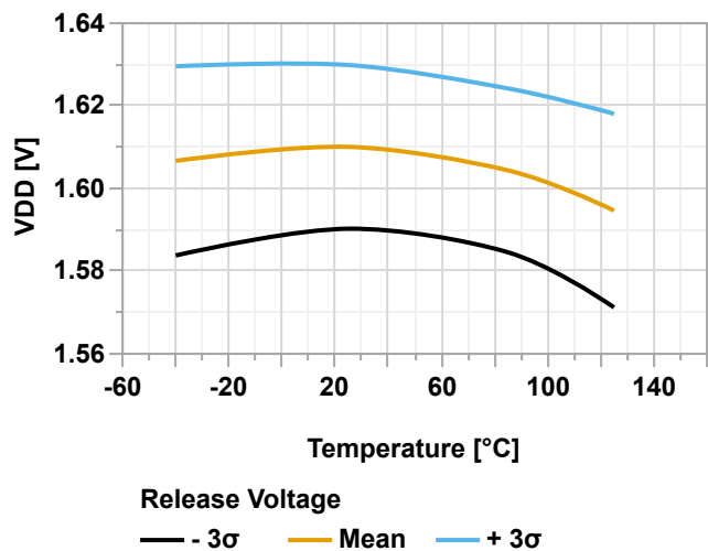
Figure 40-48. POR Release Voltage vs. Temperature
