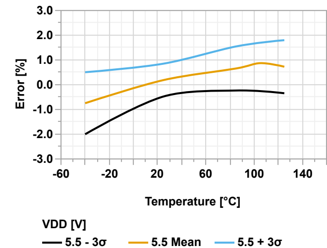
Figure 40-86. ADC0REF Voltage Error vs. Temperature ( V_{DD} = 5.5V , V_{VREF} = 2.048V )
