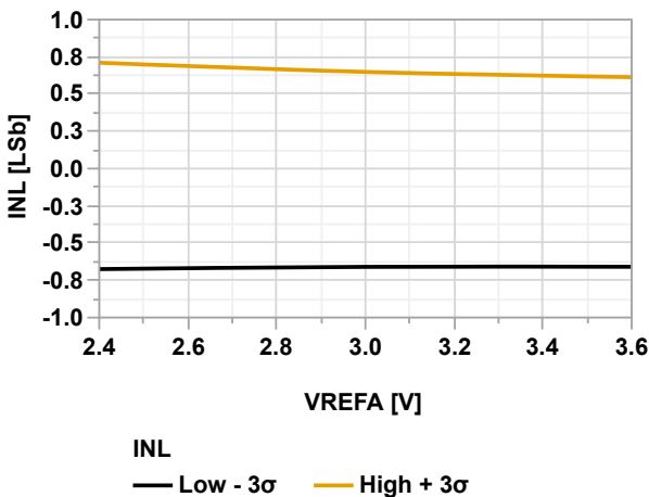
Figure 40-127. INL vs. V_{\text{REFA}} (ADC Differential Mode) @60 ksp/s, V_{\text{DD}} = 3.6\text{V} , T = 85^\circ\text{C}
