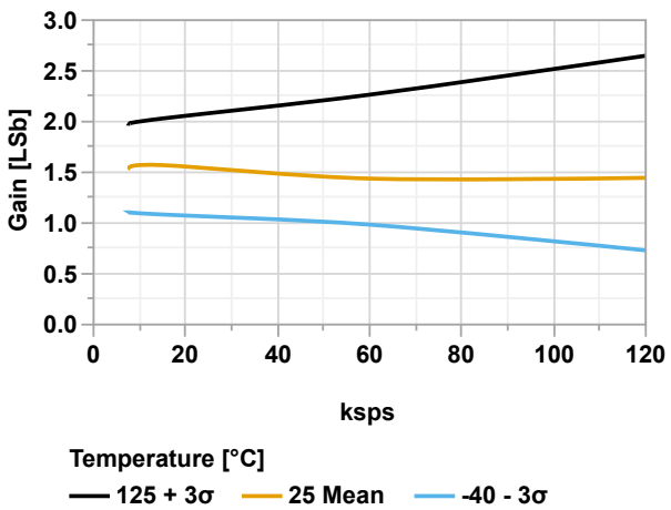
Figure 40-116. Positive Gain Error vs. Sample Rate (ADC Differential Mode, V_{\text{REFA}} = V_{\text{DD}} = 3.6\text{V} )
