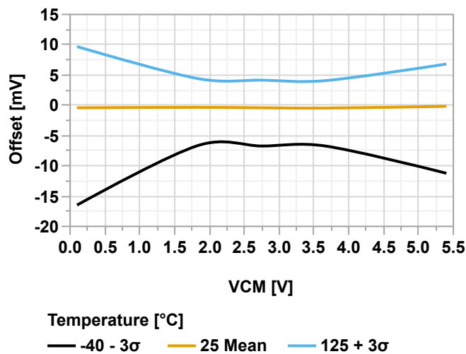
Figure 40-140. Input Offset vs. Common Mode Voltage ( V_{DD} = 5.5V )
