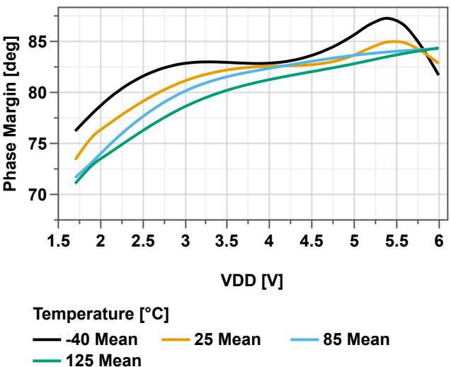
Figure 40-160. Phase Margin Over V_{DD} and Temperature
