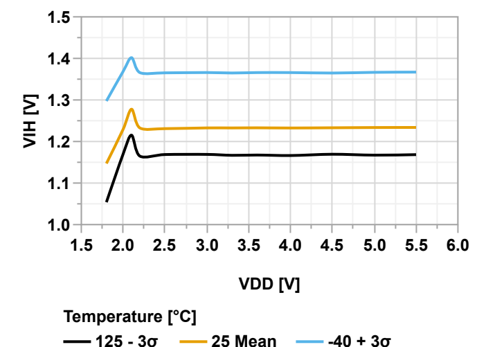
Figure 40-73. Input Pin SMBus - Minimum V_{IH} vs. V_{DD}
