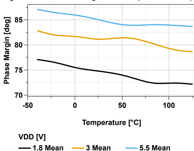
Figure 40-159. Phase Margin Over Temperature and V_{\text{DD}}
