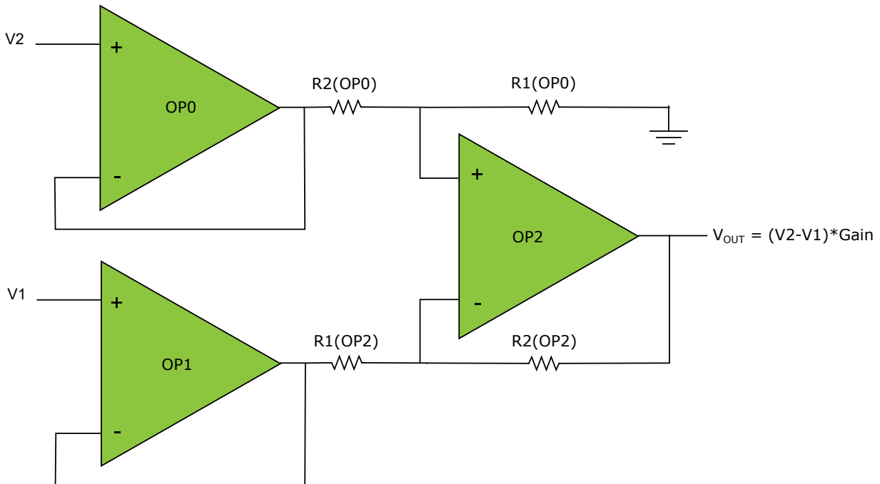
Figure 35-12. Instrumentation Amplifier
