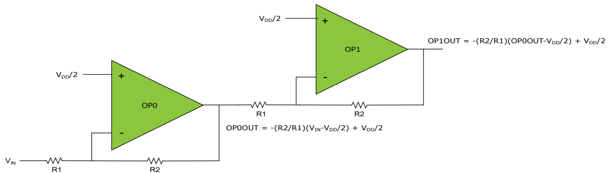
Figure 35-9. Cascaded (Two) Inverting PGA
