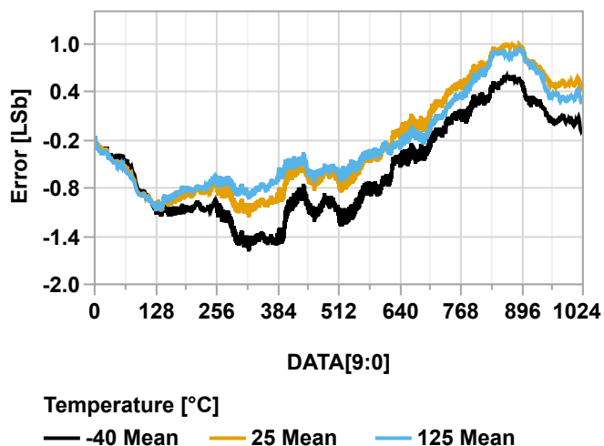
Figure 40-149. INL vs. DAC Code ( V_{\text{REFA}} = V_{\text{DD}} = 5.5\text{V} )
