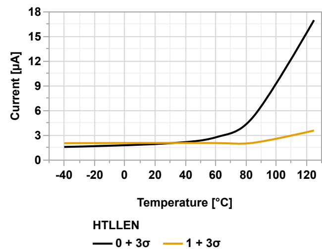
Figure 40-17. Typical +3σ Power-Down Power Consumption vs. Temperature (V DD = 5.5V)
