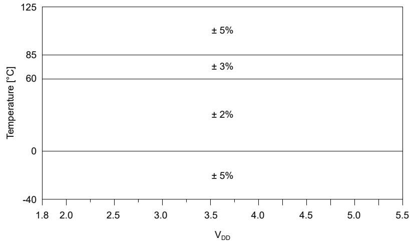
Figure 39-2. Precision Calibrated OSCHF ( f_{\text{OSCHF}} \geq 4 MHz) Frequency Accuracy Over Device V_{\text{DD}} and Temperature (1)
