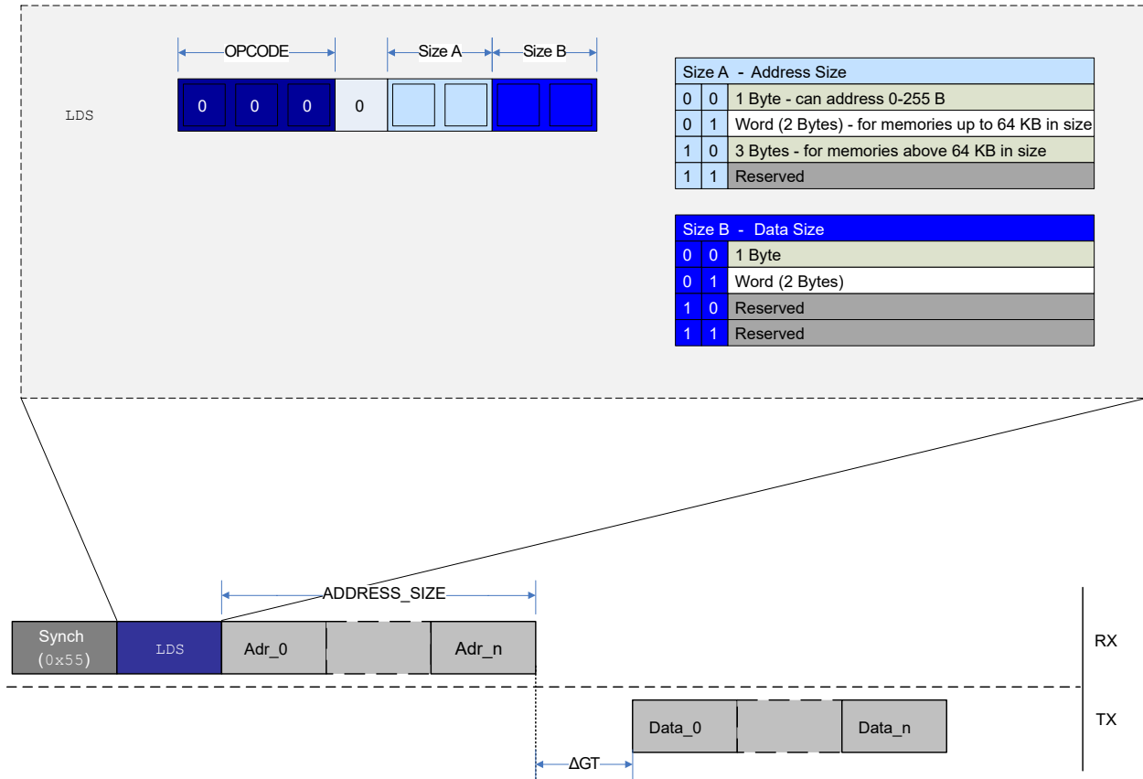
Figure 37-8. LDS Instruction Operation
