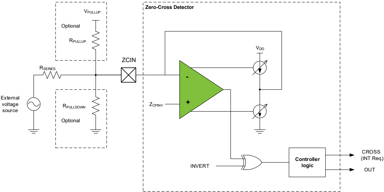
Figure 36-1. Zero-Cross Detector
