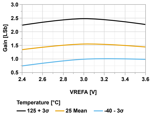
Figure 40-115. Positive Gain Error vs. V_{\text{REFA}} (ADC Differential Mode @60 kpsps, V_{\text{DD}} = 3.6\text{V} )
