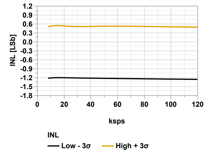
Figure 40-114. INL vs. Sample Rate (ADC Single Ended Mode, V_{\text{REFA}} = V_{\text{DD}} = 3.0\text{V} , T = 125^\circ\text{C} )
