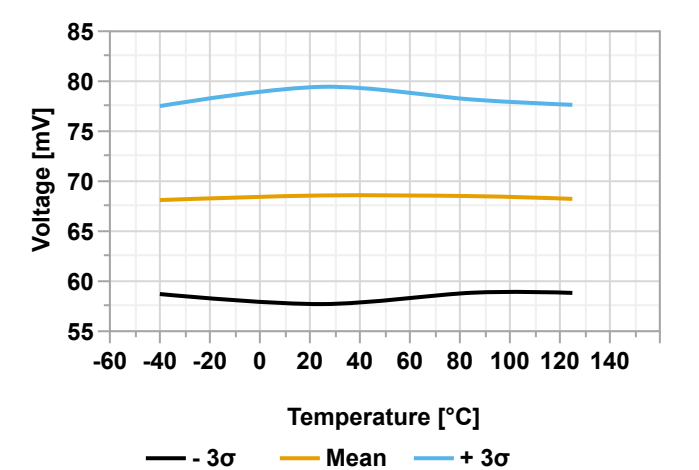
Figure 40-59. BOD Hysteresis vs. Temperature (BODCFG.LVL = 0x03)
