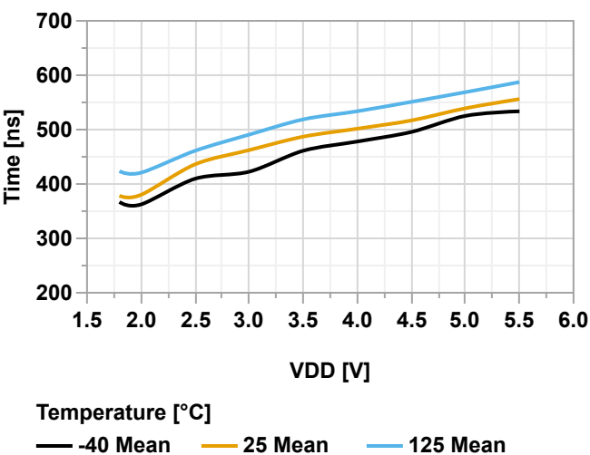
Figure 40-192. Rising Edge Response Time vs. V_{DD}
