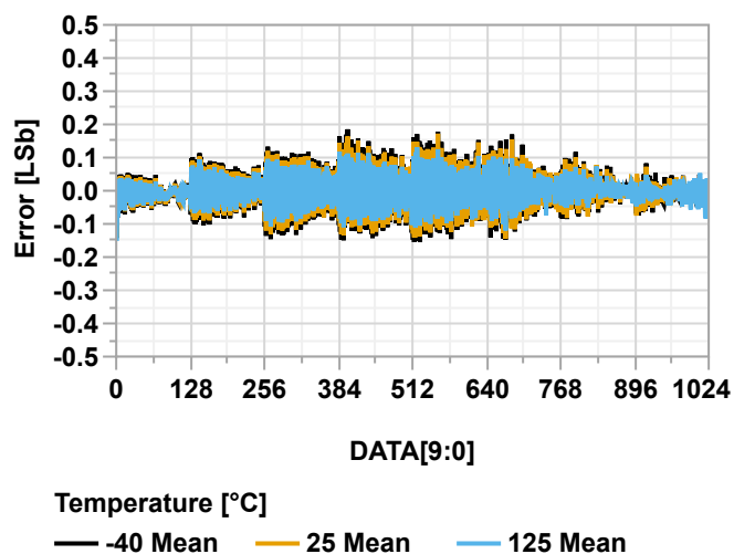
Figure 40-146. DNL vs. DAC Code ( V_{\text{REFA}} = V_{\text{DD}} = 3.0\text{V} )
