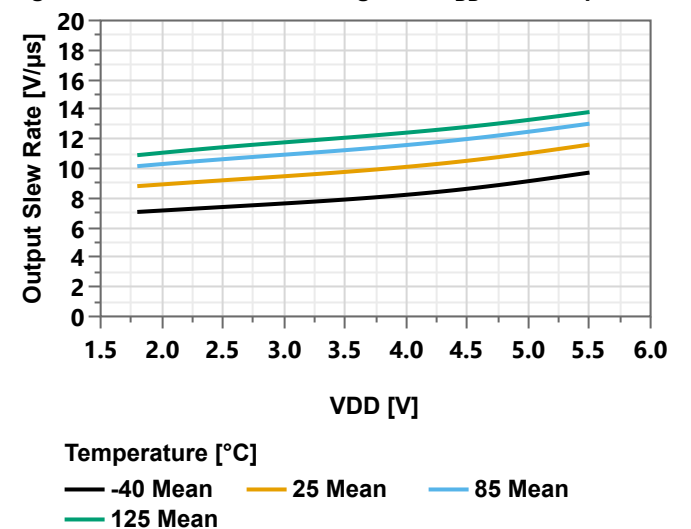
Figure 40-167. Slew Rate Rising Over V DD and Temperature
