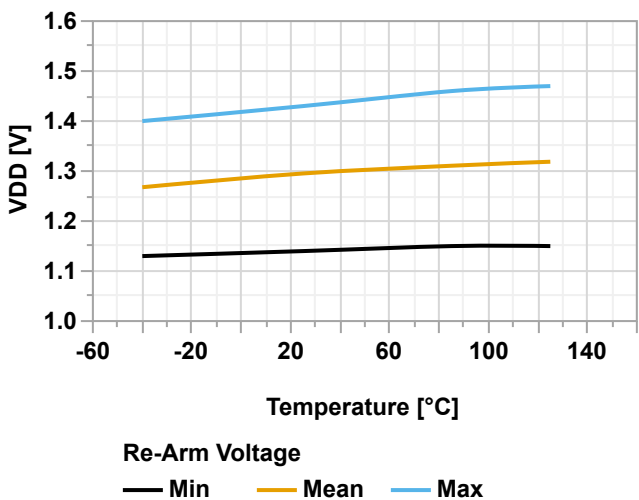
Figure 40-49. POR Re-Arm Voltage vs. Temperature
