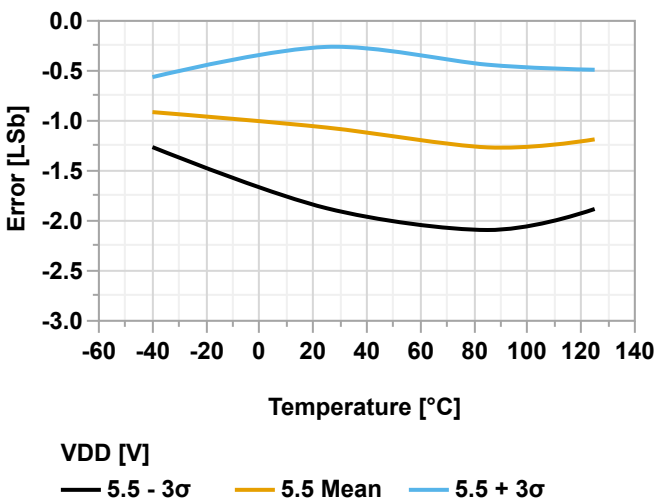
Figure 40-143. Gain Error vs. Temperature ( V_{REFA} = V_{DD} = 5.5V )
