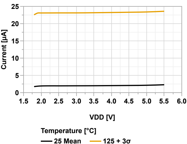
Figure 40-13. Standby Power Consumption vs. V_{DD} (RTC.CLKSEL = XOSC32K, XOSC32KCTRLA.LPMODE = 1)
