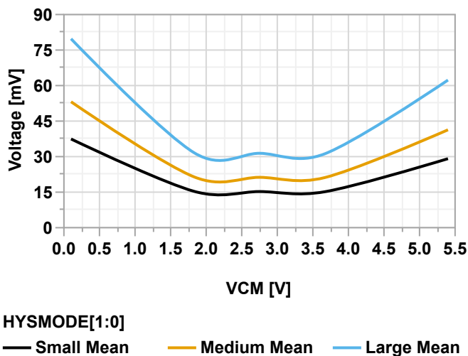
Figure 40-141. Input Hysteresis vs. Common Mode Voltage ( V_{DD} = 5.5V )
