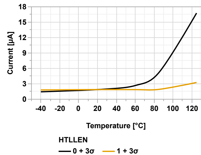
Figure 40-16. Typical +3σ Power-Down Power Consumption vs. Temperature (V DD = 3.0V)
