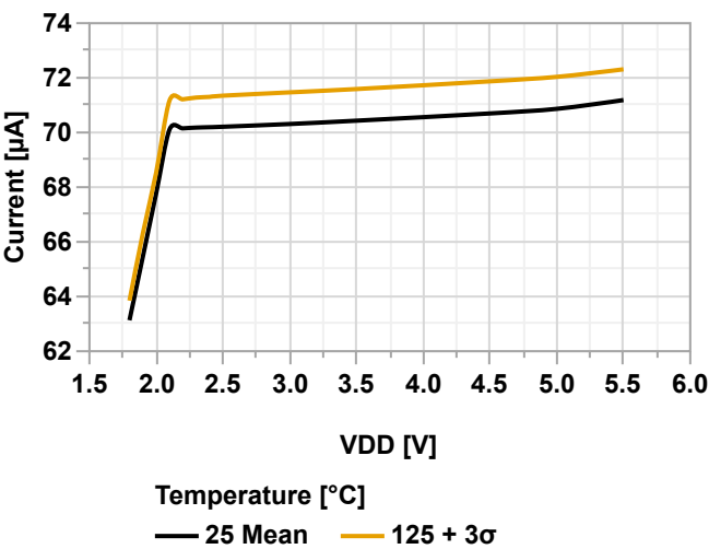
Figure 40-39. VREF Power Consumption vs. V_{DD} (ACREF Enabled)
