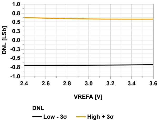
Figure 40-123. DNL vs. V_{\text{REFA}} (ADC Differential Mode @60 kps, V_{\text{DD}} = 3.6\text{V} , T = 85^\circ\text{C} )
