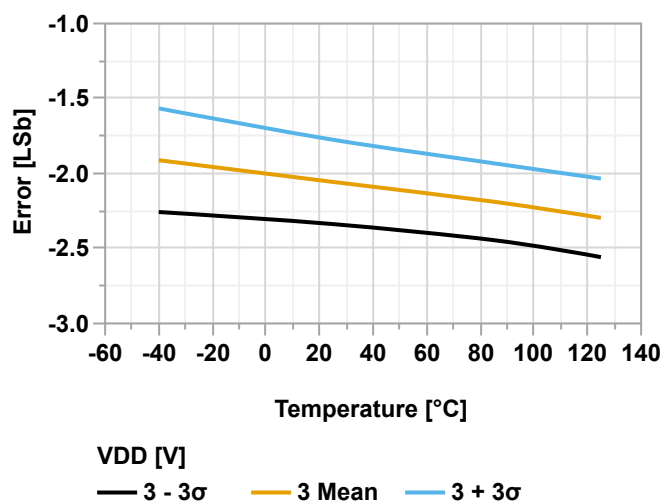
Figure 40-150. Gain Error vs. Temperature ( V_{\text{REFA}} = V_{\text{DD}} = 3.0\text{V} )
