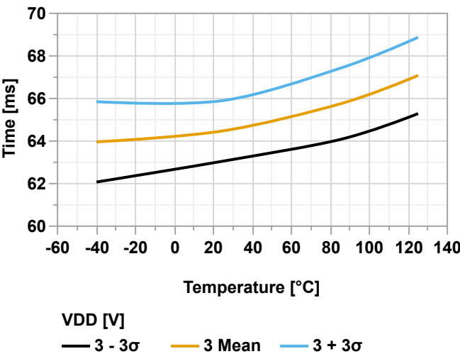
Figure 40-46. Start-up Time vs. Temperature (SYSCFG1 = 0x07, V_{DD} = 3.0V)
