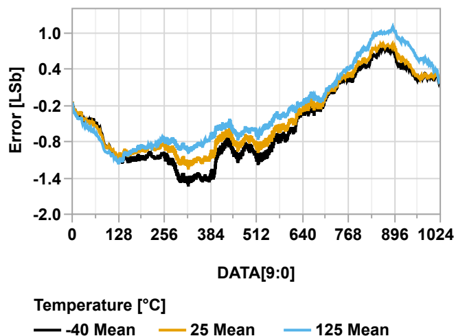
Figure 40-148. INL vs. DAC Code ( V_{\text{REFA}} = V_{\text{DD}} = 3.0\text{V} )
