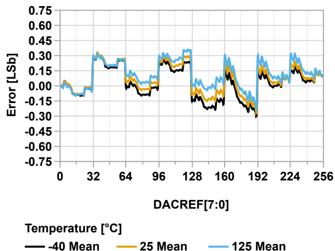
Figure 40-156. INL vs. DAC Code ( V_{\text{REFA}} = V_{\text{DD}} = 3.0\text{V} )
