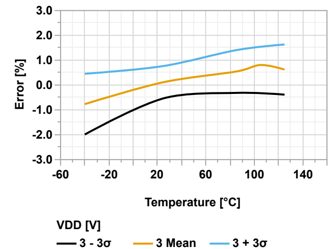
Figure 40-87. ADC0REF Voltage Error vs. Temperature ( V_{DD} = 3.0V , V_{VREF} = 2.048V )
