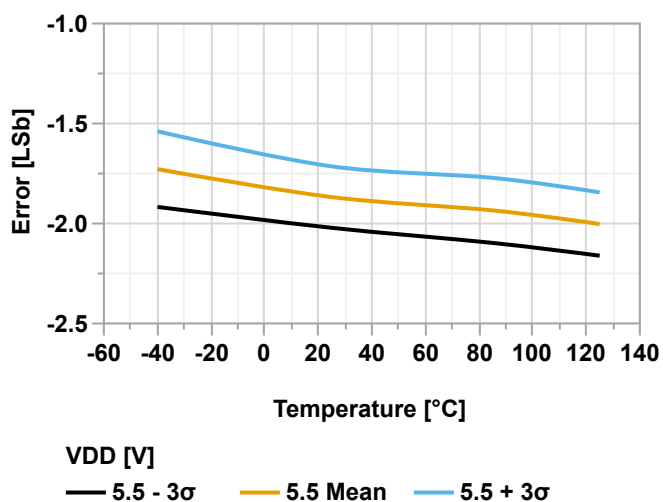
Figure 40-151. Gain Error vs. Temperature ( V_{\text{REFA}} = V_{\text{DD}} = 5.5\text{V} )
