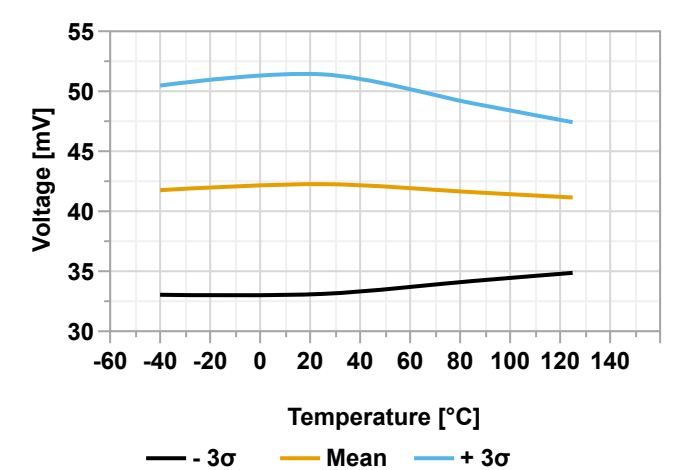
Figure 40-58. BOD Hysteresis vs. Temperature (BODCFG.LVL = 0x02)
