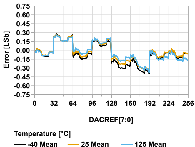
Figure 40-157. INL vs. DAC Code ( V_{\text{REFA}} = V_{\text{DD}} = 5.5\text{V} )
