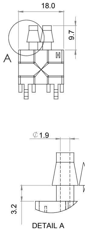
Dimensional drawing ZA009102 plug-in adapter
