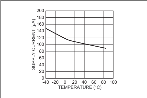
FIGURE 2-10: On-State Supply Current vs. Temperature.
