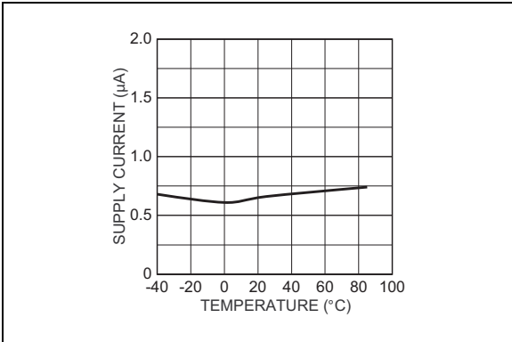
FIGURE 2-11: Off-State Supply Current vs. Temperature.
