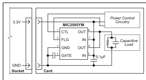
FIGURE 6-3: Hot Plug-In Concept.
