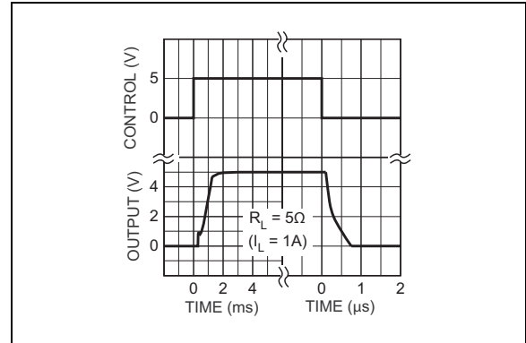
FIGURE 2-4: MIC2506 Turn-On, Turn-Off Characteristics.
