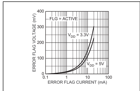
FIGURE 2-6: Error Flag Voltage vs. Error Flag Current.
