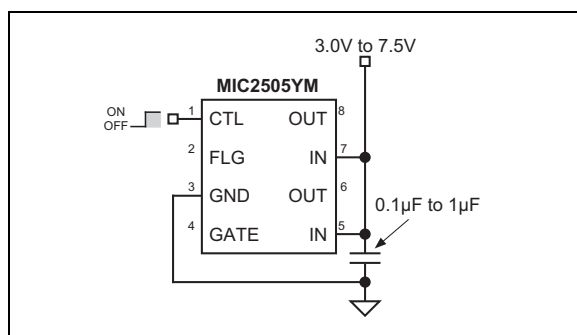
FIGURE 6-1: Supply Bypassing.
