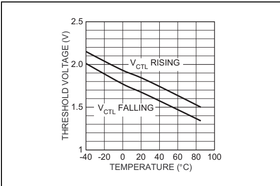
FIGURE 2-12: Control Threshold vs. Temperature.
